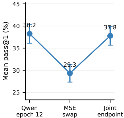
GSM8K / ELF-B
