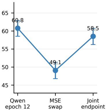
GSM8K / ELF-L
