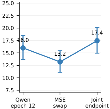
MATH500 / ELF-L
