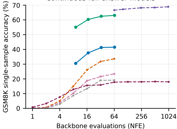
Continuous full-answer models
