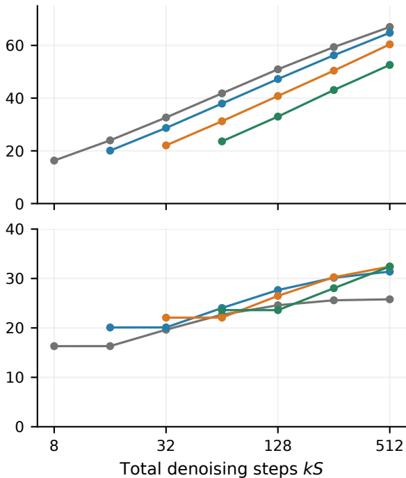
MATH500 · ELF-L
