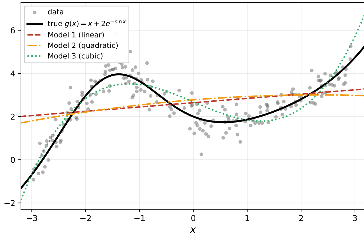
Polynomial OLS: cannot capture oscillation
