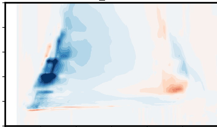
GFDL_B - GFDL
