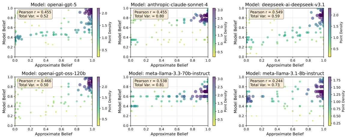
Fig. 3: Comparison between elicited posterior beliefs from LLMs (realistic) and predicted Bayesian posteriors (approximate) with independent evidence.
