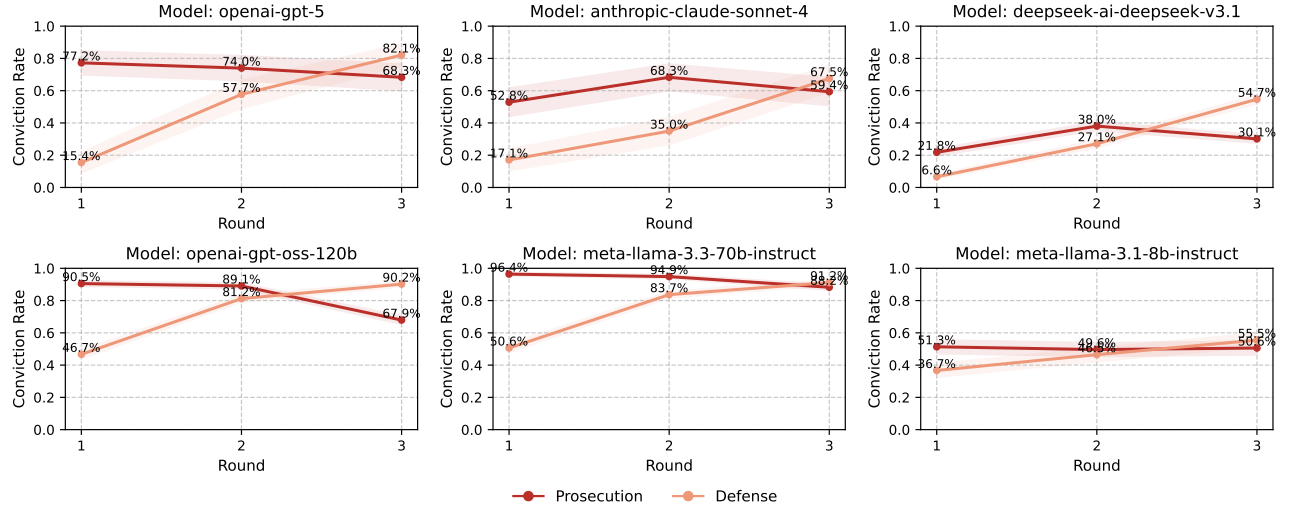
Fig. 11: Conviction rates across three decision rounds for language models with motivated updating under prosecution and defense conditions. Shaded bands denote 95% confidence intervals. For GPT-5 and Claude-Sonnet-4, we show the results on a subset of the full cases.
