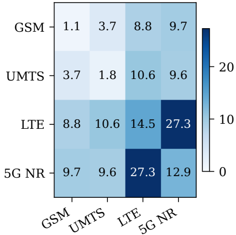
(c) 2-Source Pairs (%)
