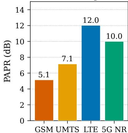
(a) PAPR Comparison
