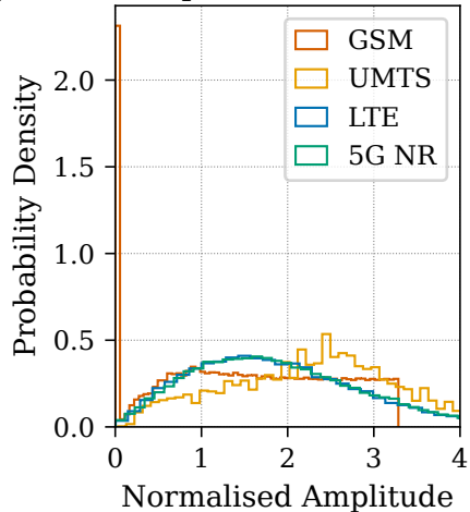
(c) Amplitude Distribution
