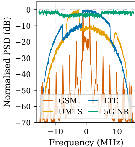
(b) Power Spectral Density
