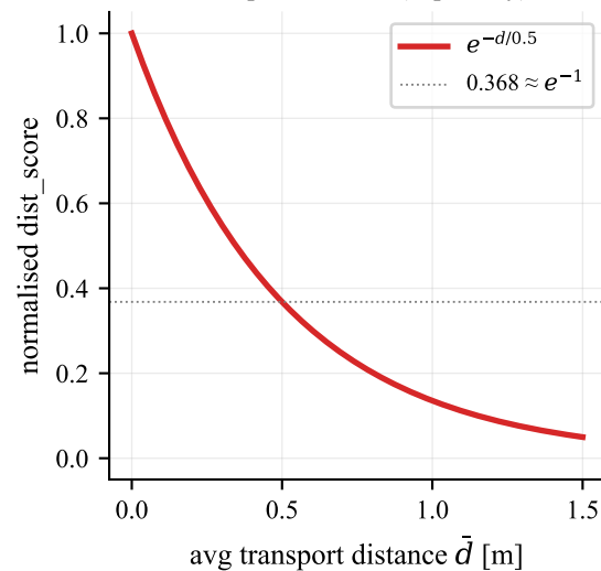
Transport distance (exp decay)
