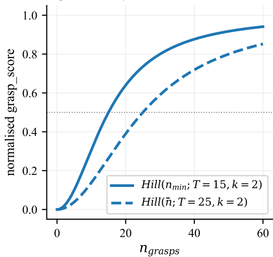
Grasp redundancy (Hill function, soft saturation)
