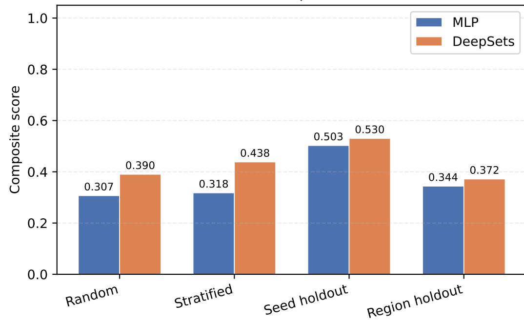
(a) Composite
