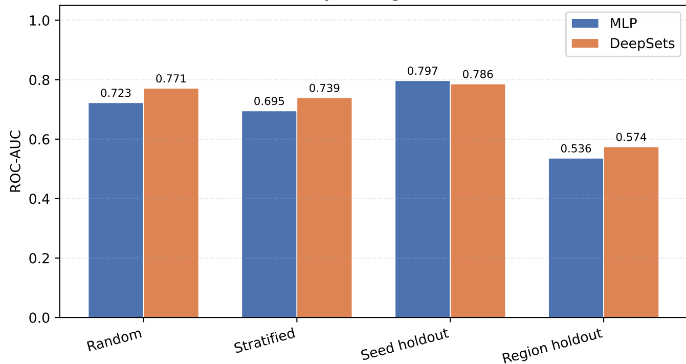
Feasibility ranking (ROC-AUC)
