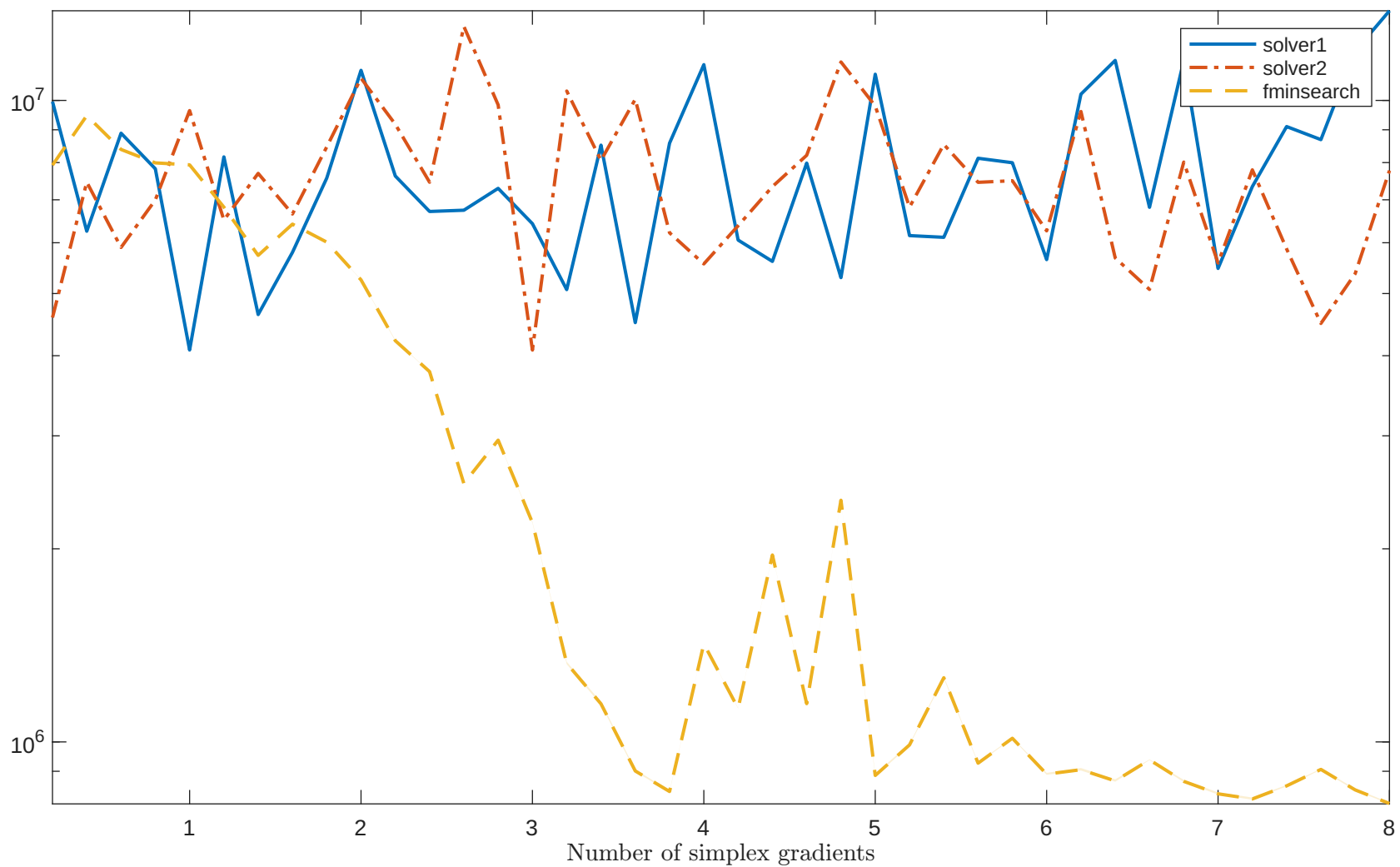
Solving "BROWNDEN" with "noisy_0.001-mixed-gaussian" feature
