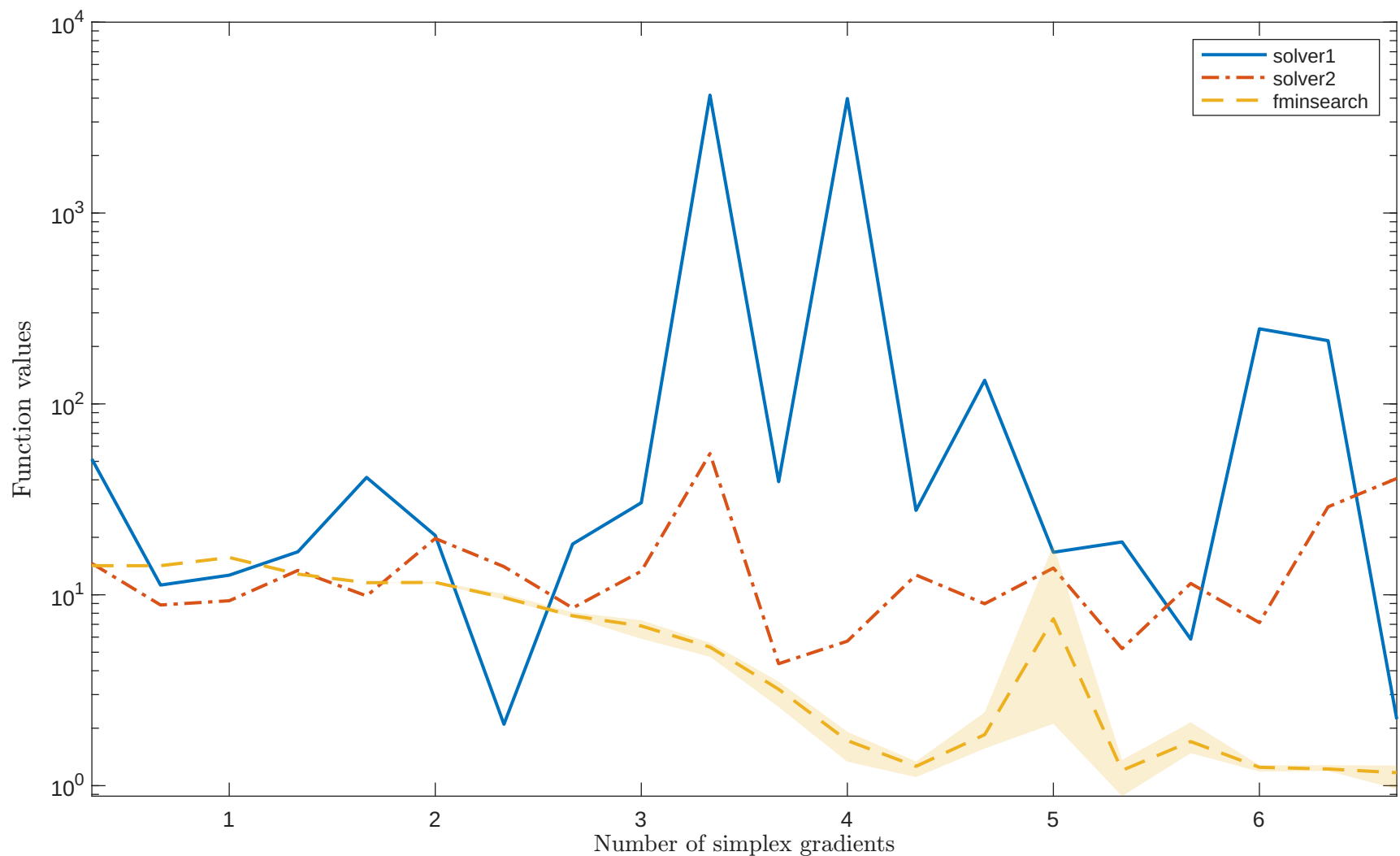
Solving “BEALE” with “noisy_0.001_mixed_gaussian” feature
