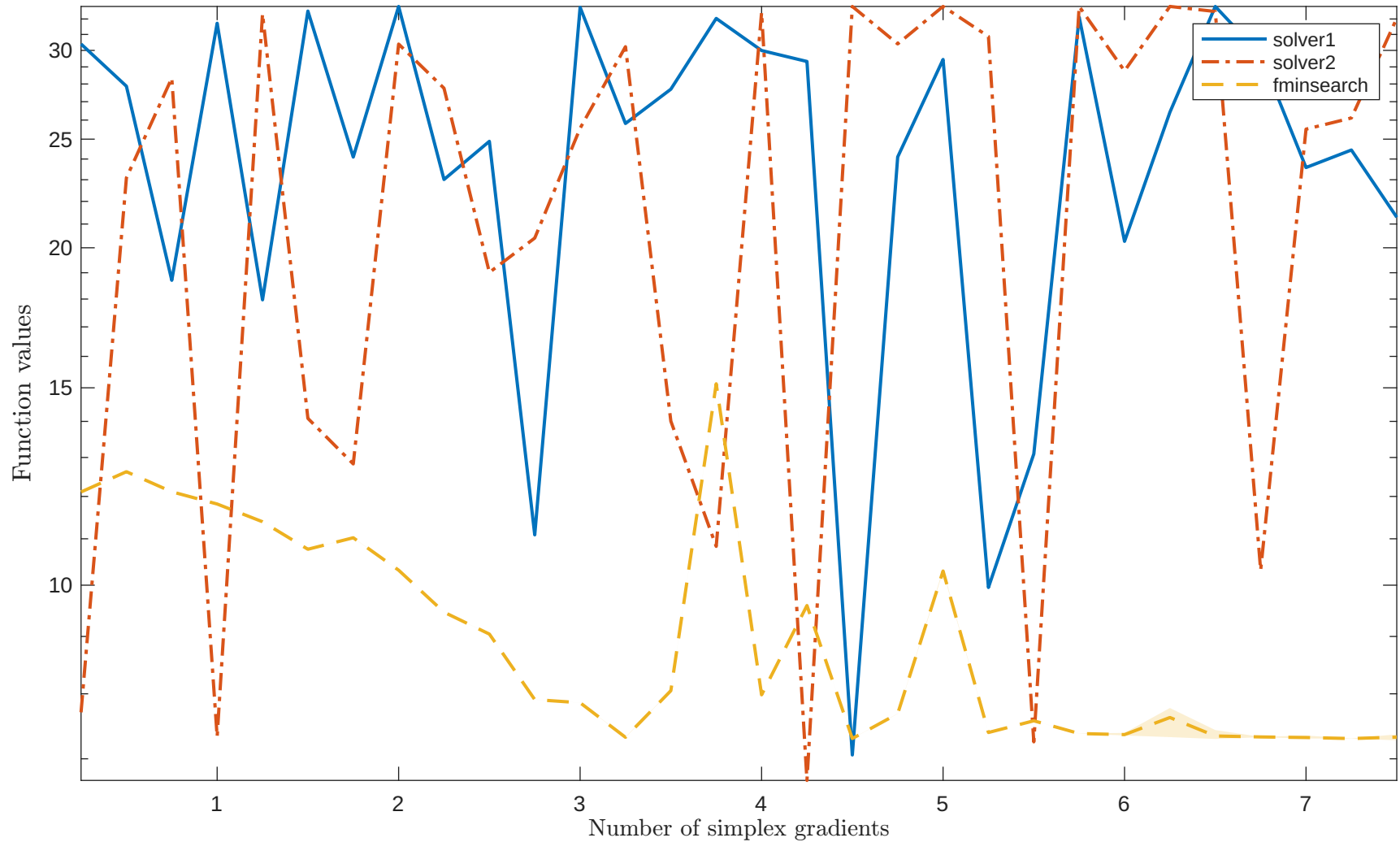
Solving "GULF" with "noisy_0.001_mixed_gaussian" feature
