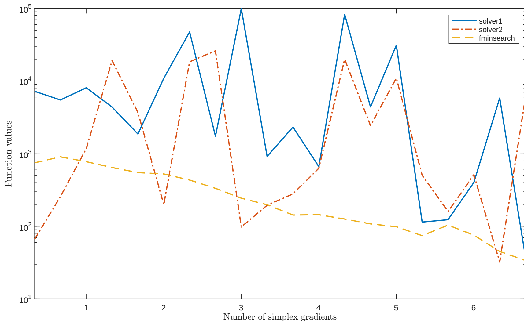
Solving “CUBE” with “noisy_0.001_mixed_gaussian” feature
