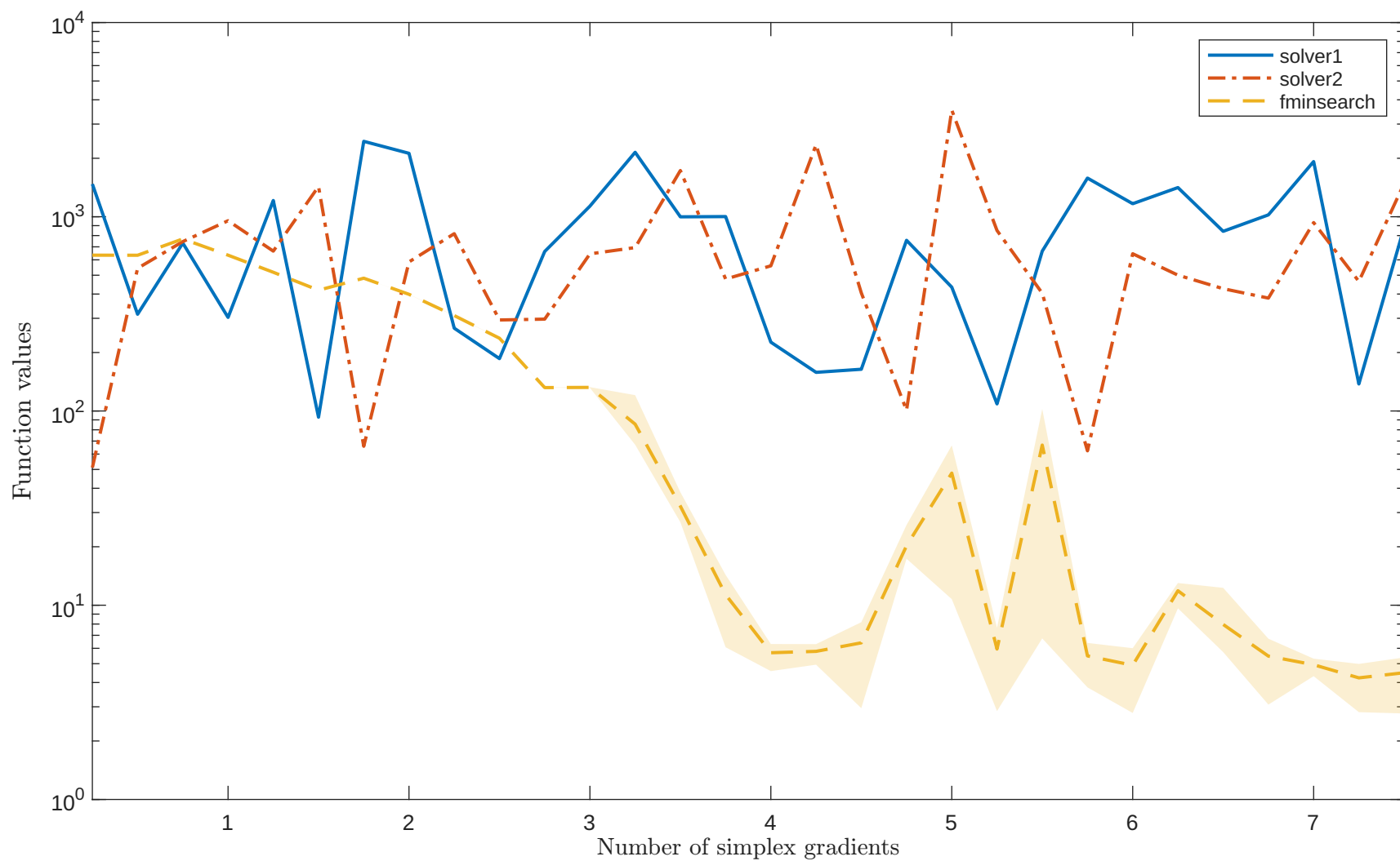
Solving “RECIPELS” with “noisy_0.001_mixed_gaussian” feature
