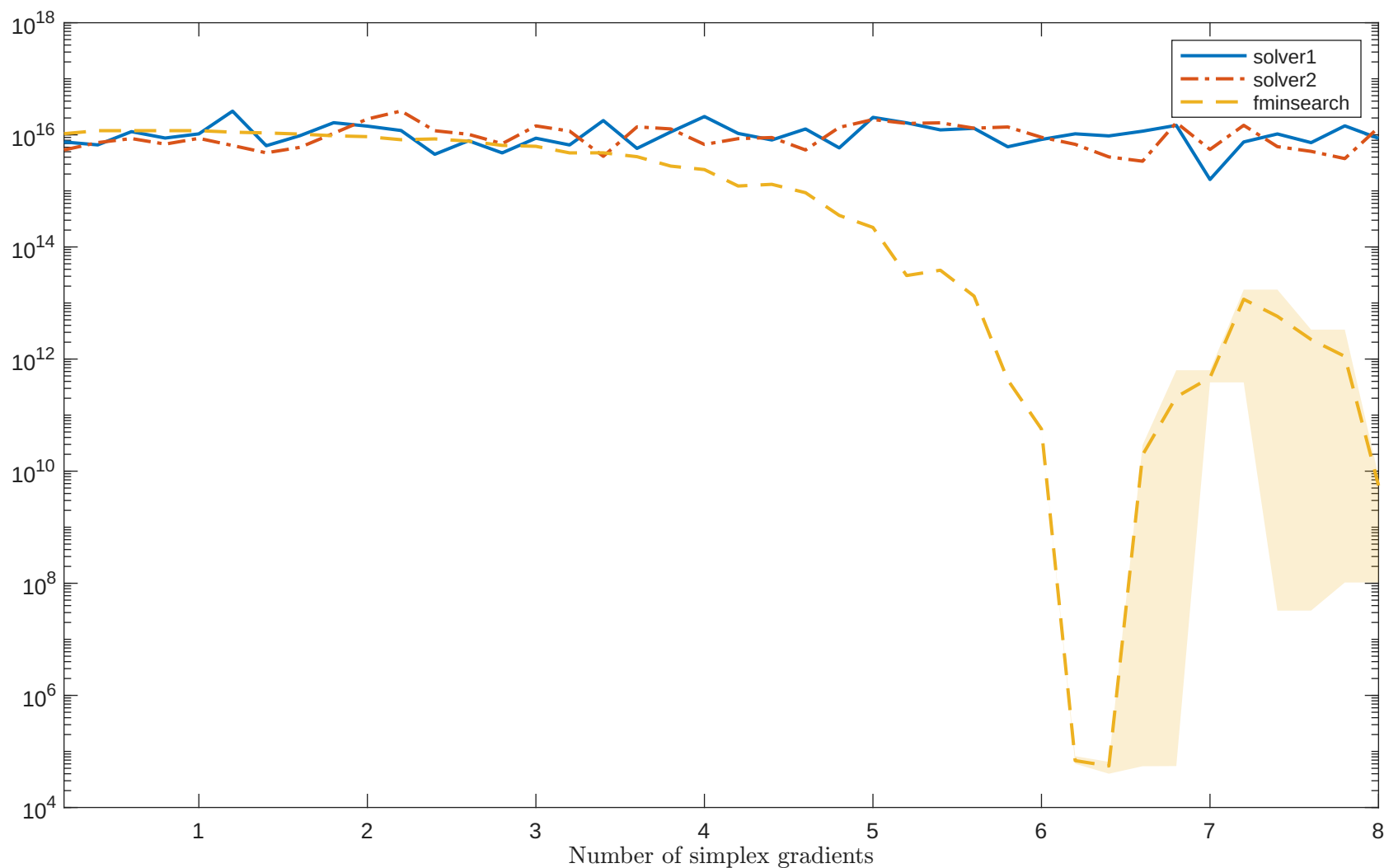
Solving “n10FOLDTRLs” with “noisy_0.001_mixed_gaussian” feature
