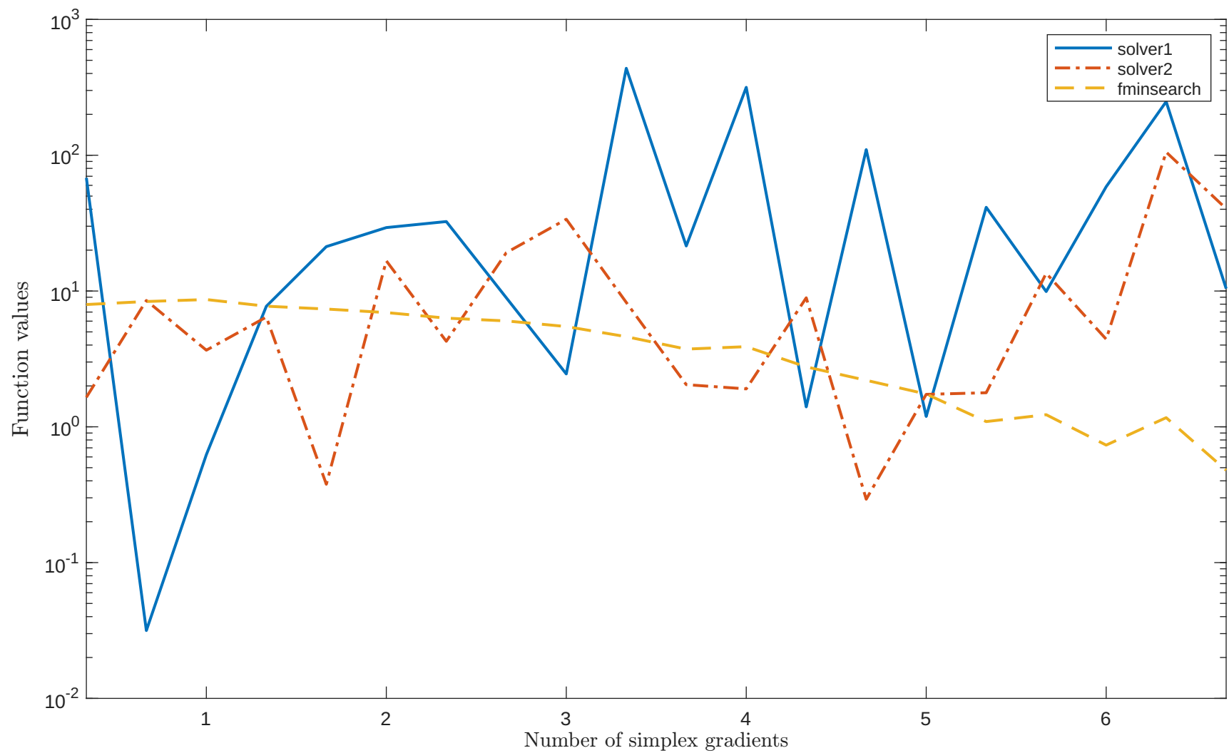
Solving “DENSCHNA” with “noisy_0.001_mixed_gaussian” feature
