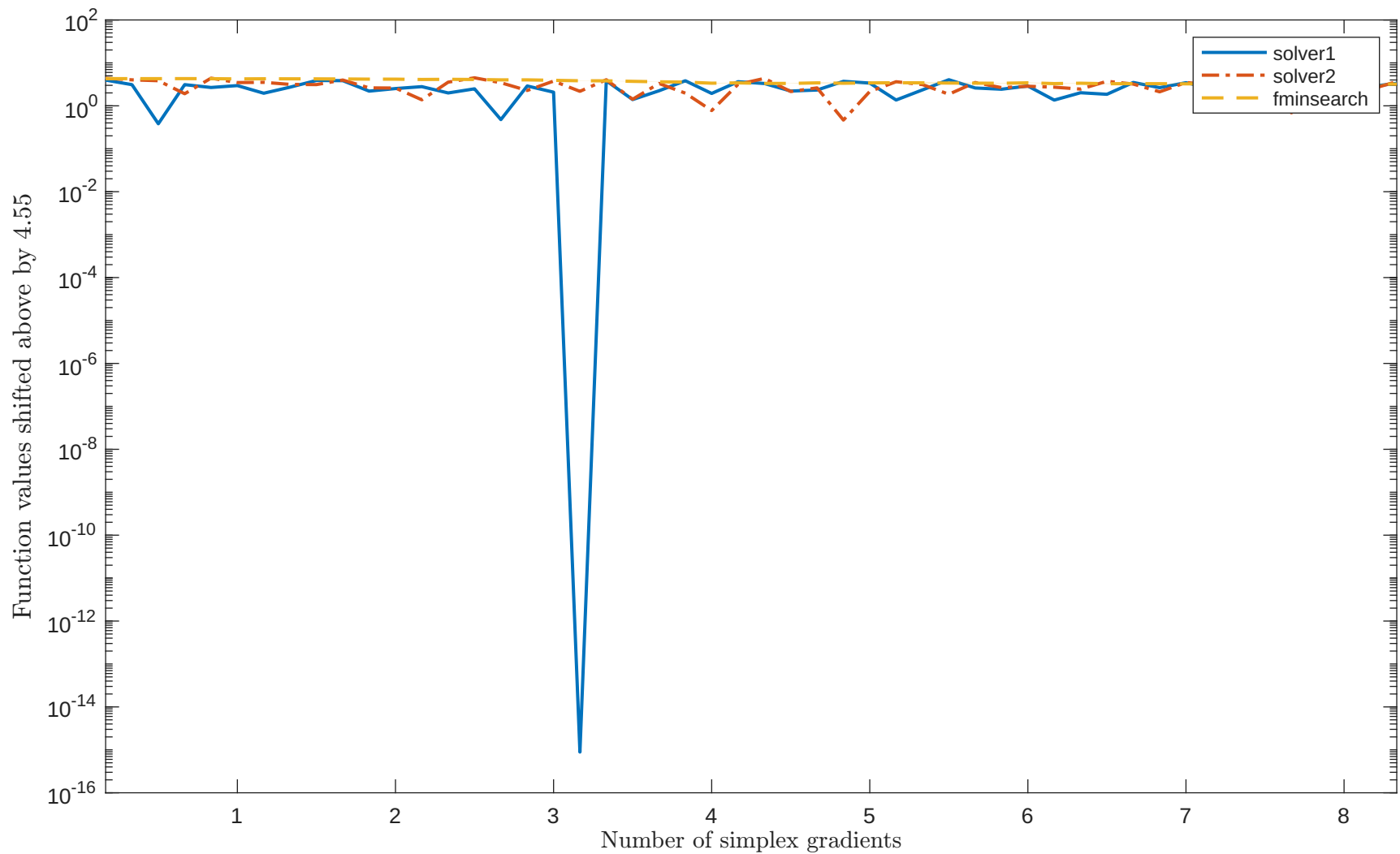
Solving "SENSORS" with "noisy_0.001_mixed_gaussian" feature
