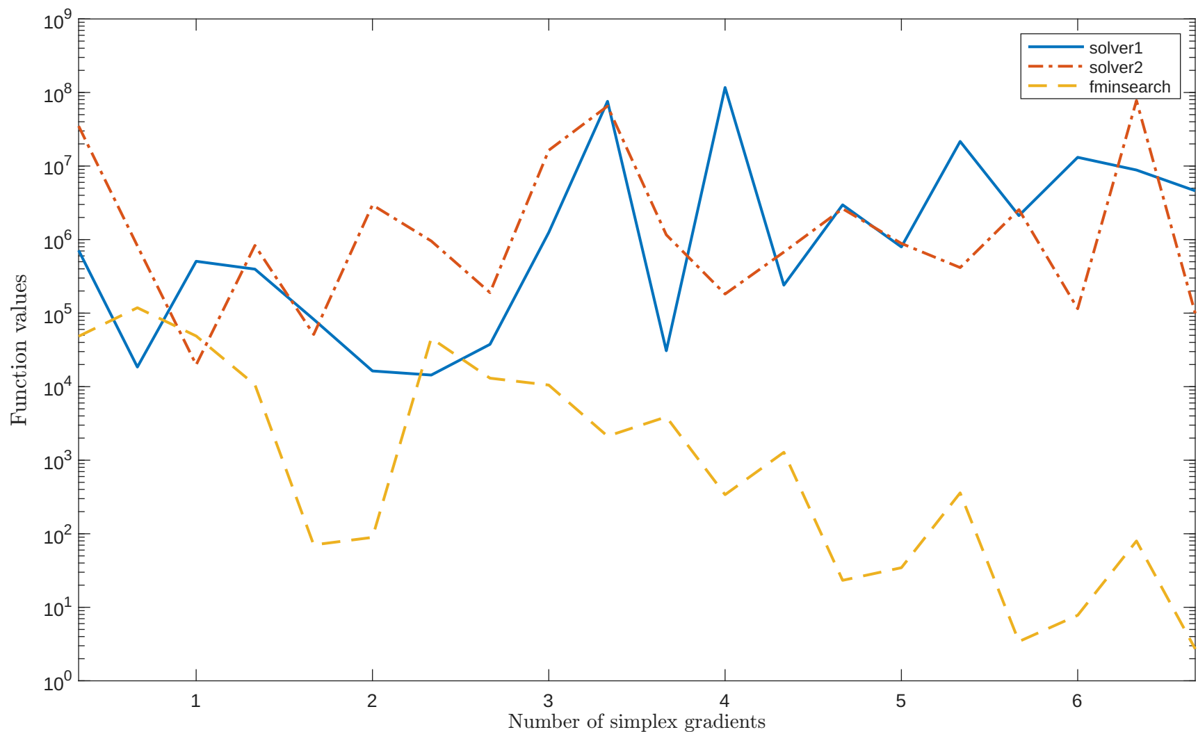
Solving “MARATOSB” with “noisy_0.001_mixed_gaussian” feature
