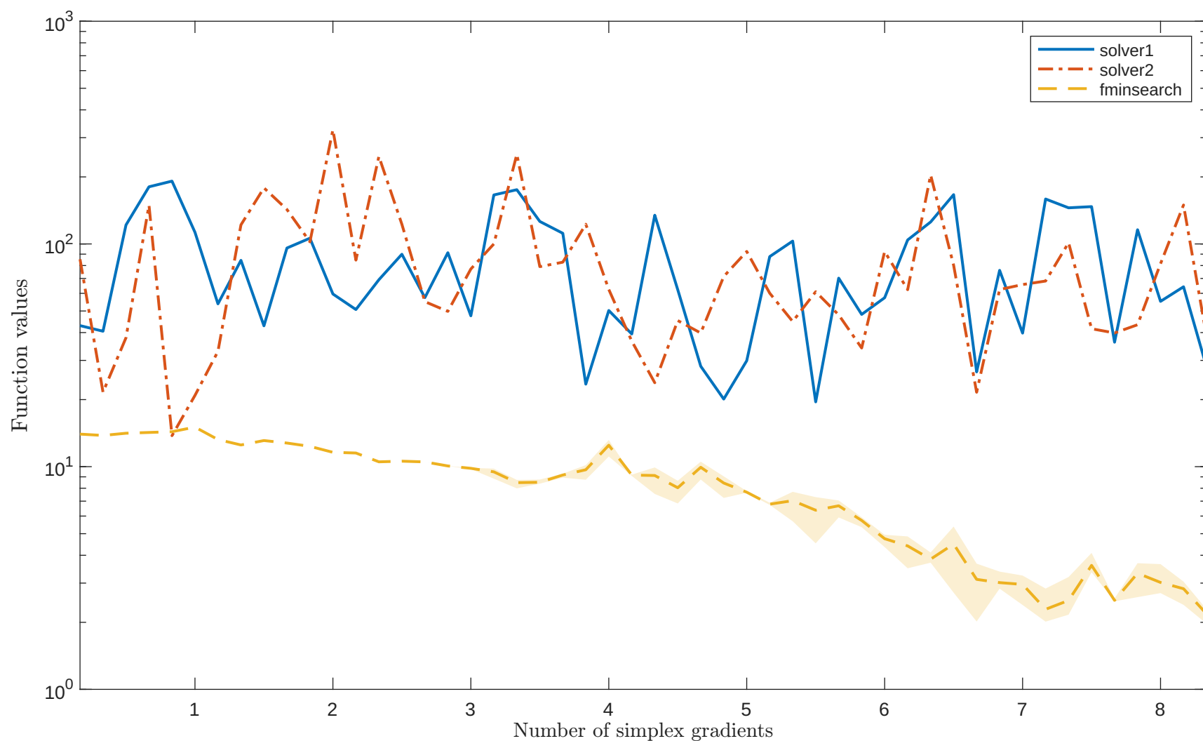
Solving "TRIDIA" with "noisy_0.001_mixed_gaussian" feature
