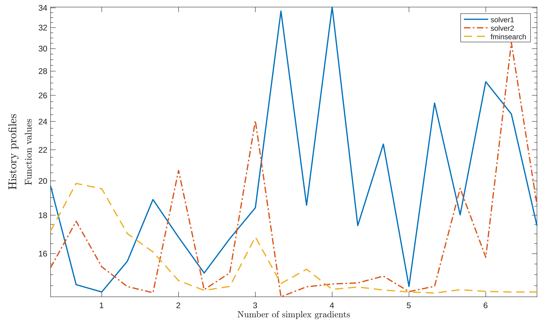
Solving “SNAIL” with “noisy_0.001_mixed_gaussian” feature
