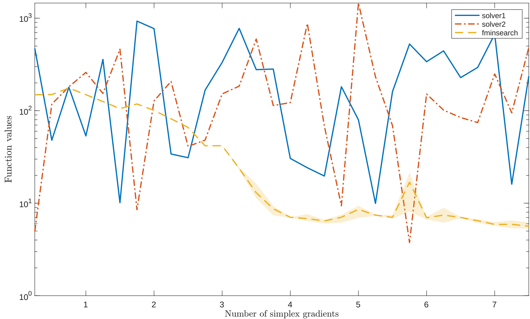
Solving “DENSCHNE” with “noisy_0.001_mixed_gaussian” feature
