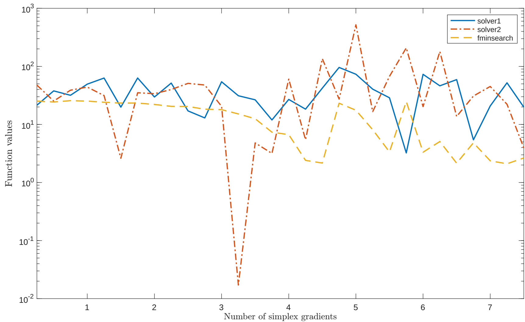
Solving “HATFLDD” with “noisy_0.001_mixed_gaussian” feature
