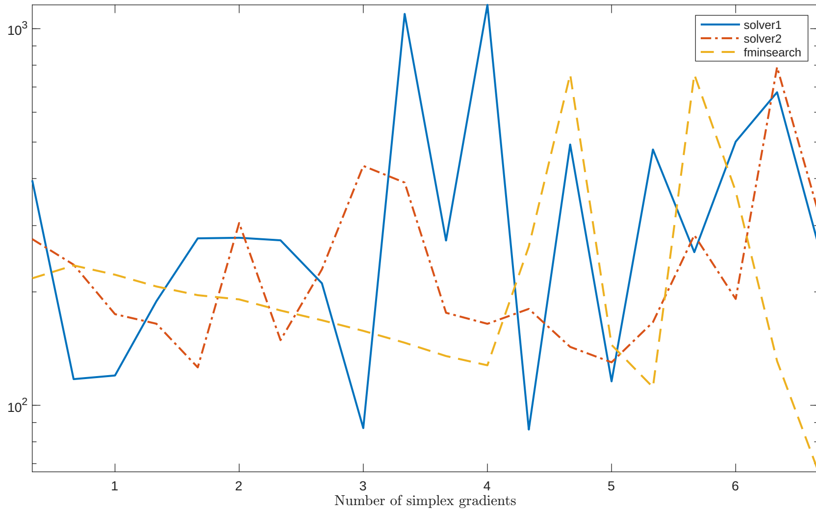
Solving "POWELLSQLS" with "noisy_0.001_mixed_gaussian" feature
