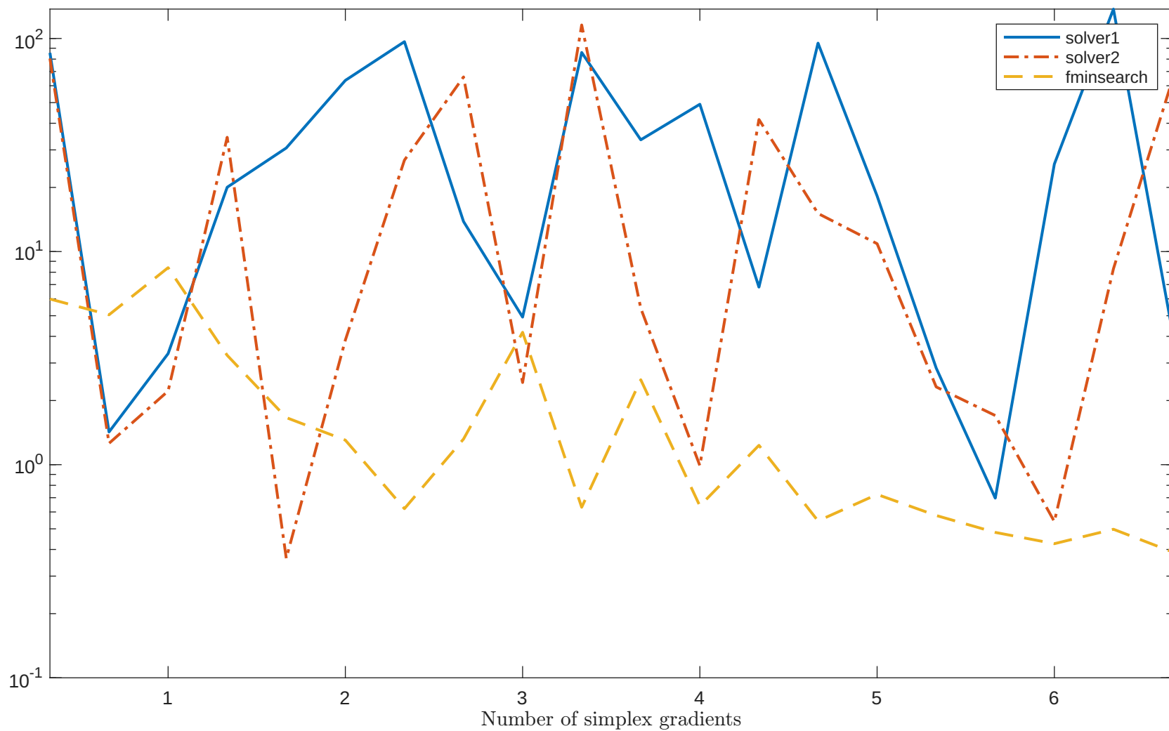
Solving “BRKMCC” with “noisy_0.001_mixed_gaussian” feature
