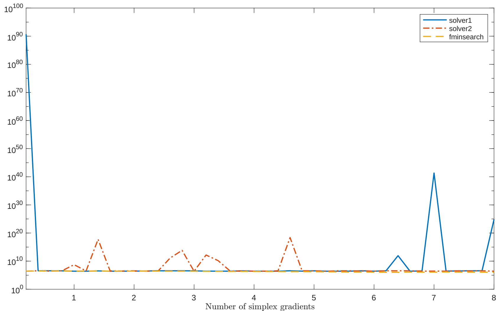
Solving "RAT43LS" with "noisy_0.001_mixed_gaussian" feature
