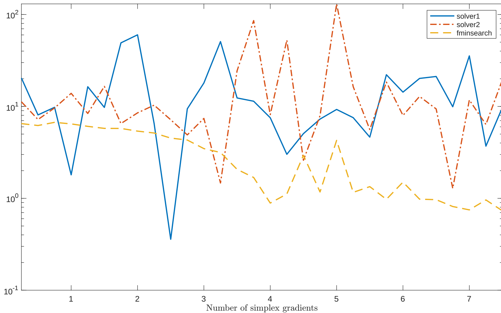
Solving "SSI" with "noisy_0.001_mixed_gaussian" feature
