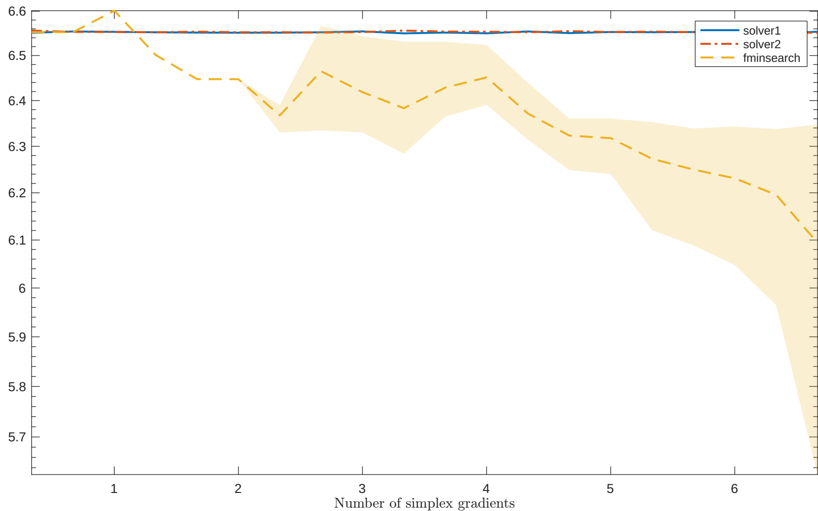
Solving "LOGHAIRY" with "noisy_0.001_mixed_gaussian" feature
