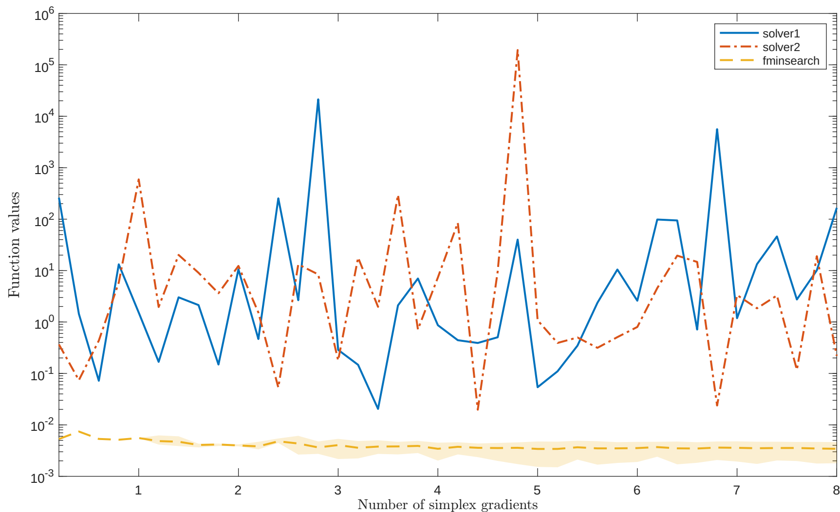
Solving “KOWOSB” with “noisy_0.001_mixed_gaussian” feature
