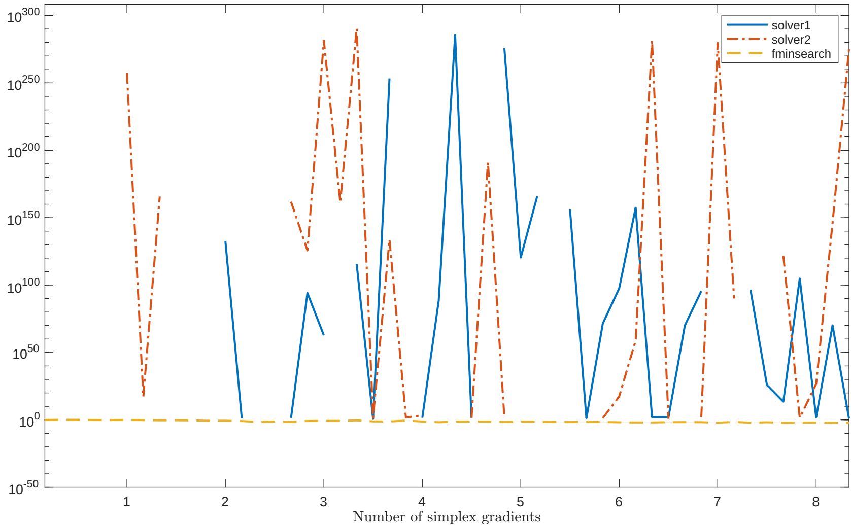
Solving “OSBORNEA” with “noisy_0.001_mixed_gaussian” feature
