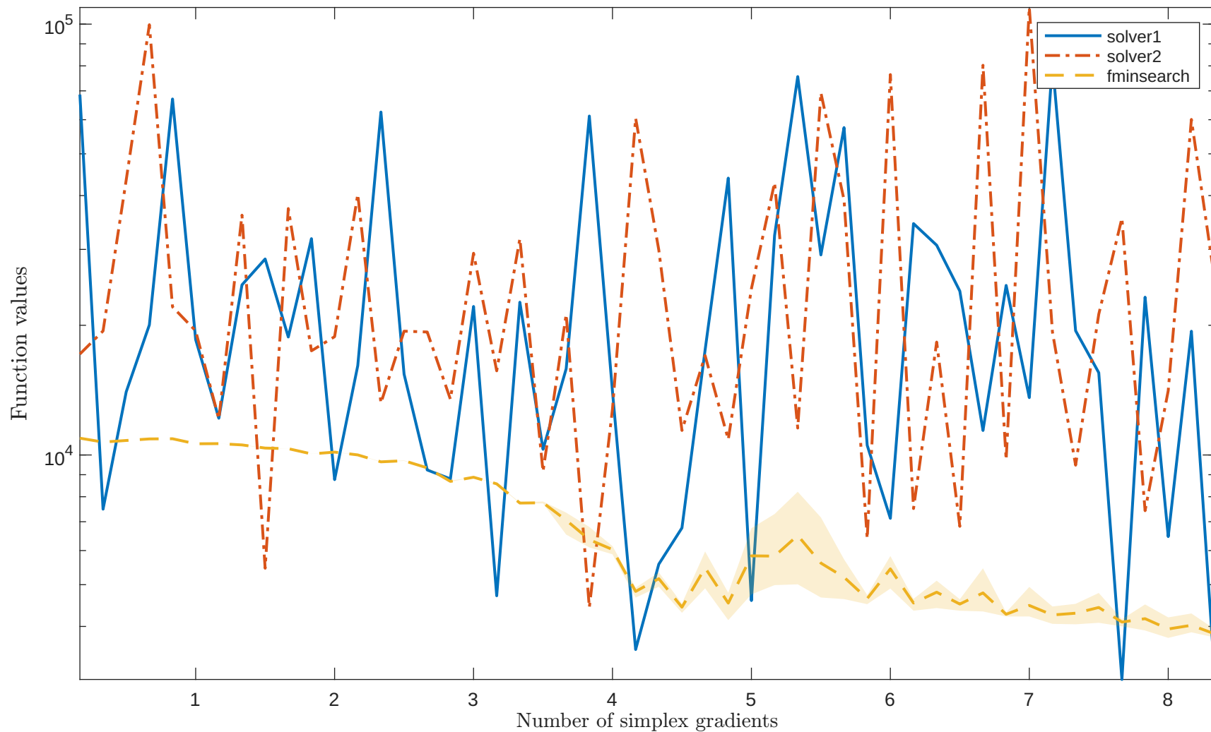
Solving “DEVGLA2” with “noisy_0.001_mixed_gaussian” feature
