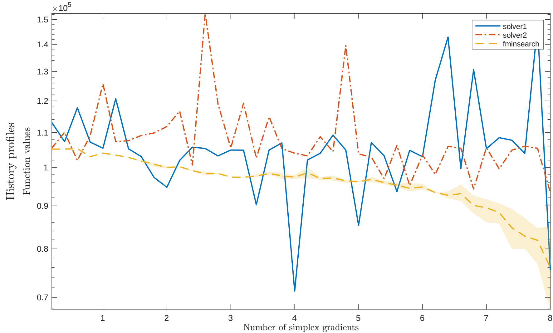
Solving “DEVGLA1” with “noisy_0.001_mixed_gaussian” feature
