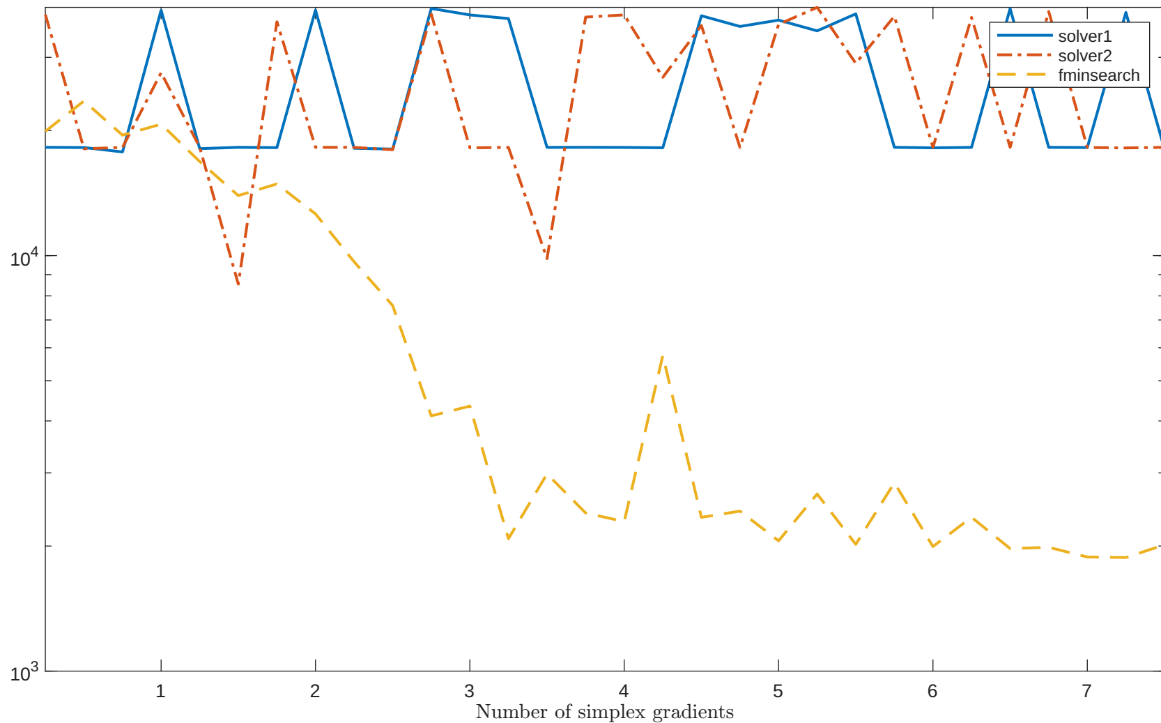
Solving "RAT42LS" with "noisy_0.001_mixed_gaussian" feature
