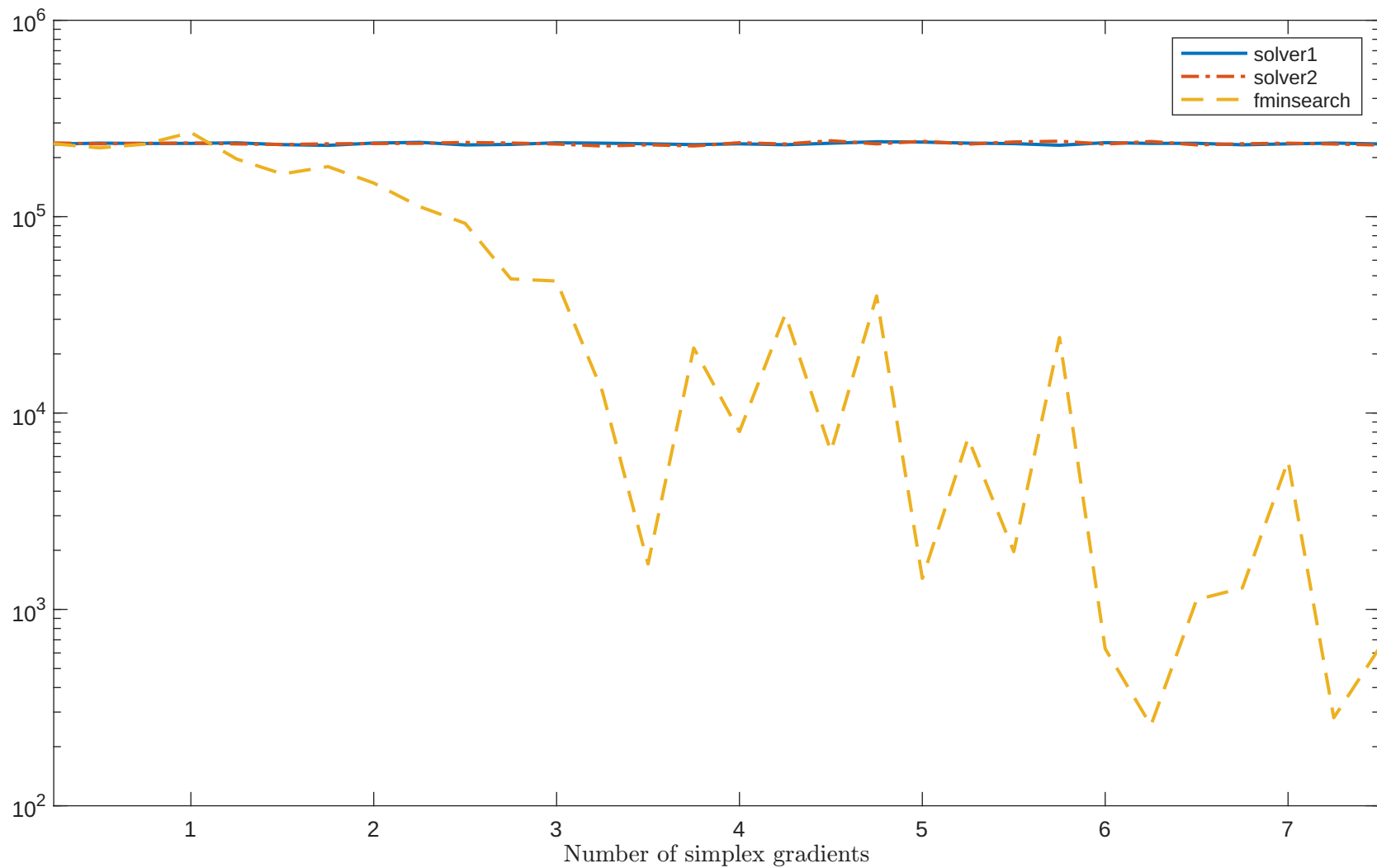
Solving “LSC2LS” with “noisy_0.001_mixed_gaussian” feature
