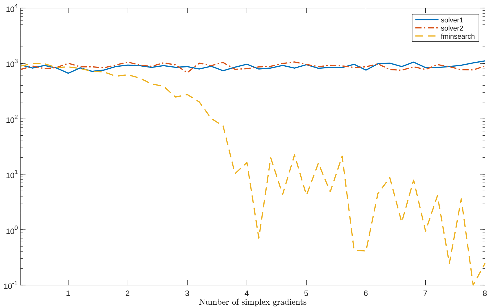
Solving “MGH09LS” with “noisy_0.001_mixed_gaussian” feature
