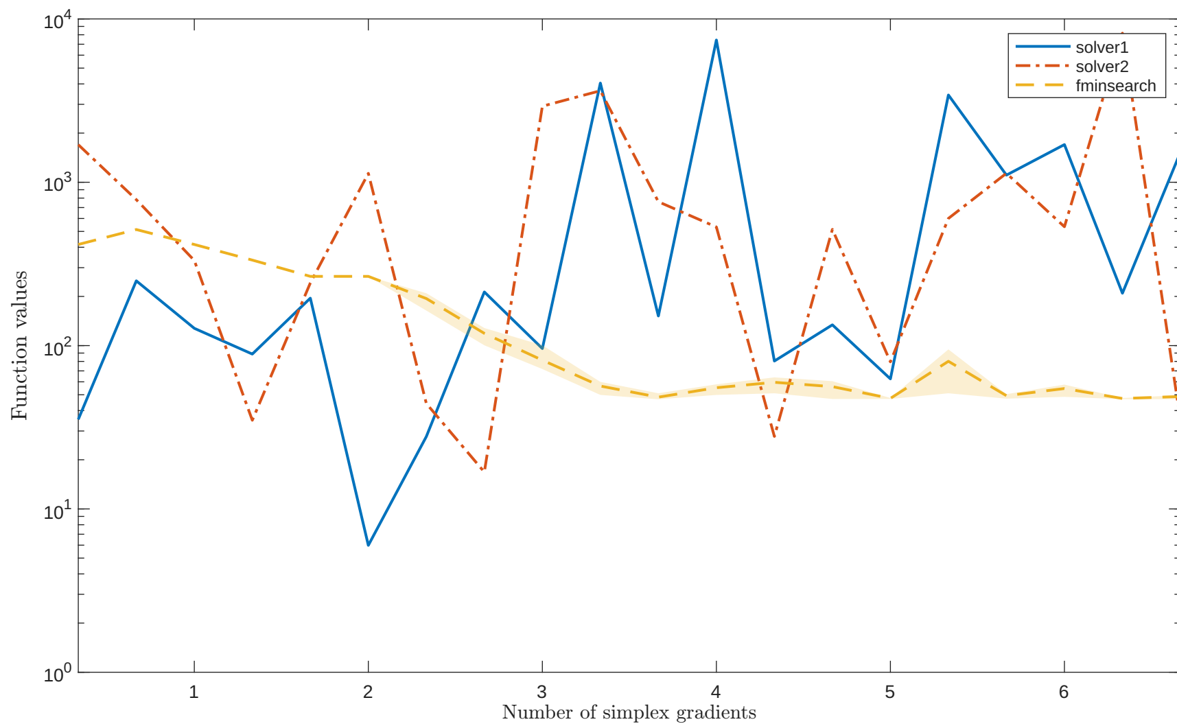
Solving “DENSCHNF” with “noisy_0.001_mixed_gaussian” feature
