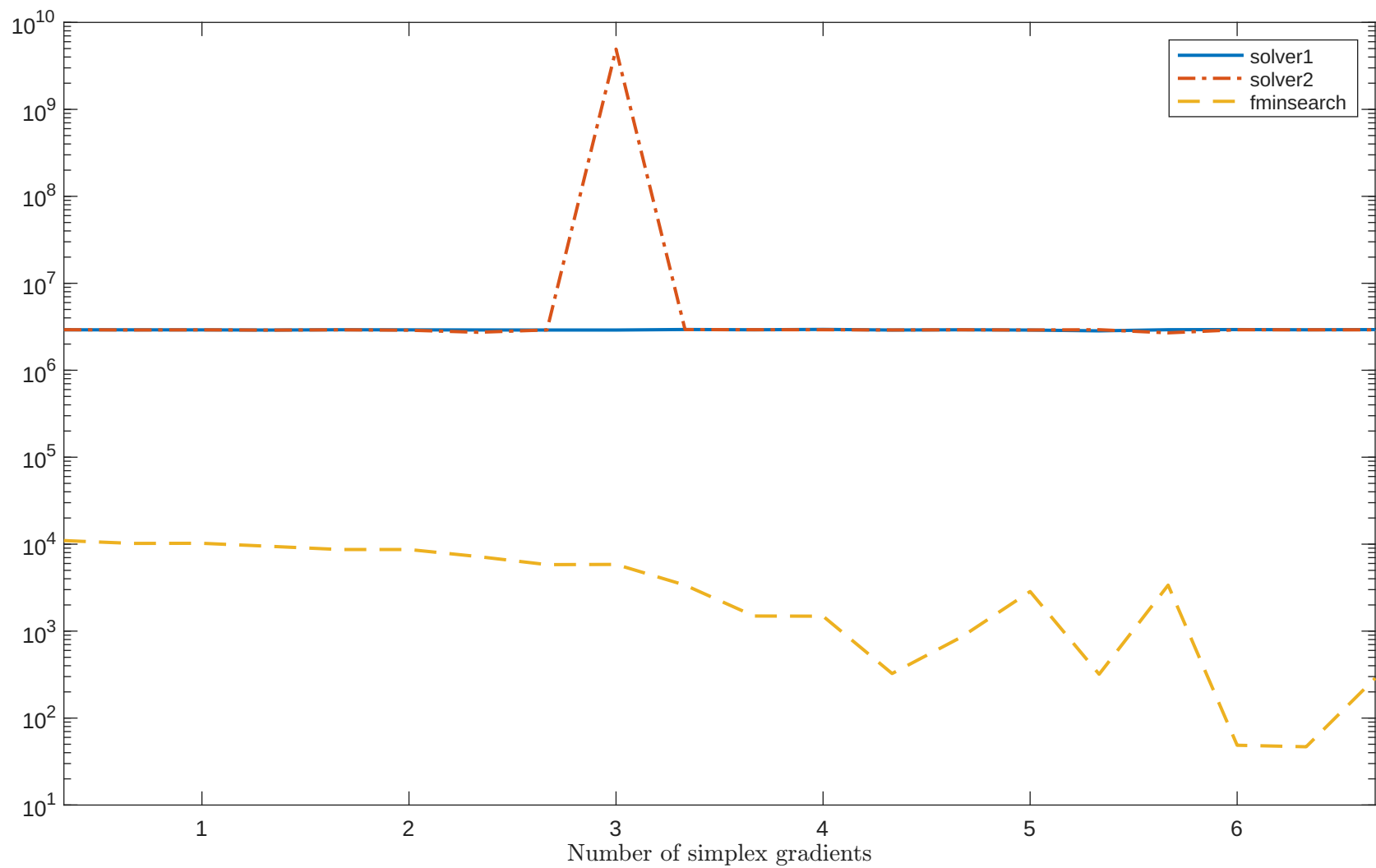
Solving “MISRA1BLS” with “noisy_0.001_mixed_gaussian” feature
