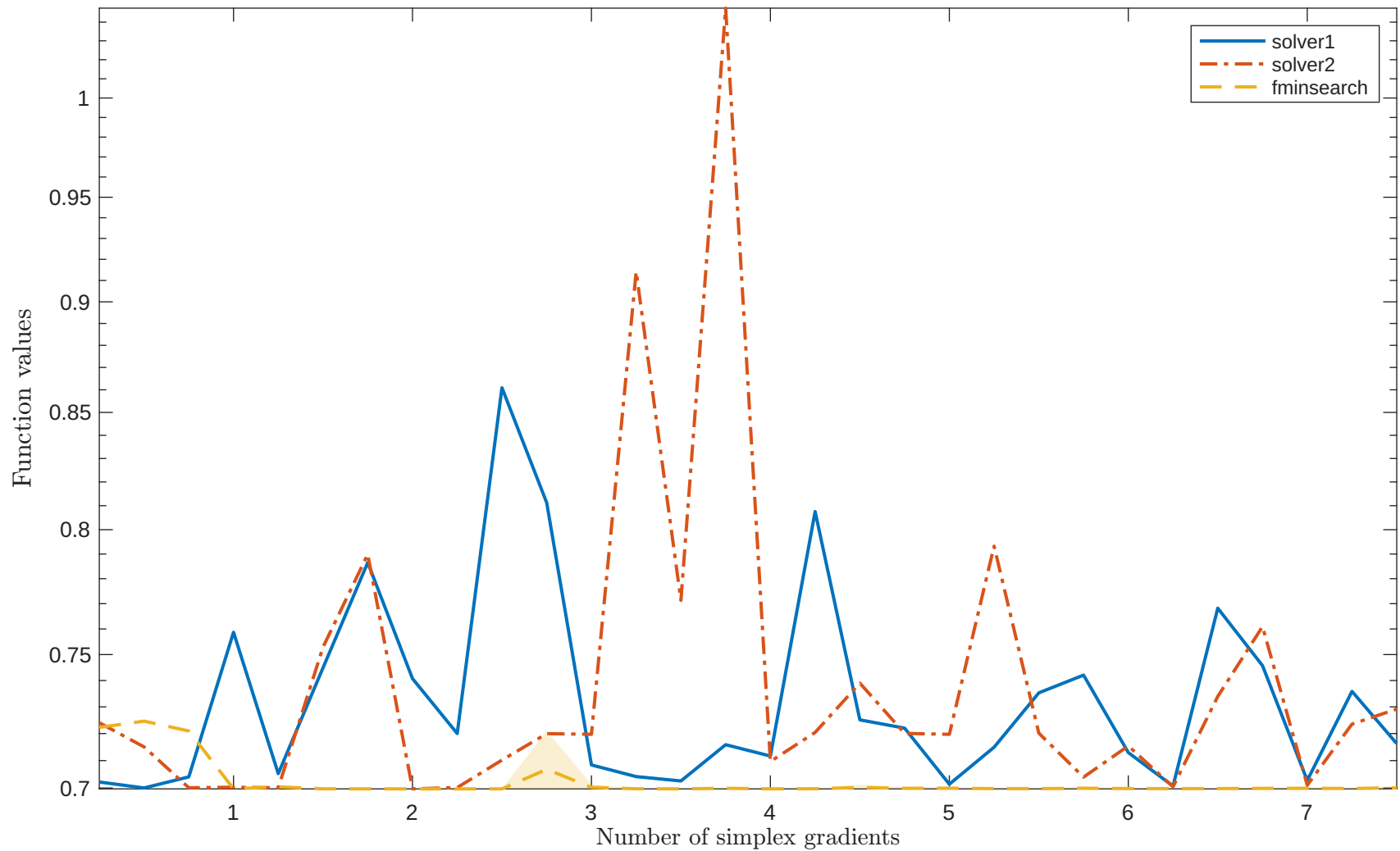
Solving "ECKERLE4LS" with "noisy_0.001_mixed_gaussian" feature
