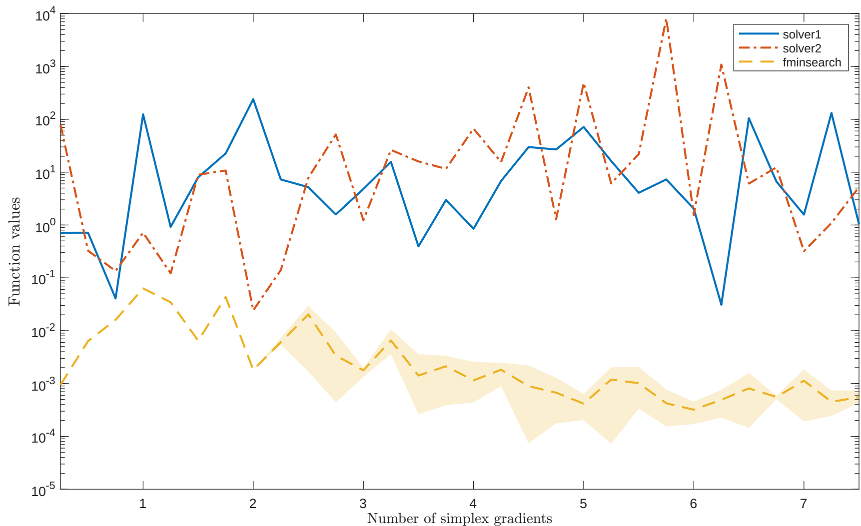
Solving “HATFLDFL” with “noisy_0.001_mixed_gaussian” feature
