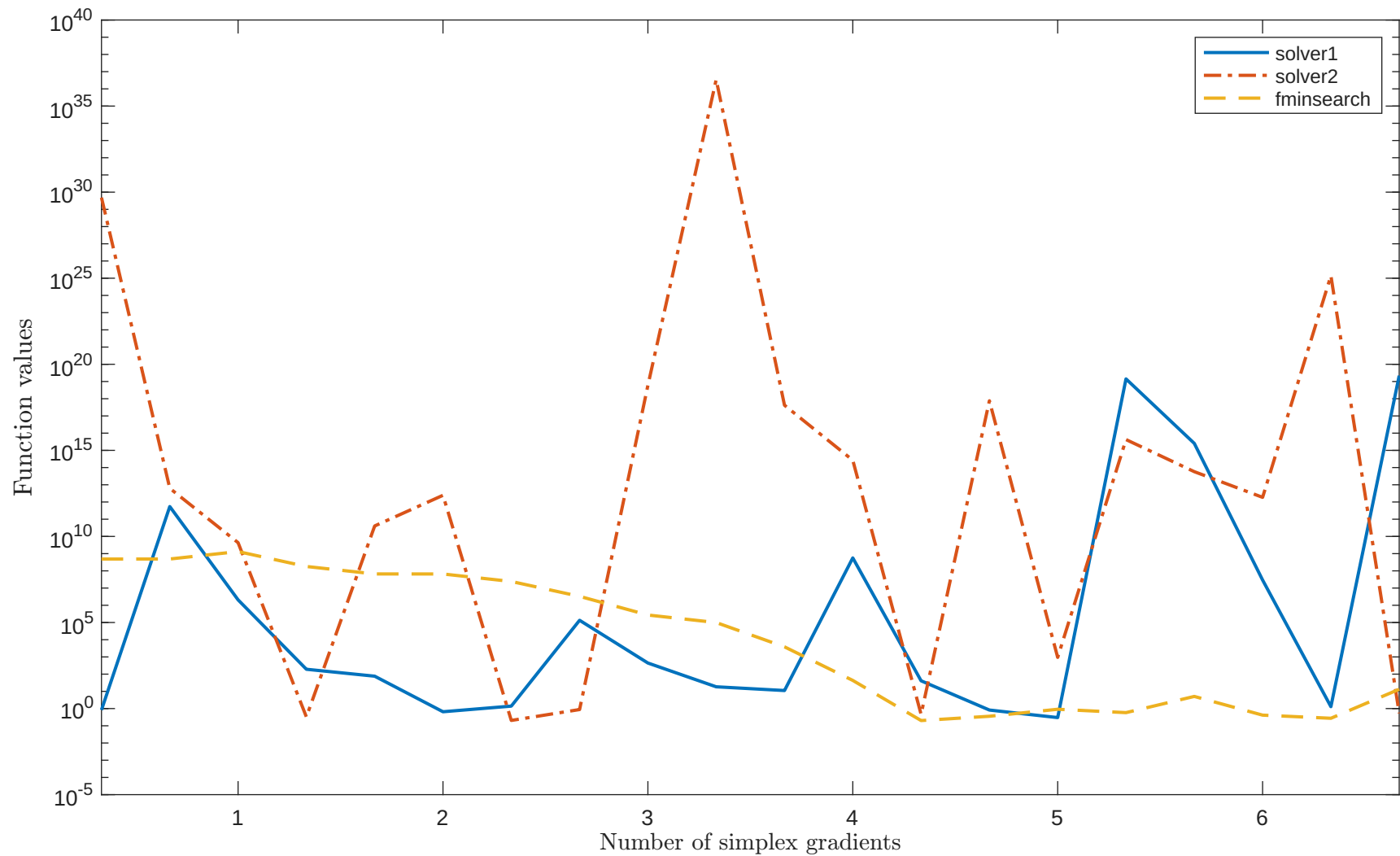
Solving “CLIFF” with “noisy_0.001_mixed_gaussian” feature
