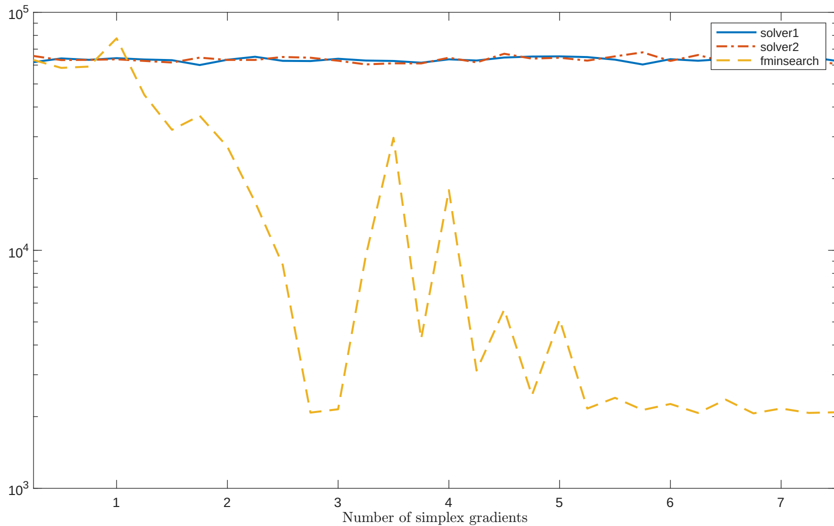
Solving "LSC1LS" with "noisy_0.001_mixed_gaussian" feature
