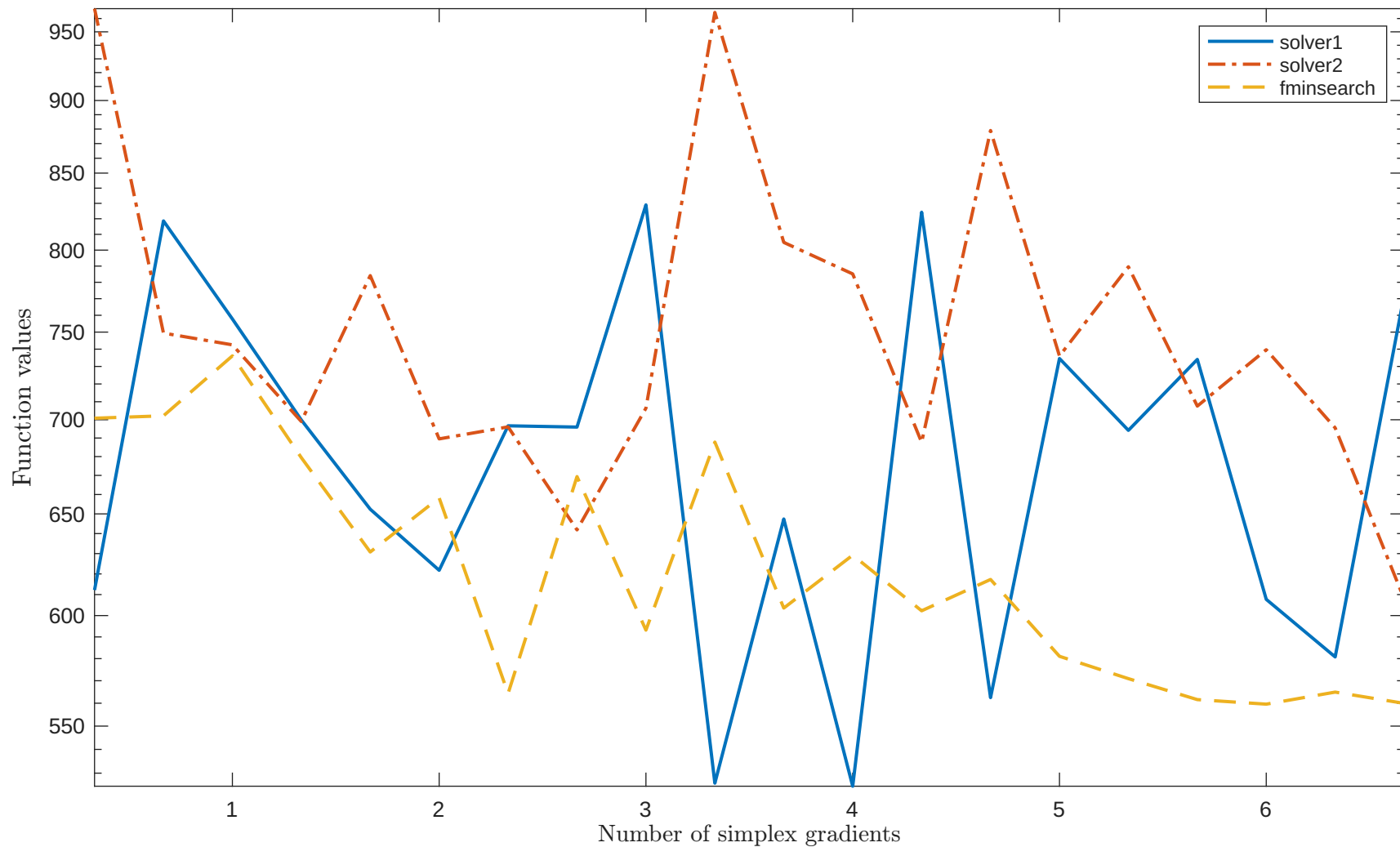
Solving "HAIRY" with "noisy_0.001_mixed_gaussian" feature
