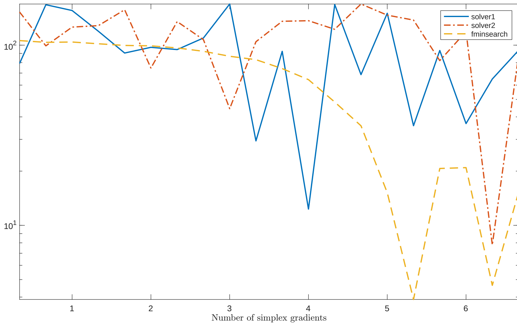
Solving "HIMMELBCLS" with "noisy_0.001-mixed-gaussian" feature
