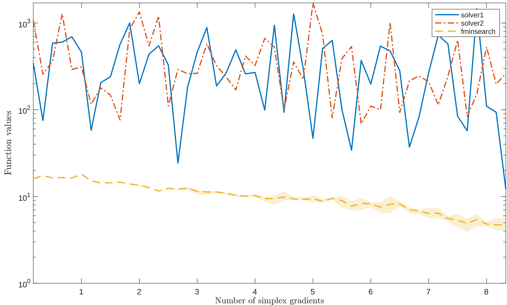
Solving “BROYDN3DLS” with “noisy_0.001_mixed_gaussian” feature
