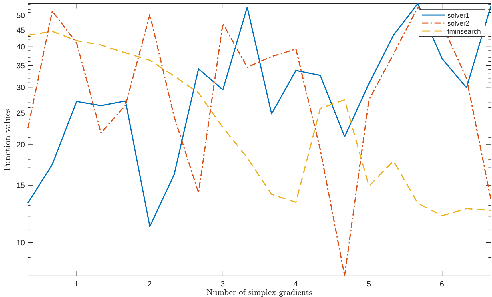
Solving "EGGCRATE" with "noisy_0.001_mixed_gaussian" feature
