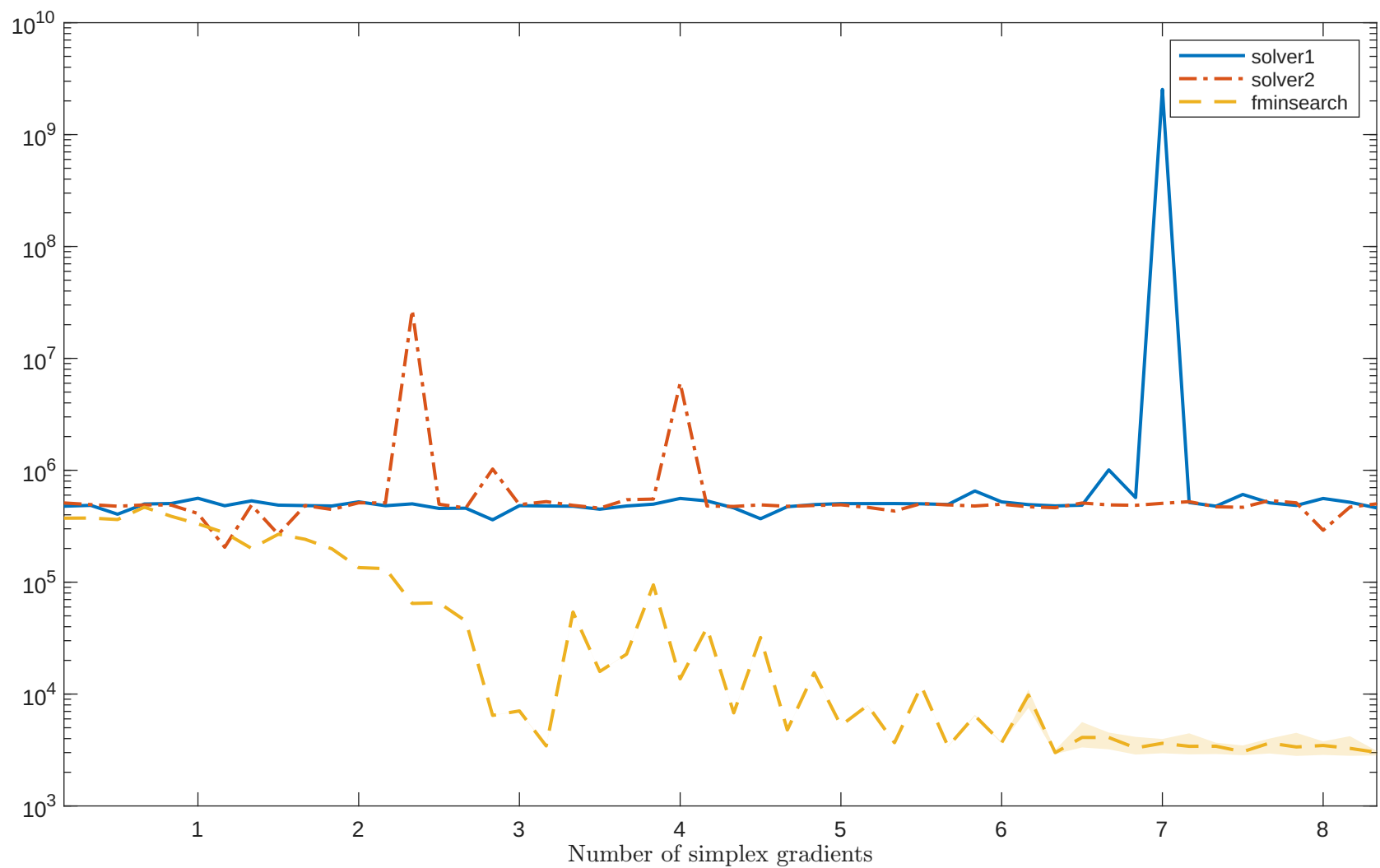
Solving "KIRBY2LS" with "noisy_0.001_mixed_gaussian" feature
