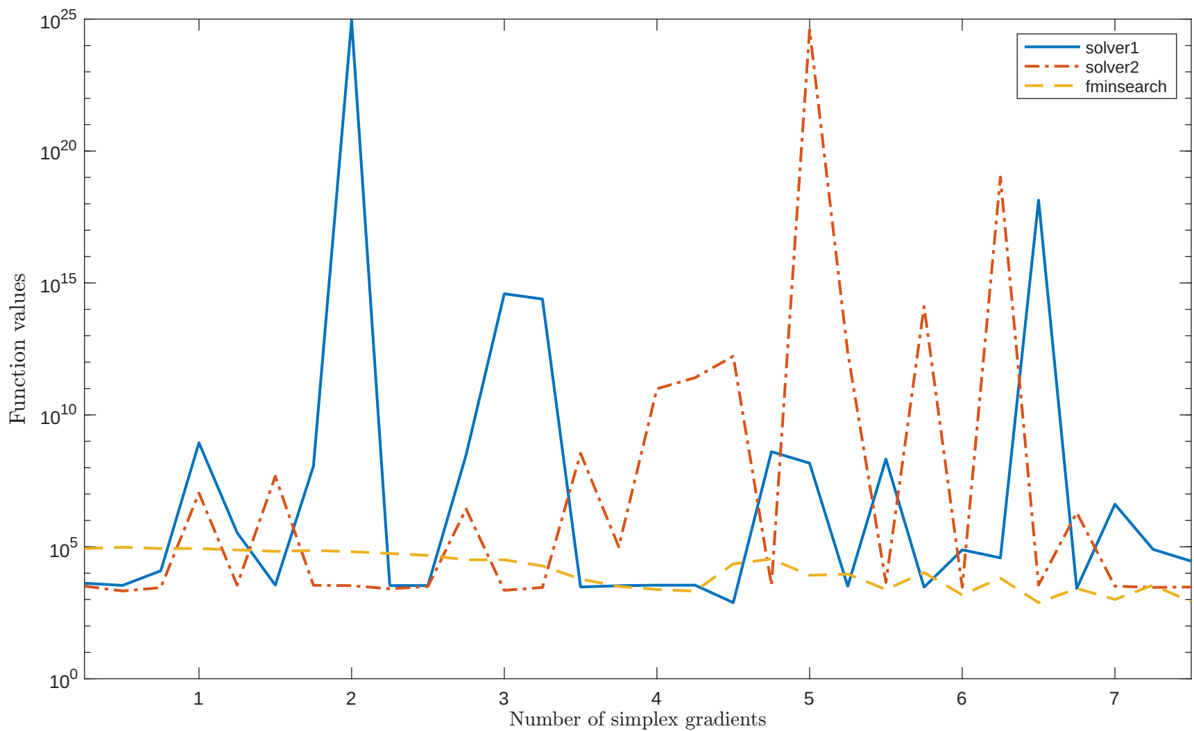
Solving “GROWTHLS” with “noisy_0.001_mixed_gaussian” feature
