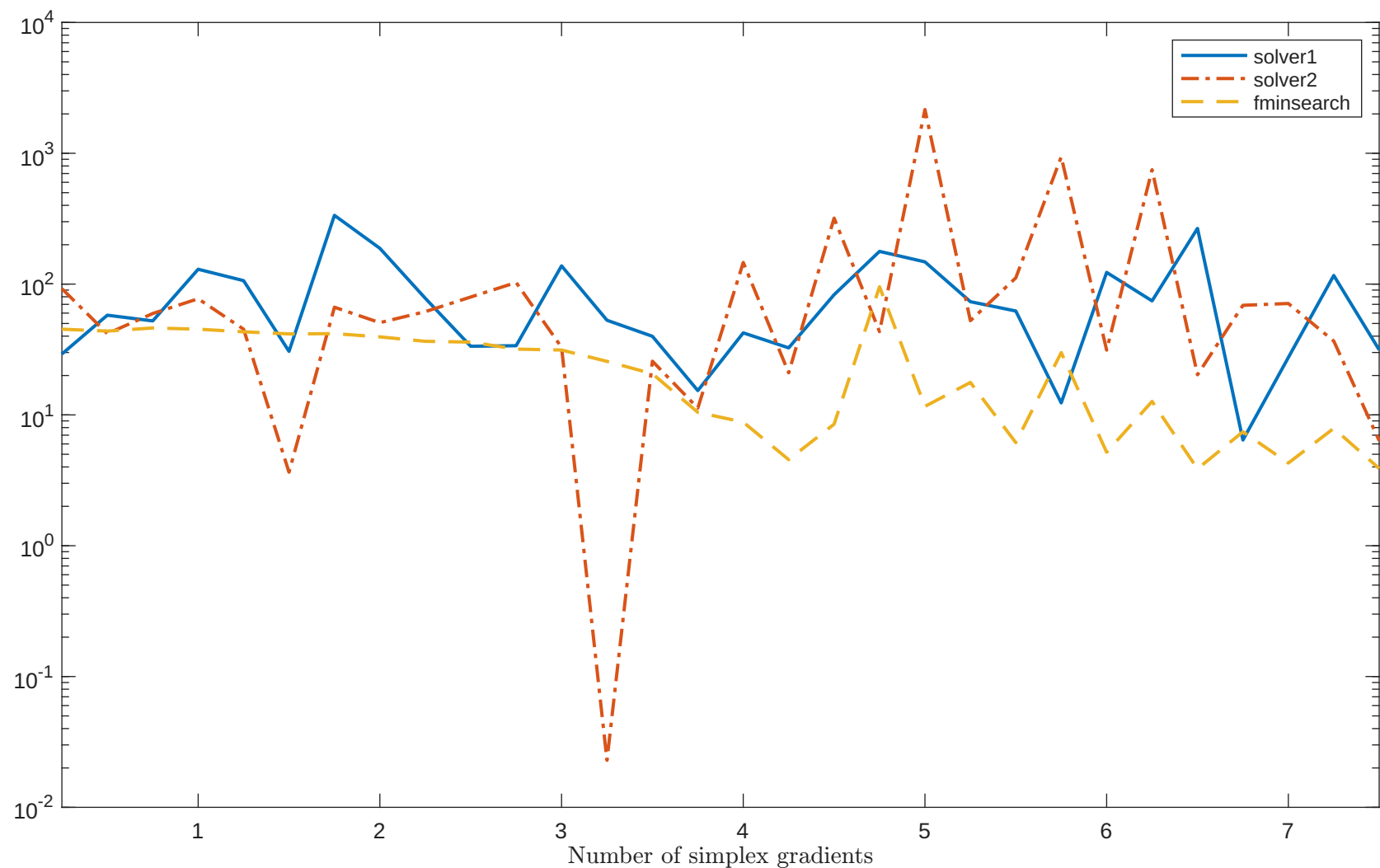
Solving “HATFLDE” with “noisy_0.001_mixed_gaussian” feature
