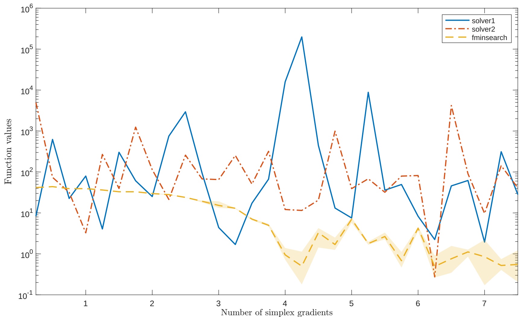
Solving “BARD” with “noisy_0.001_mixed_gaussian” feature
