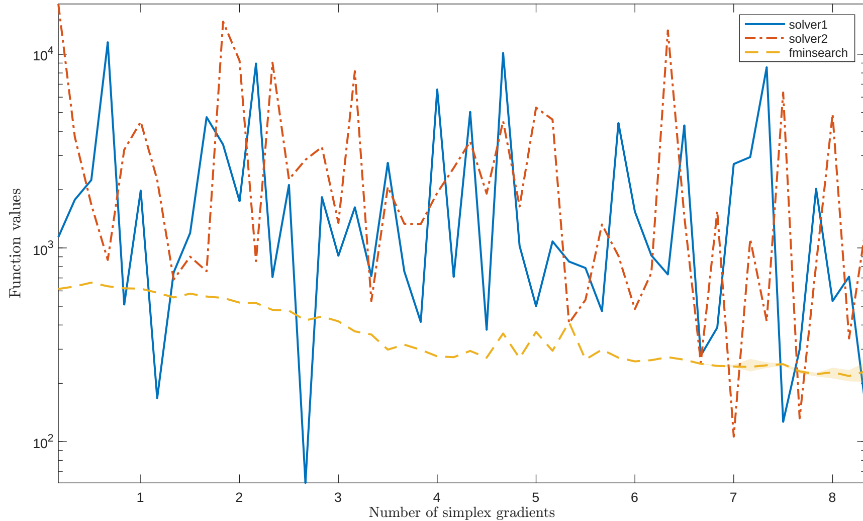
Solving "CHNRSNBM" with "noisy_0.001_mixed-gaussian" feature
