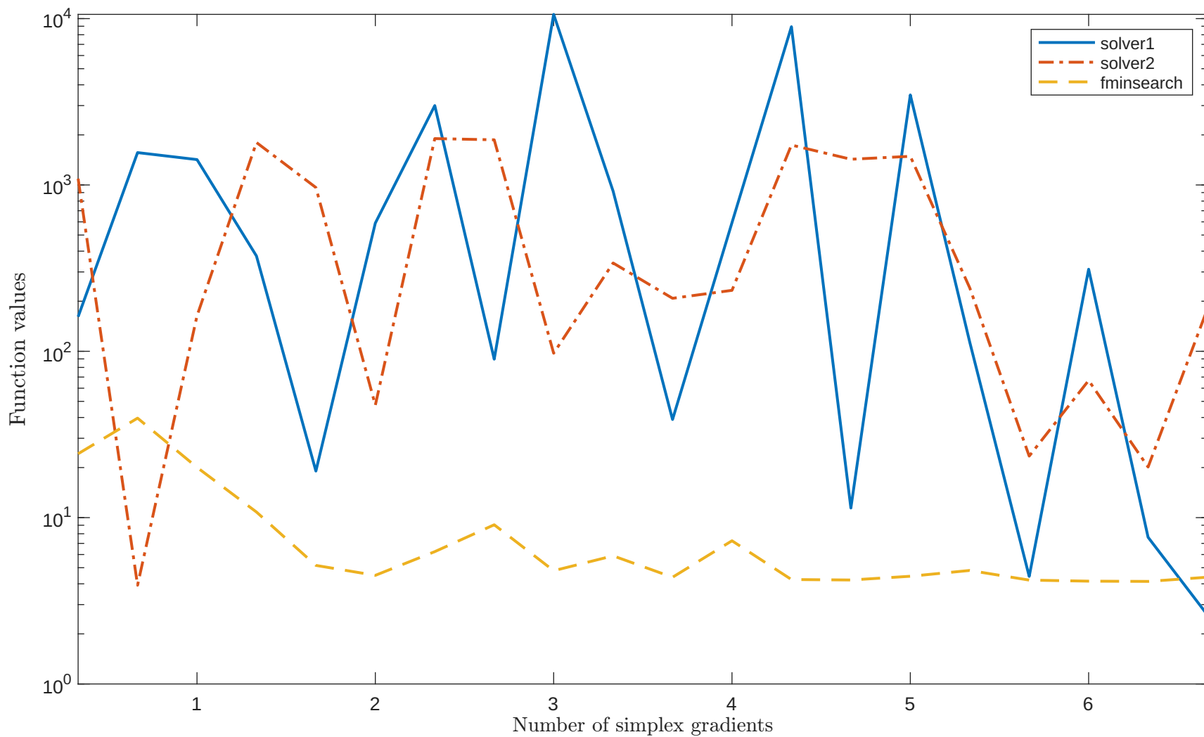
Solving "ROSENBR" with "noisy_0.001_mixed_gaussian" feature
