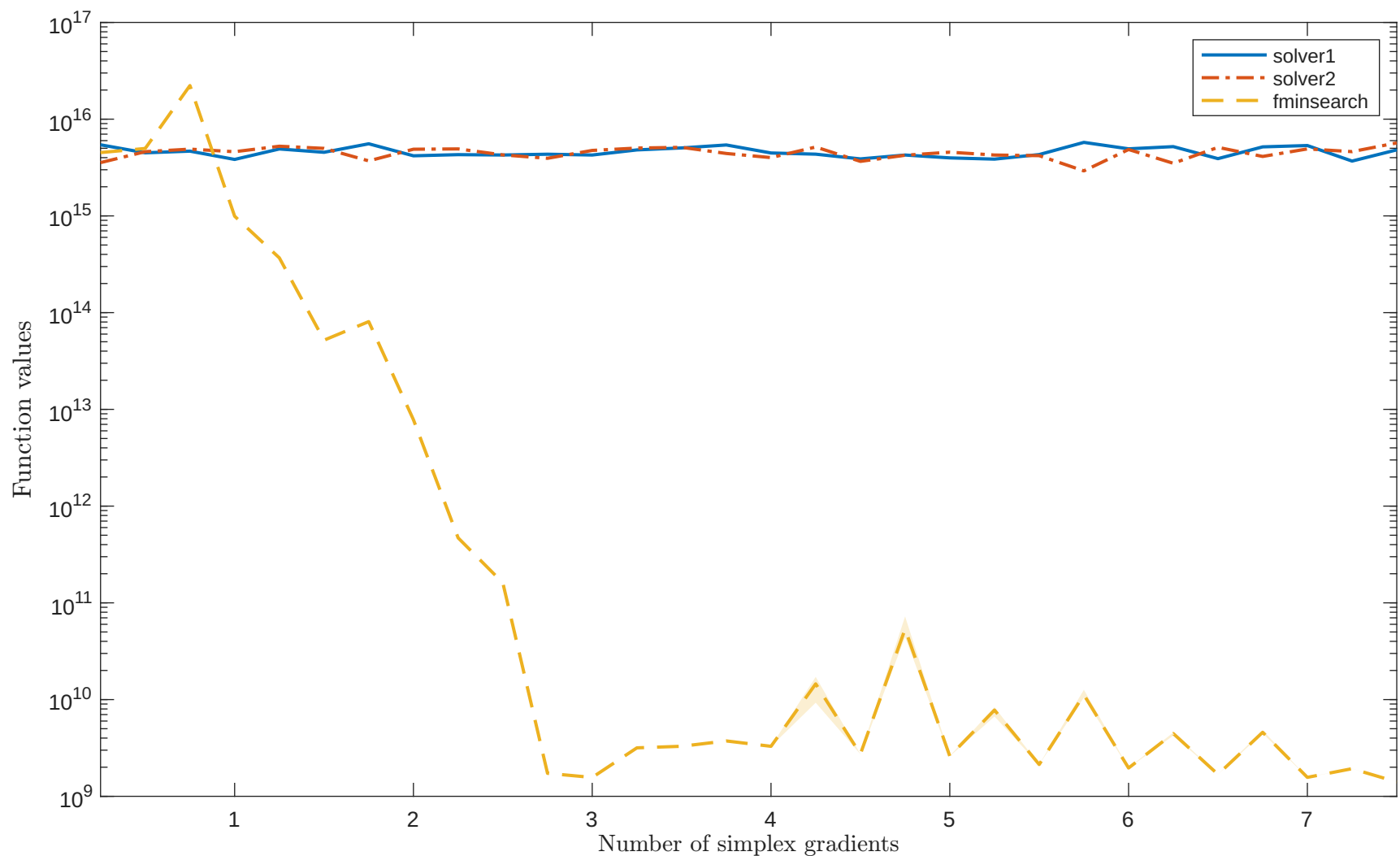
Solving “MGH10SLS” with “noisy_0.001_mixed_gaussian” feature
