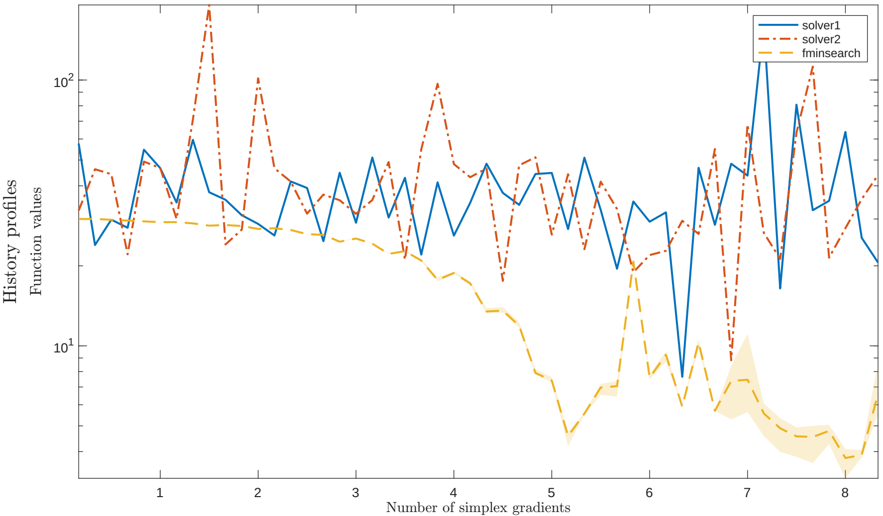
Solving “QING” with “noisy_0.001_mixed_gaussian” feature
