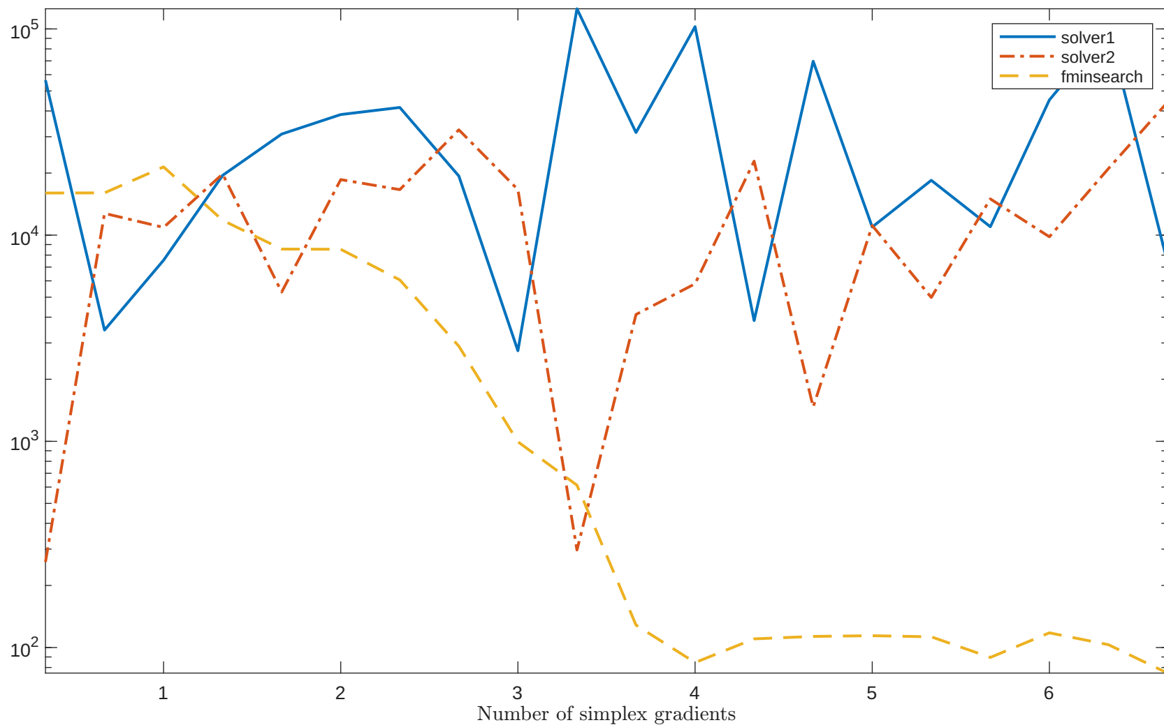
Solving "ELATVIDU" with "noisy_0.001_mixed_gaussian" feature
