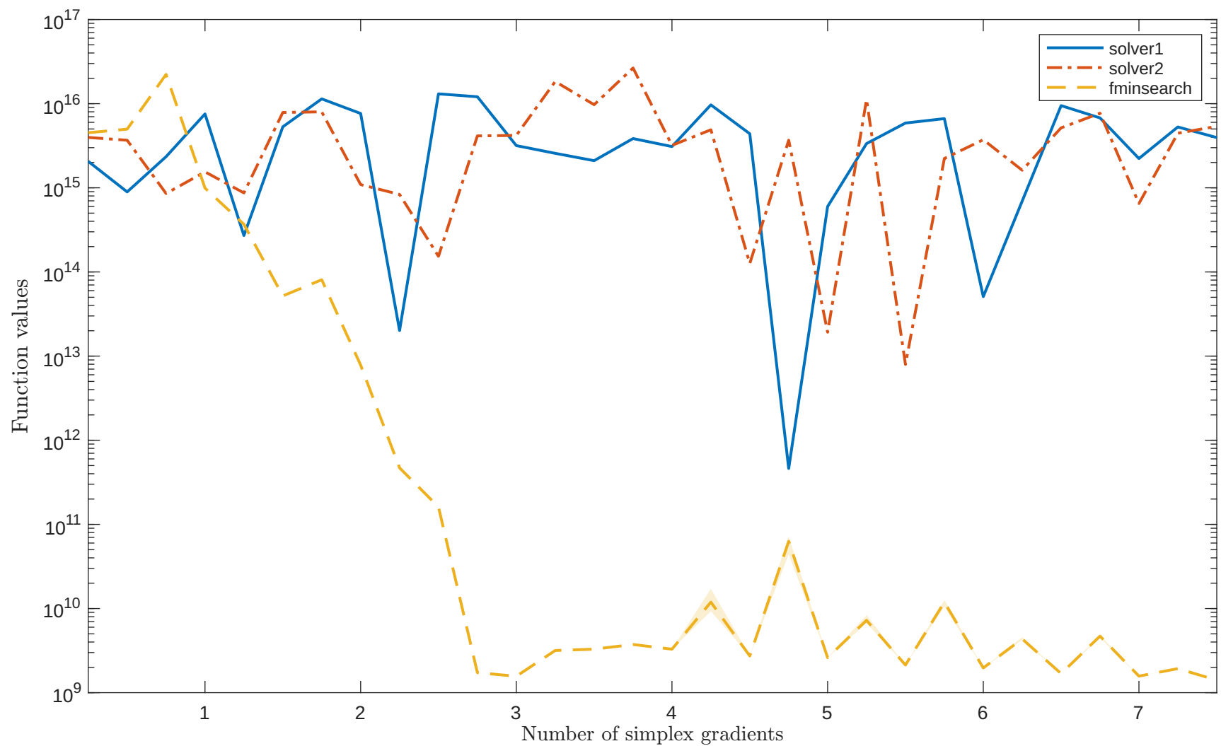
Solving “MGH10LS” with “noisy_0.001_mixed_gaussian” feature
