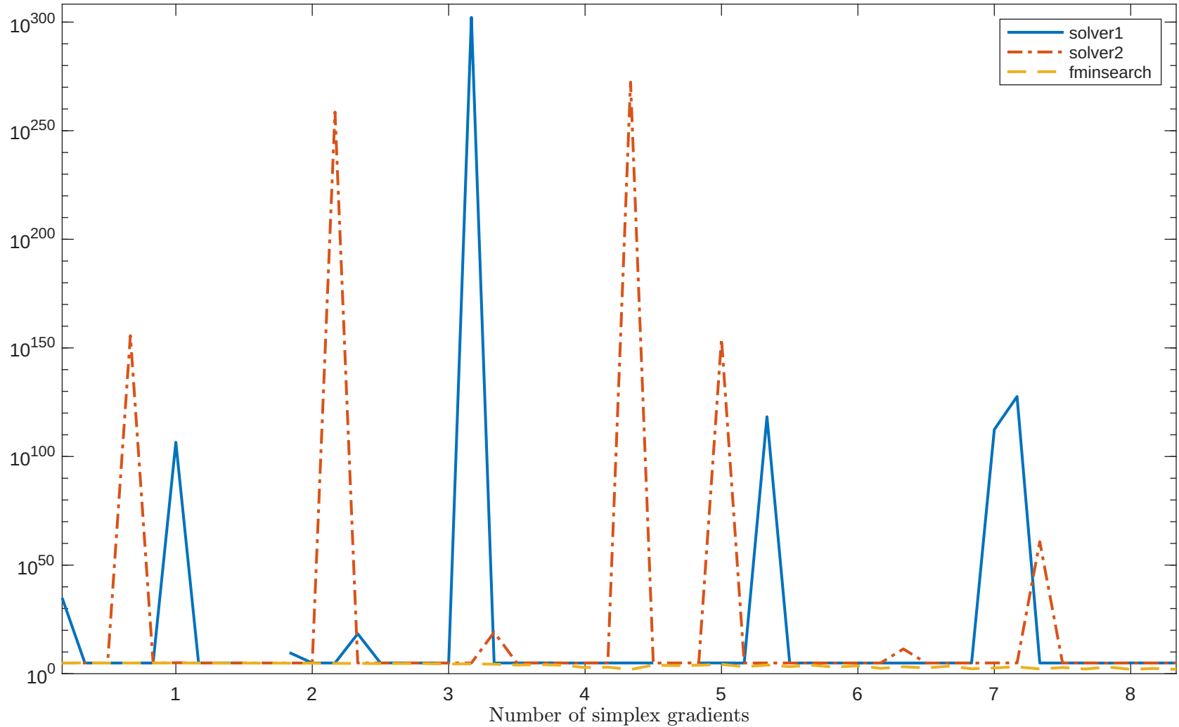
Solving “MGH17LS” with “noisy_0.001_mixed_gaussian” feature
