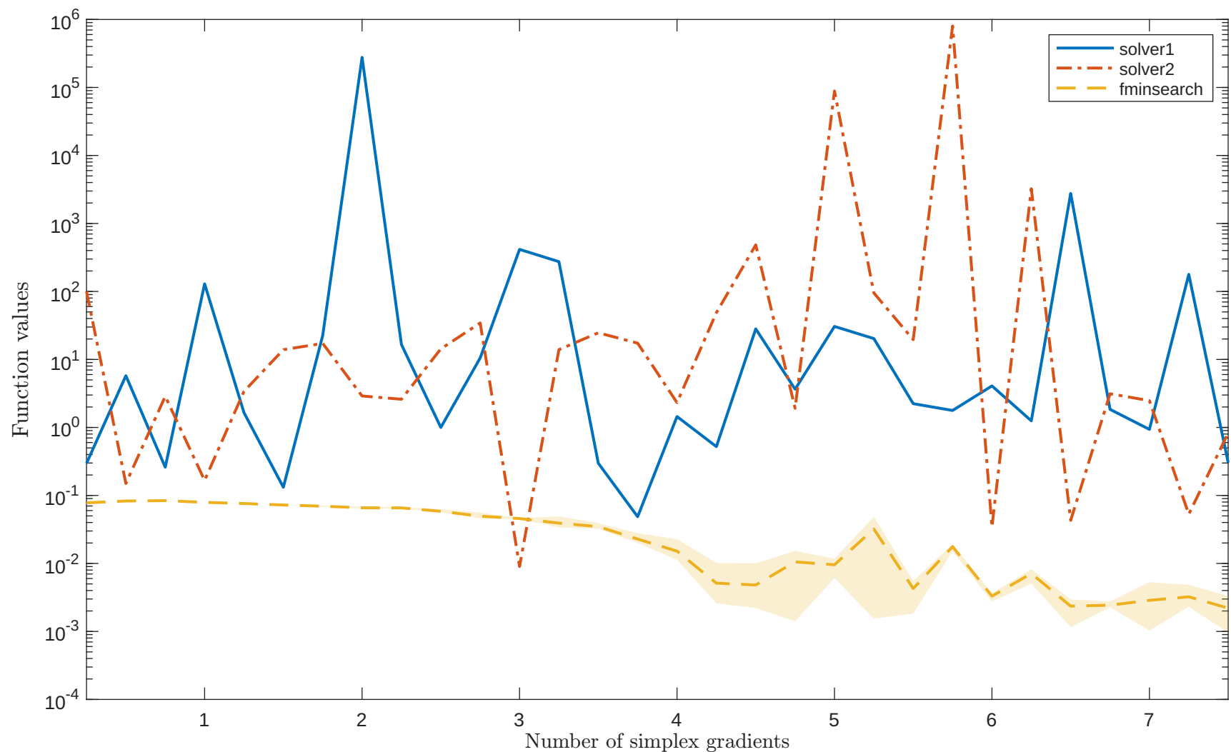
Solving "HATFLDFLS" with "noisy_0.001_mixed_gaussian" feature
