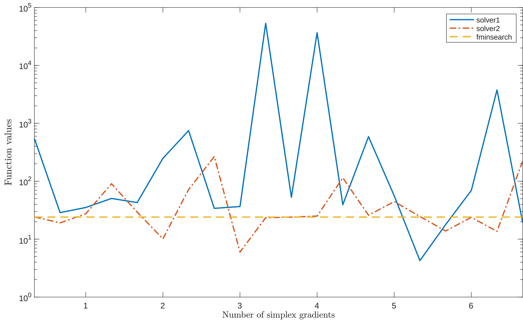
Solving “EXPFIT” with “noisy_0.001_mixed-gaussian” feature
