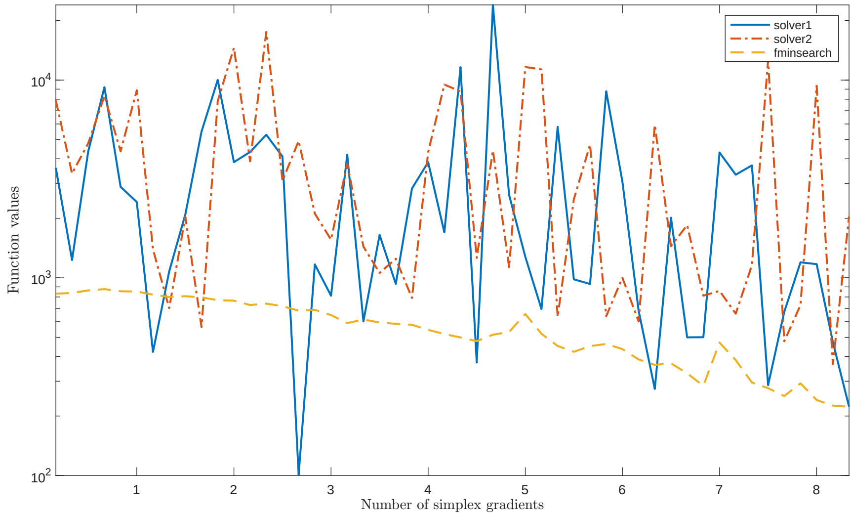
Solving “CHNROSNB” with “noisy_0.001_mixed_gaussian” feature
