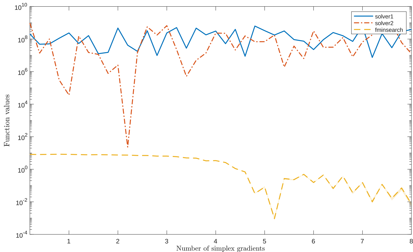
Solving "ROSZMAN1LS" with "noisy_0.001_mixed_gaussian" feature
