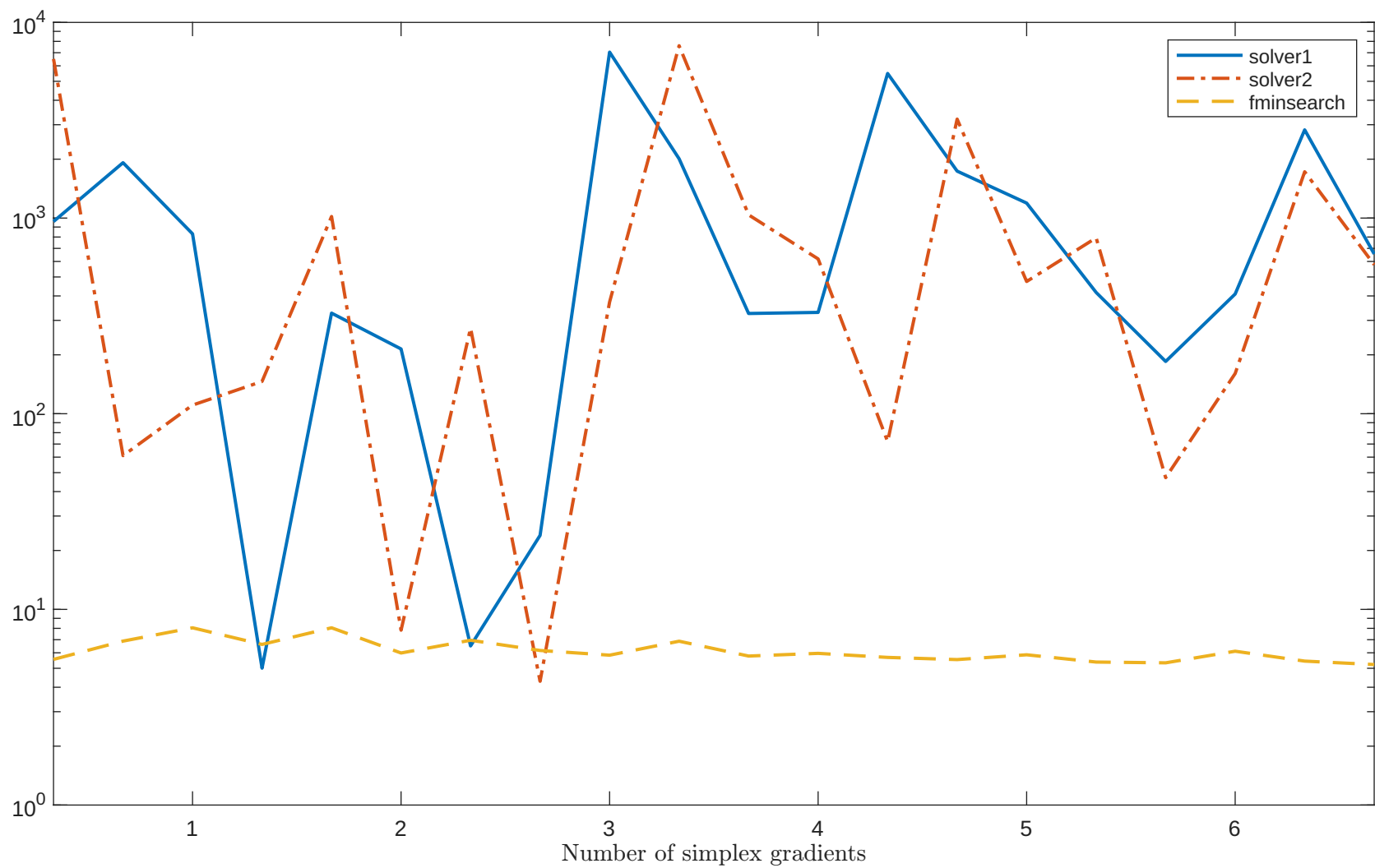
Solving "SINEVAL" with "noisy_0.001_mixed_gaussian" feature
