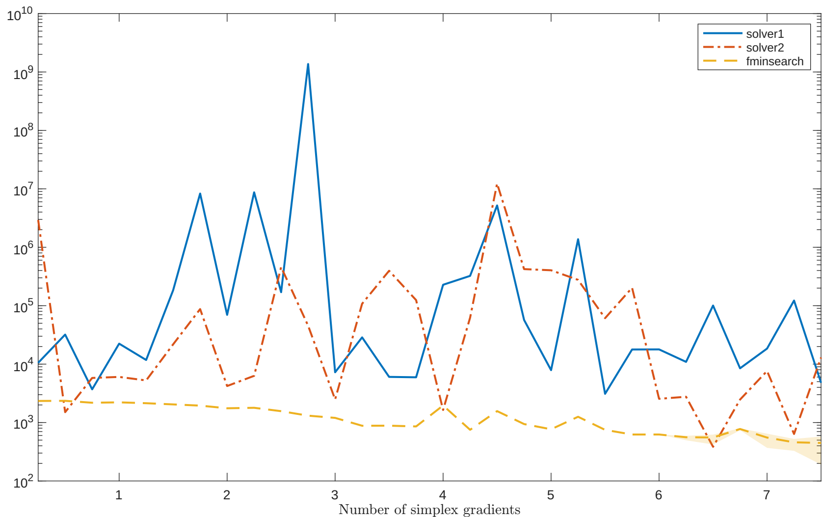
Solving “YFITU” with “noisy_0.001_mixed_gaussian” feature
