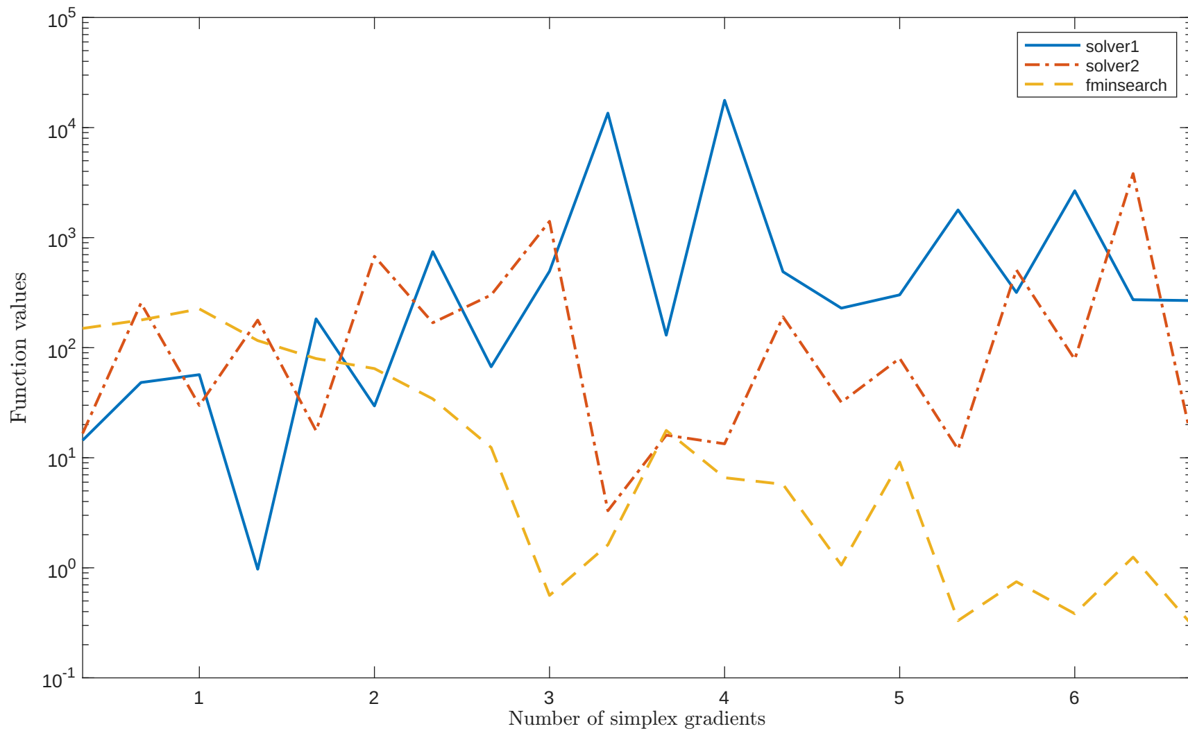
Solving “DANIWOODLS” with “noisy_0.001_mixed_gaussian” feature
