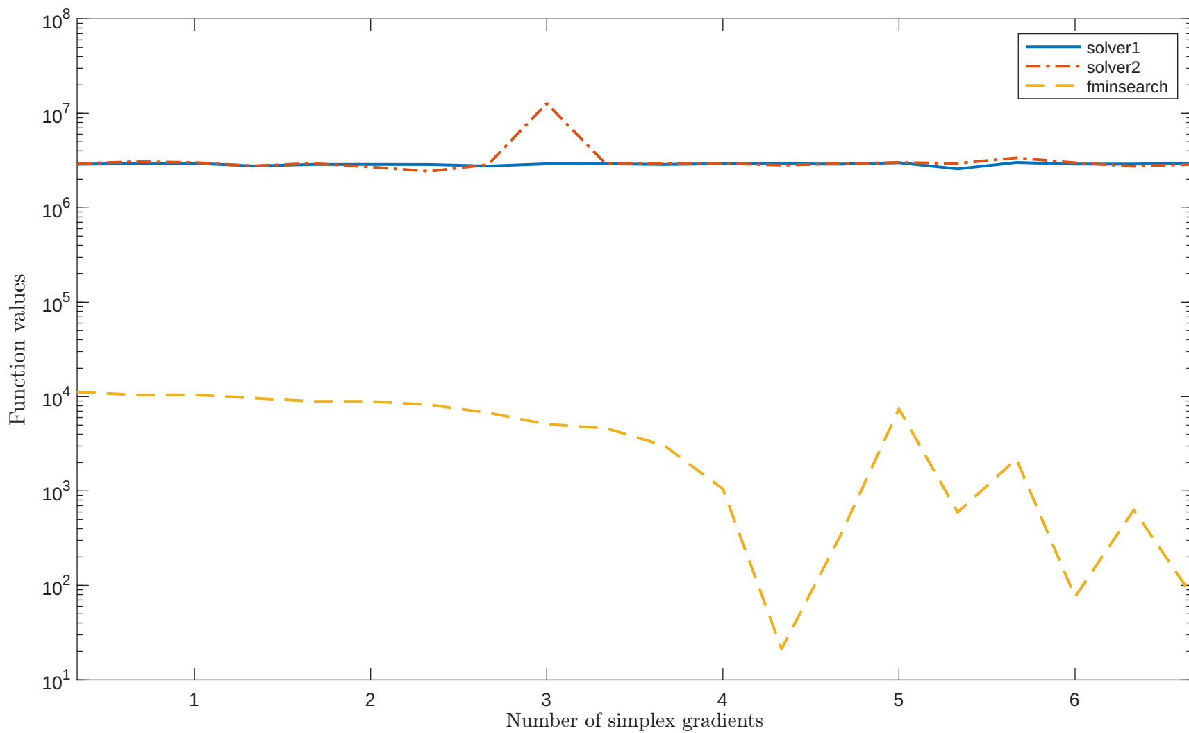
Solving "MISRA1DLS" with "noisy_0.001_mixed_gaussian" feature
