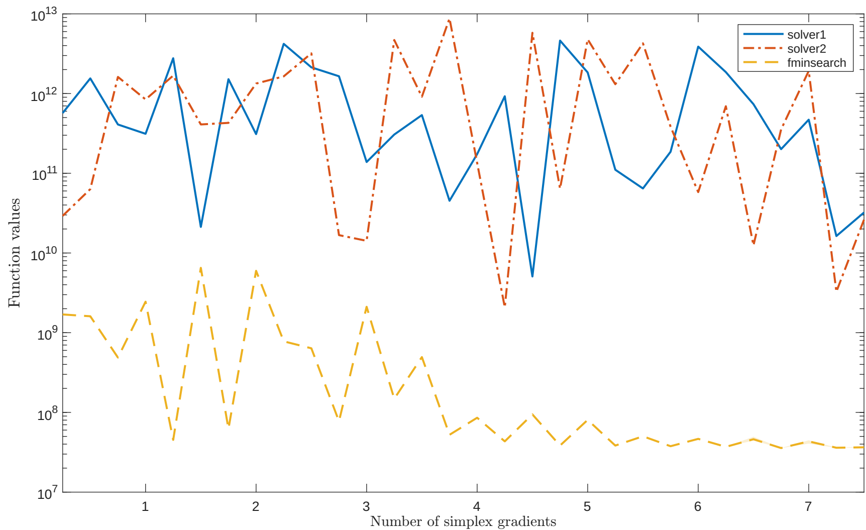
Solving “MEYER3” with “noisy_0.001_mixed_gaussian” feature
