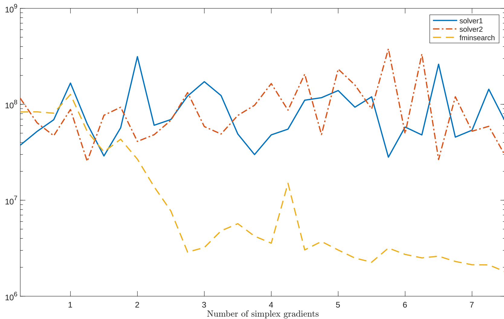
Solving "DENSCHND" with "noisy_0.001_mixed_gaussian" feature
