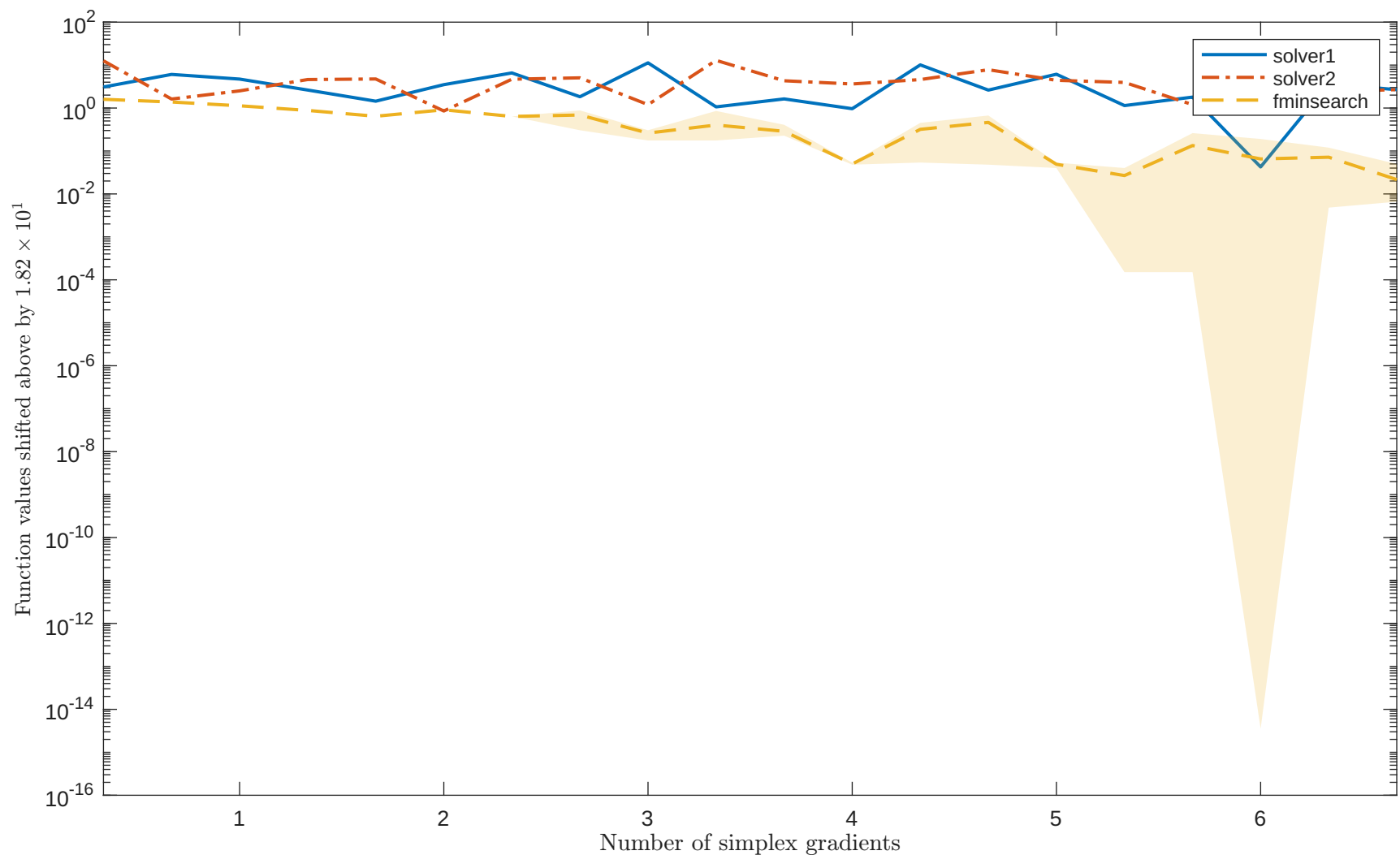
Solving “ZANGWIL2” with “noisy_0.001_mixed_gaussian” feature
