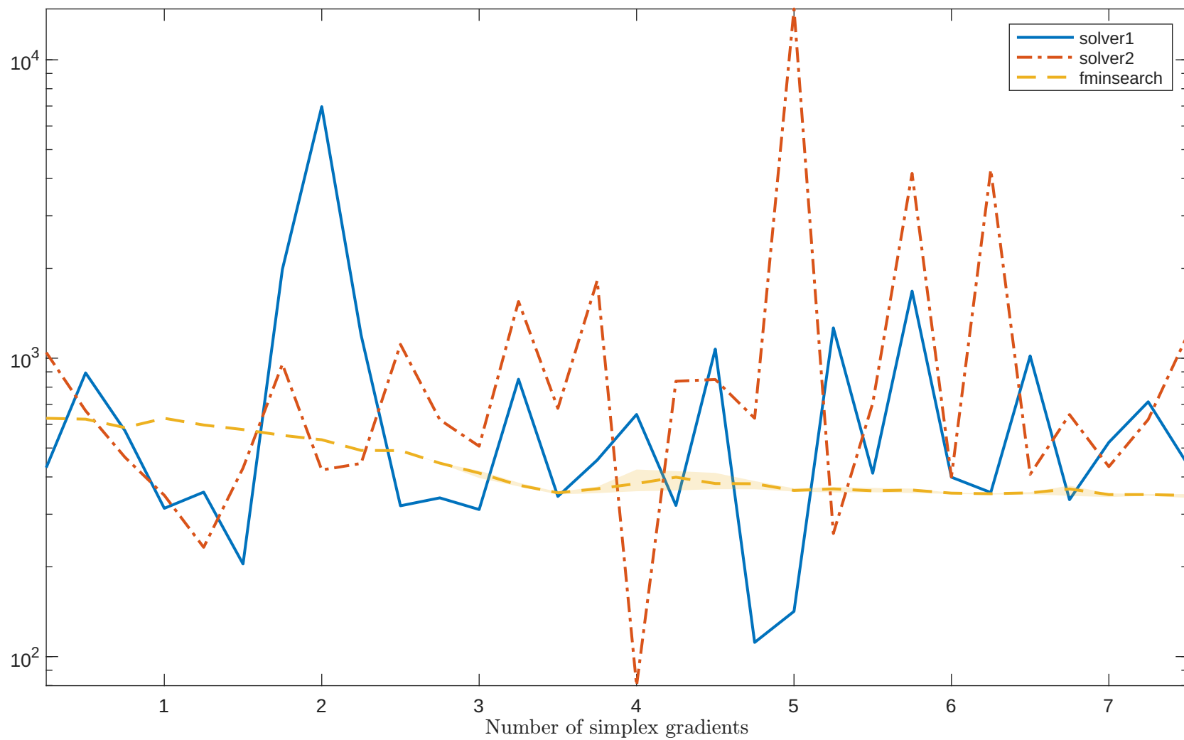
Solving “ENGVAL2” with “noisy_0.001_mixed_gaussian” feature
