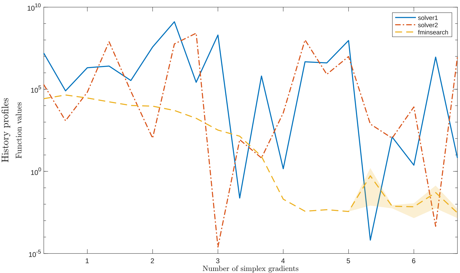
Solving “HIMMELBB” with “noisy_0.001_mixed_gaussian” feature
