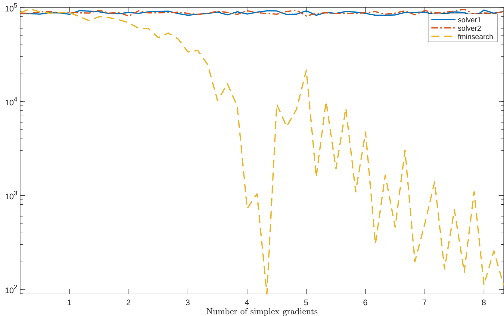
Solving “MGH17SLS” with “noisy_0.001_mixed_gaussian” feature
