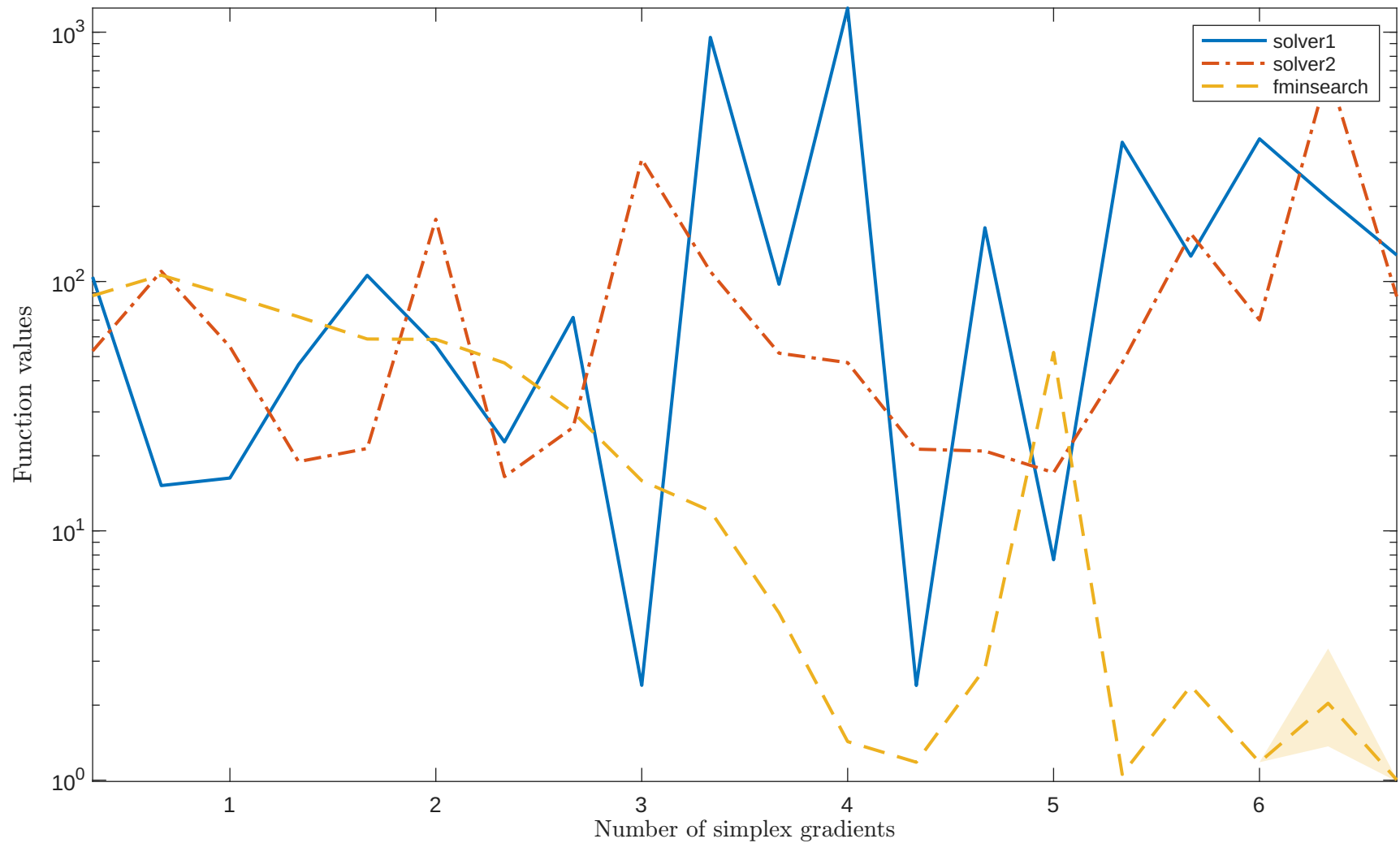
Solving "S308" with "noisy_0.001_mixed-gaussian" feature
