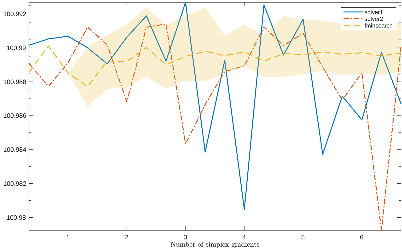
Solving "ROSENBRTU" with "noisy_0.001_mixed-gaussian" feature
