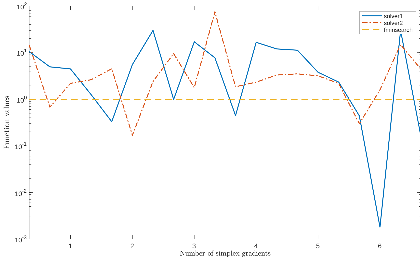
Solving "CLUSTERLS" with "noisy_0.001_mixed_gaussian" feature
