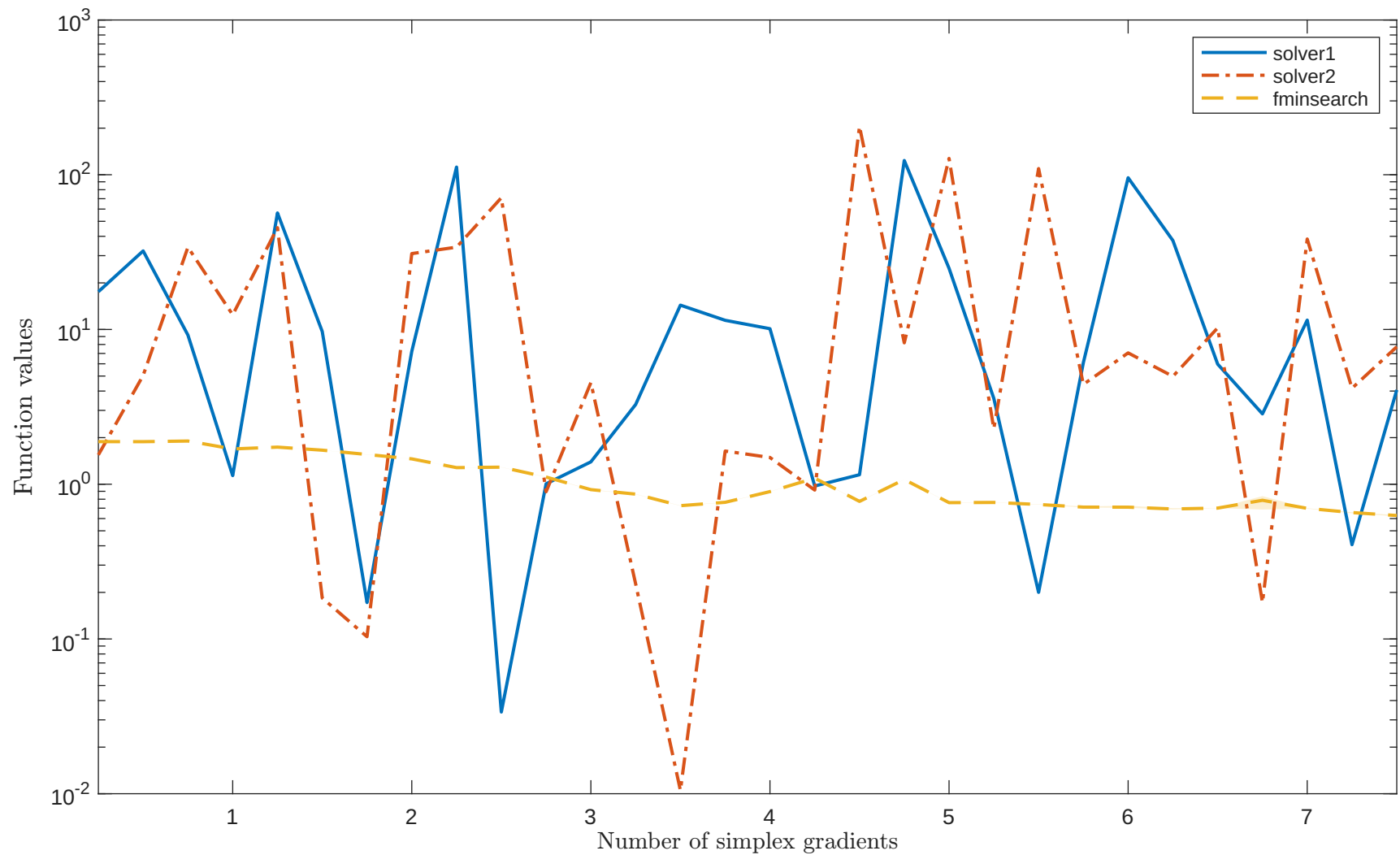
Solving "BOX3" with "noisy_0.001_mixed_gaussian" feature
