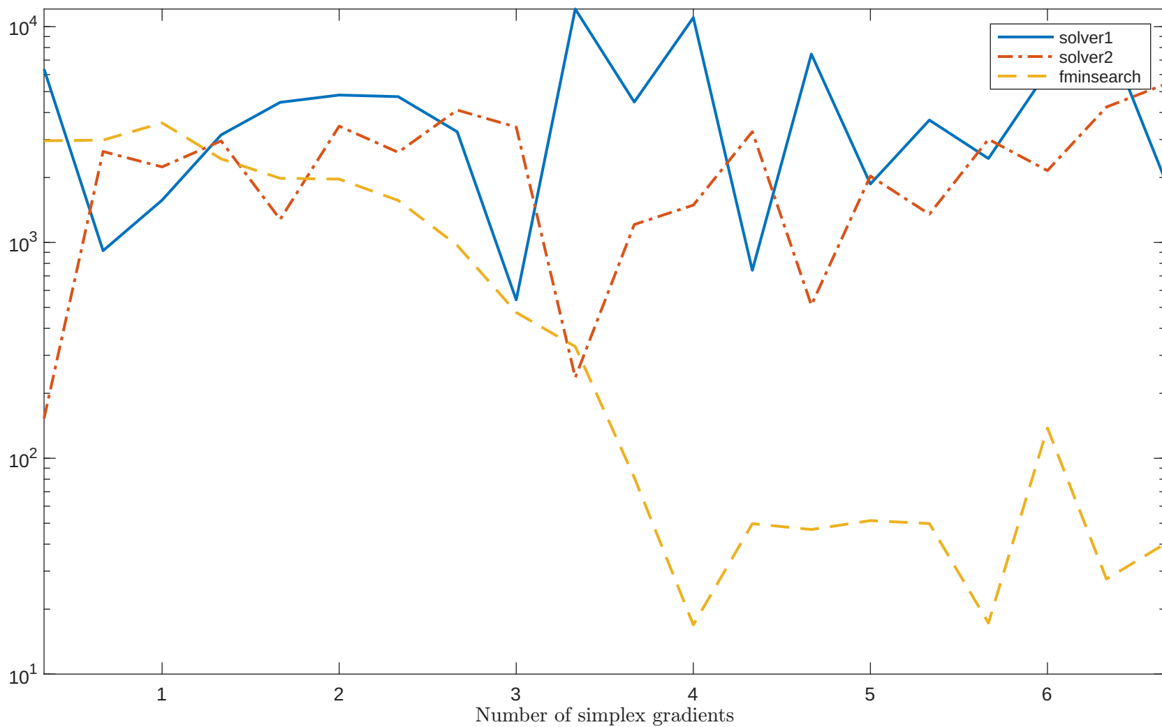
Solving “JUDGE” with “noisy_0.001_mixed_gaussian” feature
