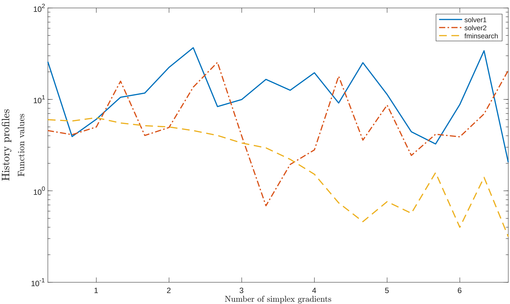
Solving “DENSCHNB” with “noisy_0.001_mixed-gaussian” feature
