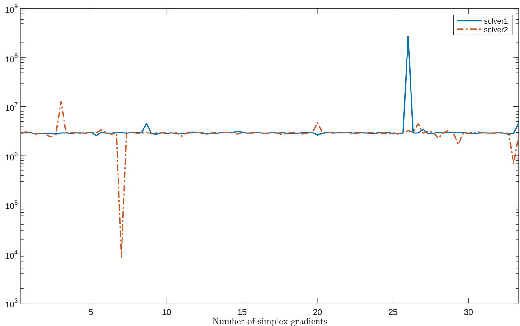
Solving "MISRA1DLS" with "plain" feature
