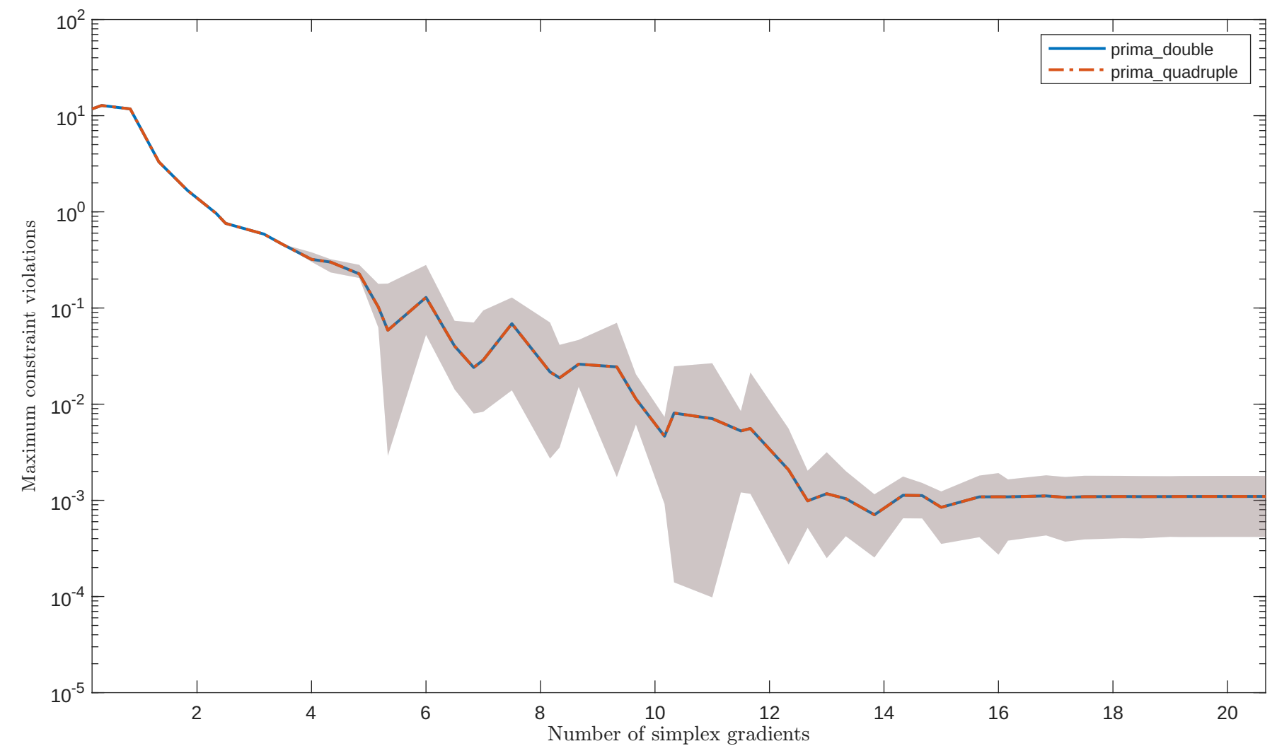
Solving "BT11" with "noisy_0.001-mixed_gaussian" feature
