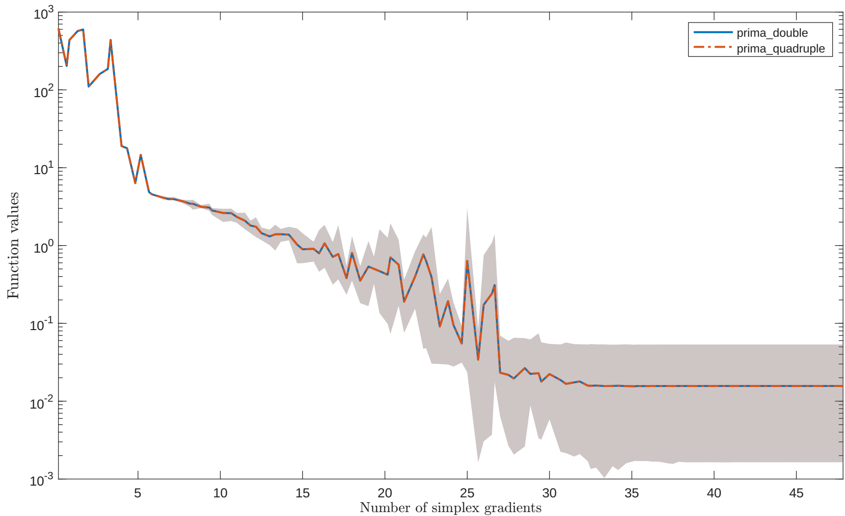
Solving “CHNRSNBM” with “noisy_0.001_mixed-gaussian” feature
