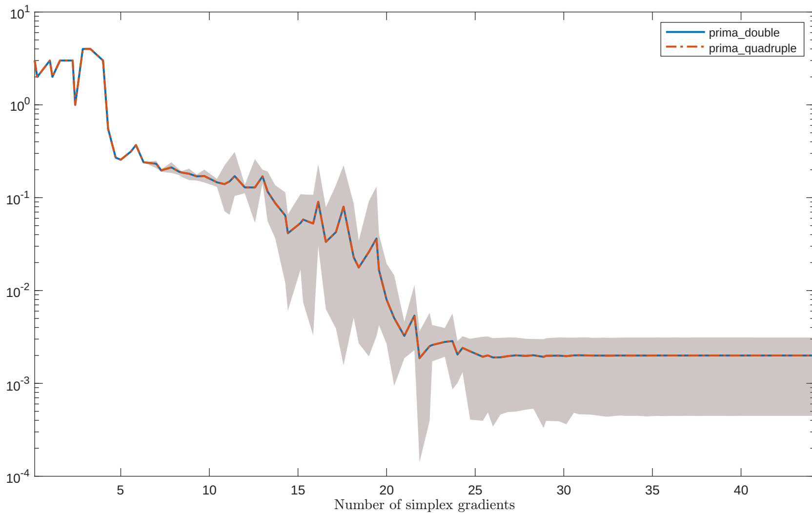
Solving “EIGENBLS” with “noisy_0.001_mixed_gaussian” feature
