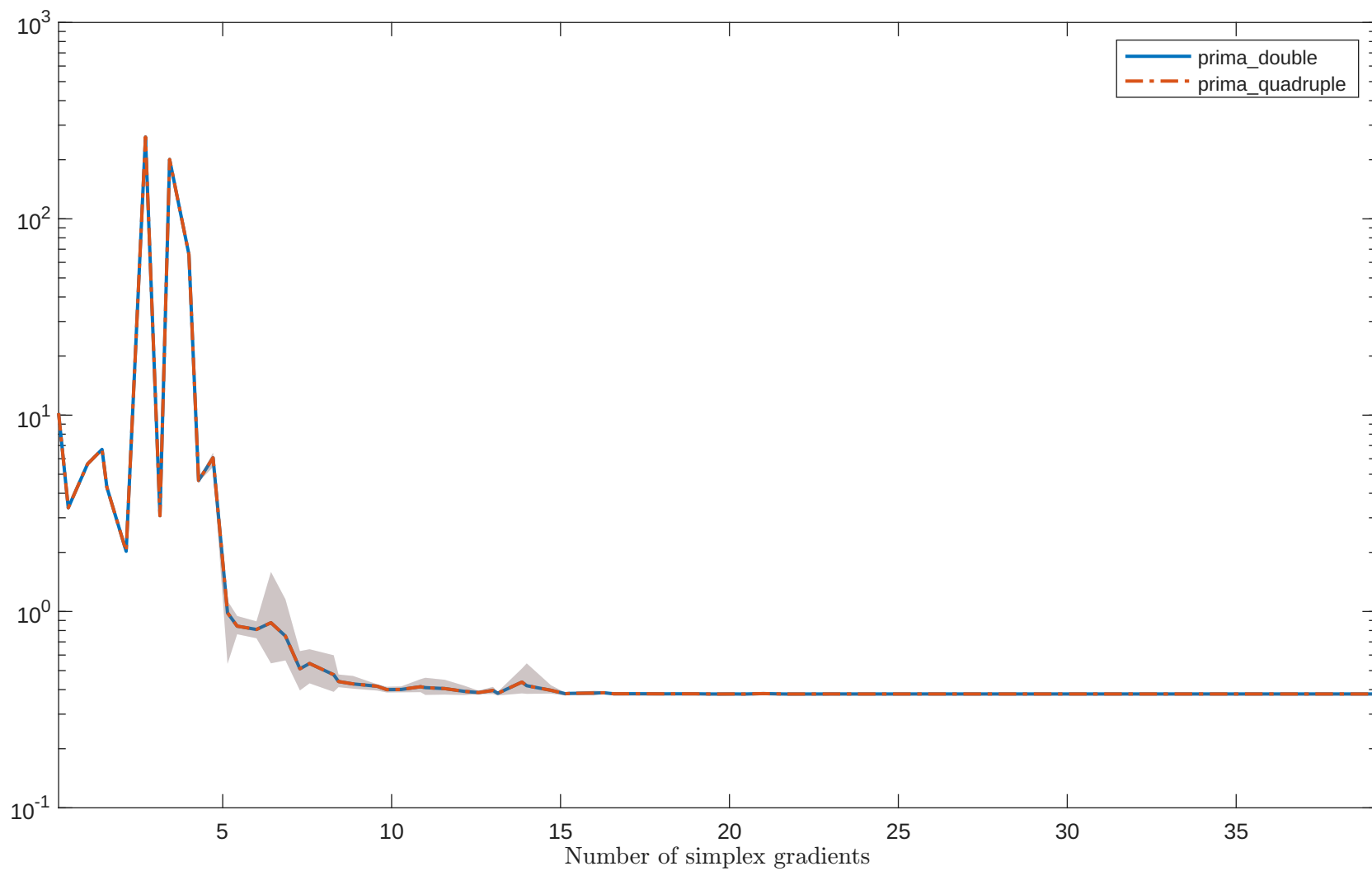
Solving “FBRAIN3LS” with “noisy_0.001_mixed_gaussian” feature
