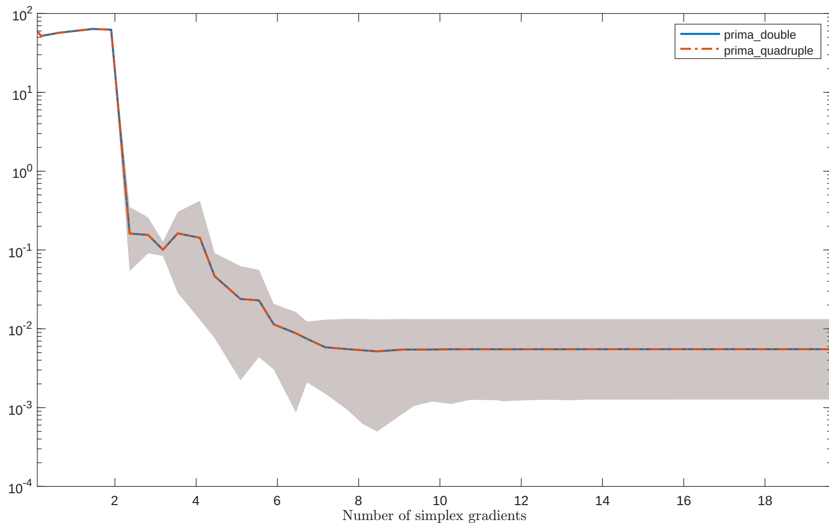
Solving "HILBERTA" with "noisy_0.001_mixed_gaussian" feature
