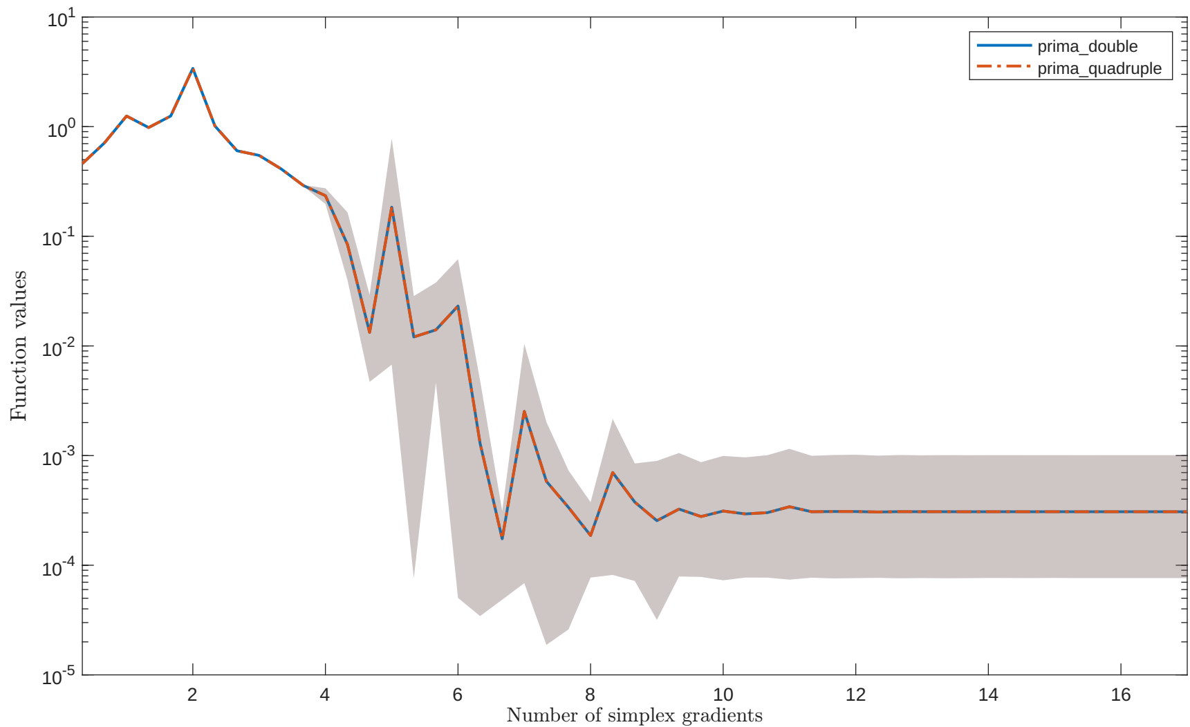
Solving “HIMMELBG” with “noisy_0.001_mixed-gaussian” feature
