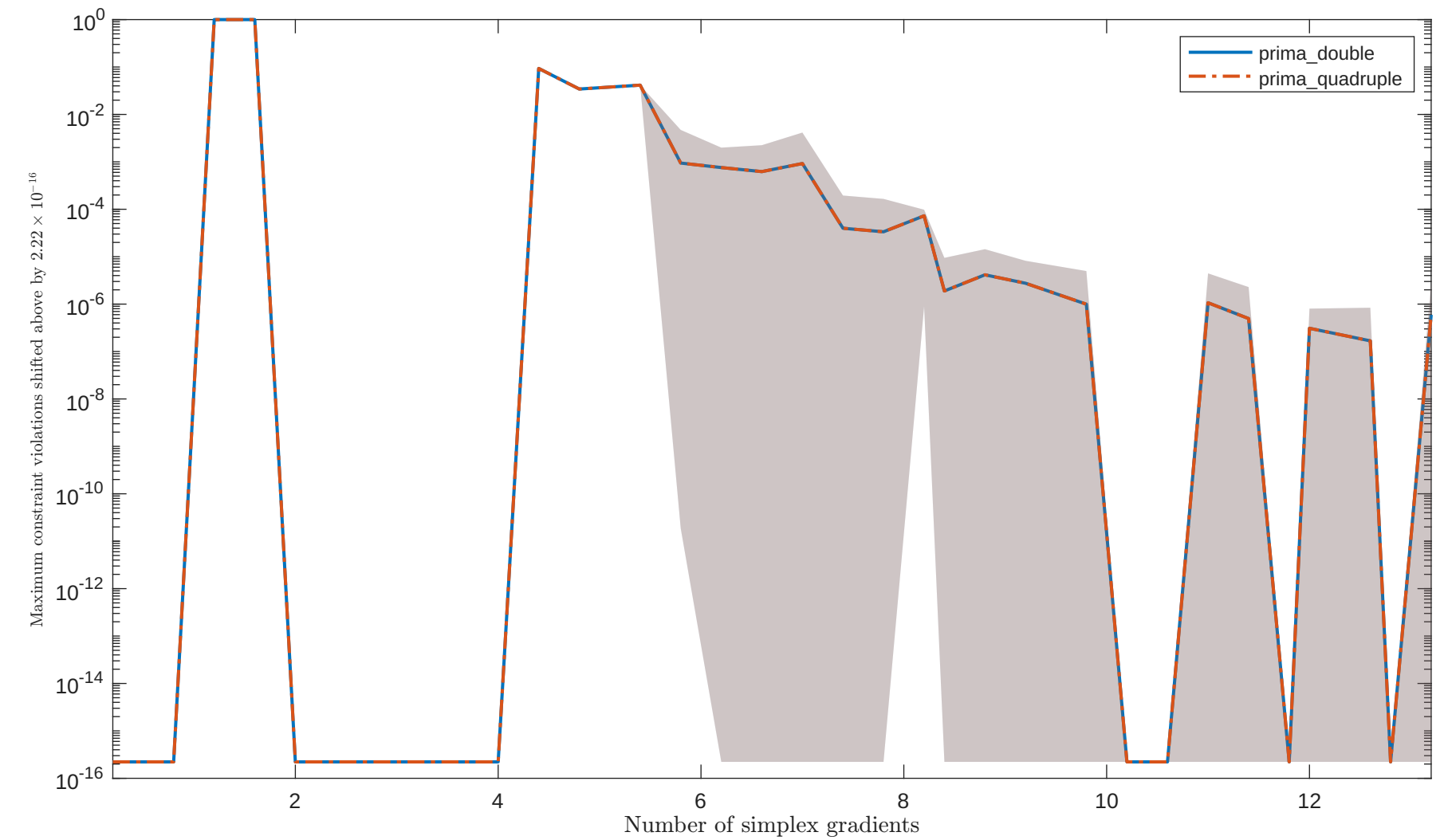
Solving “HS44” with “noisy_0.001_mixed.gaussian” feature
