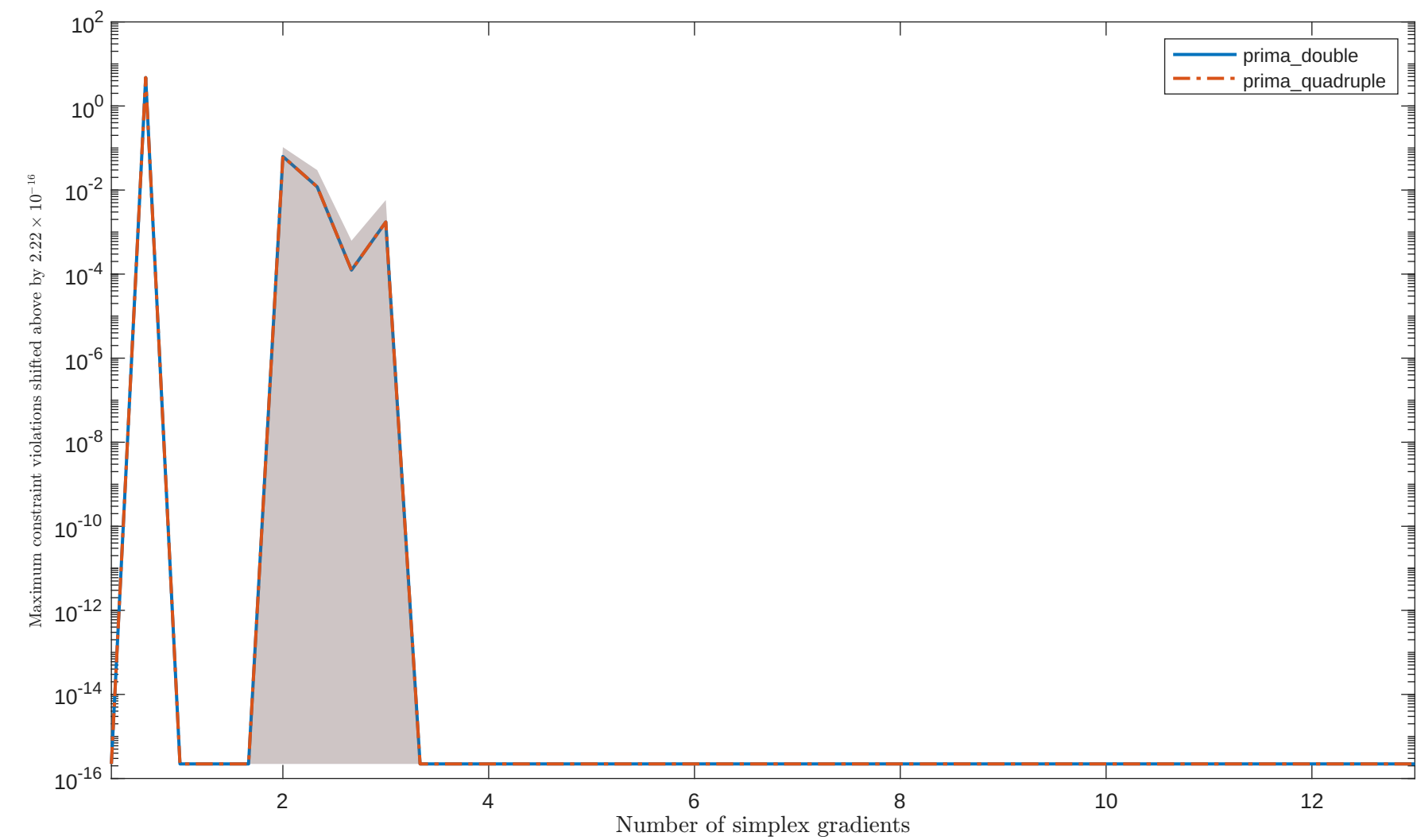
Solving “HS57” with “noisy_0.001_mixed_gaussian” feature
