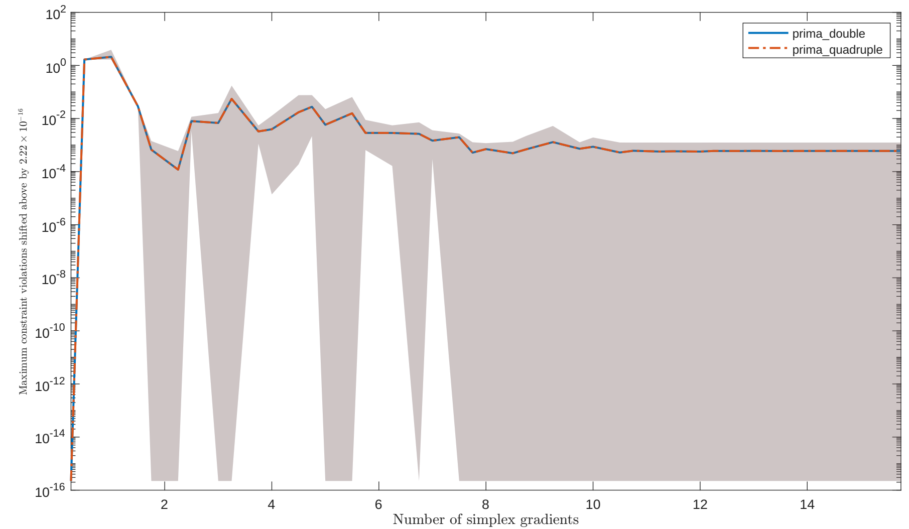
Solving “HS66” with “noisy_0.001_mixed_gaussian” feature
