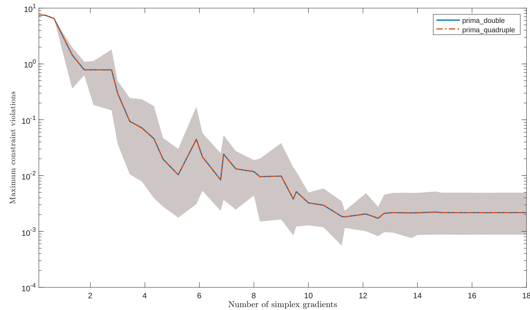
Solving "LUKVLE11" with "noisy_0.001_mixed_gaussian" feature
