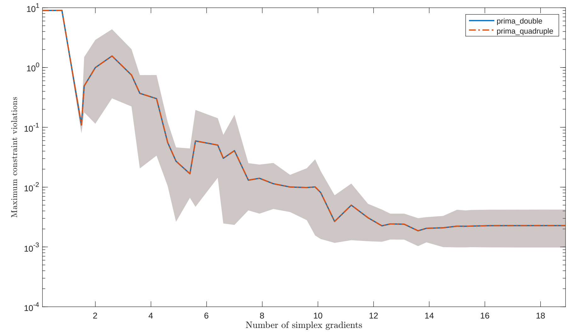
Solving "LUKVLE6" with "noisy_0.001_mixed_gaussian" feature
