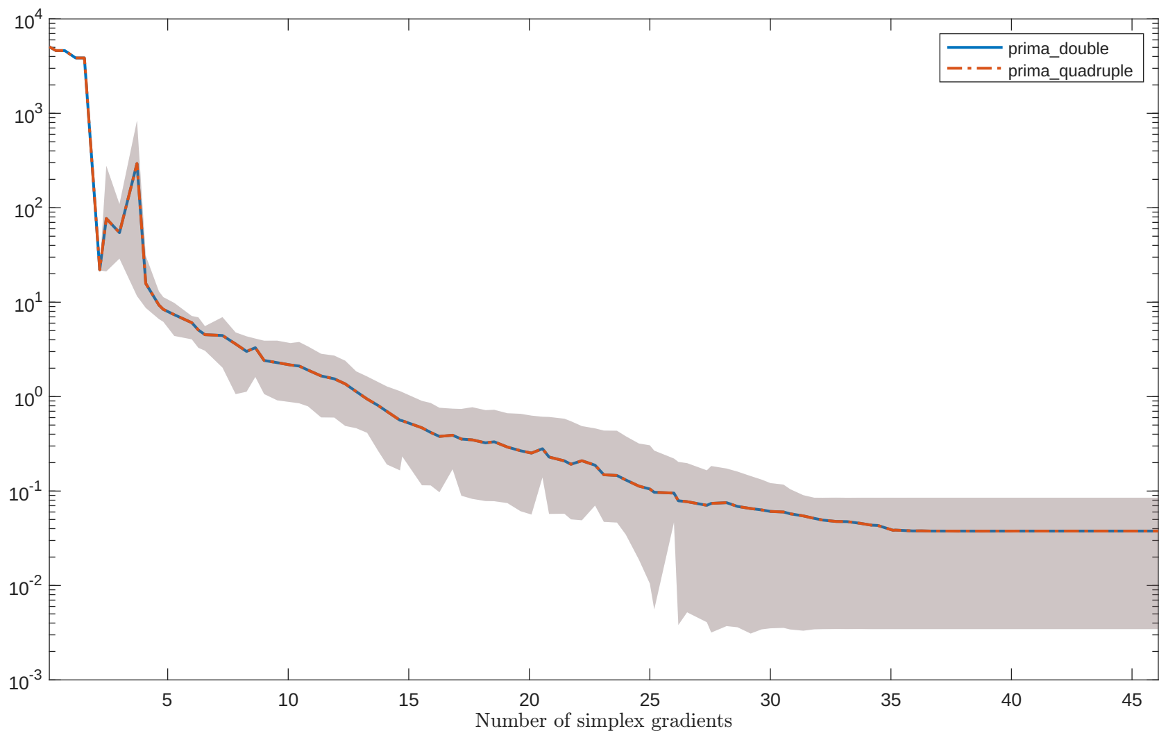
Solving “MODBEALE” with “noisy_0.001_mixed_gaussian” feature
