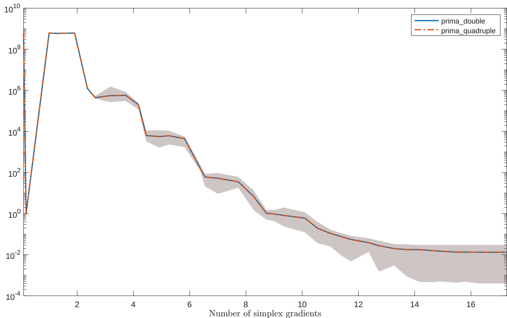
Solving “OSCIGRAD” with “noisy_0.001_mixed_gaussian” feature
