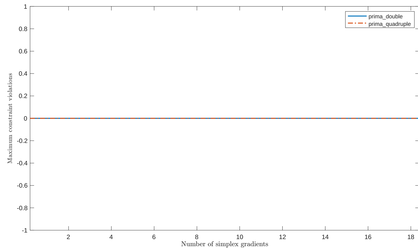
Solving "PALMER1" with "noisy_0.001_mixed_gaussian" feature
