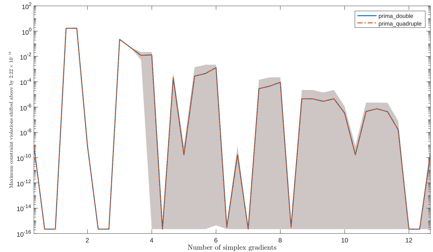
Solving "SIMPLLPB" with "noisy_0.001_mixed.gaussian" feature
