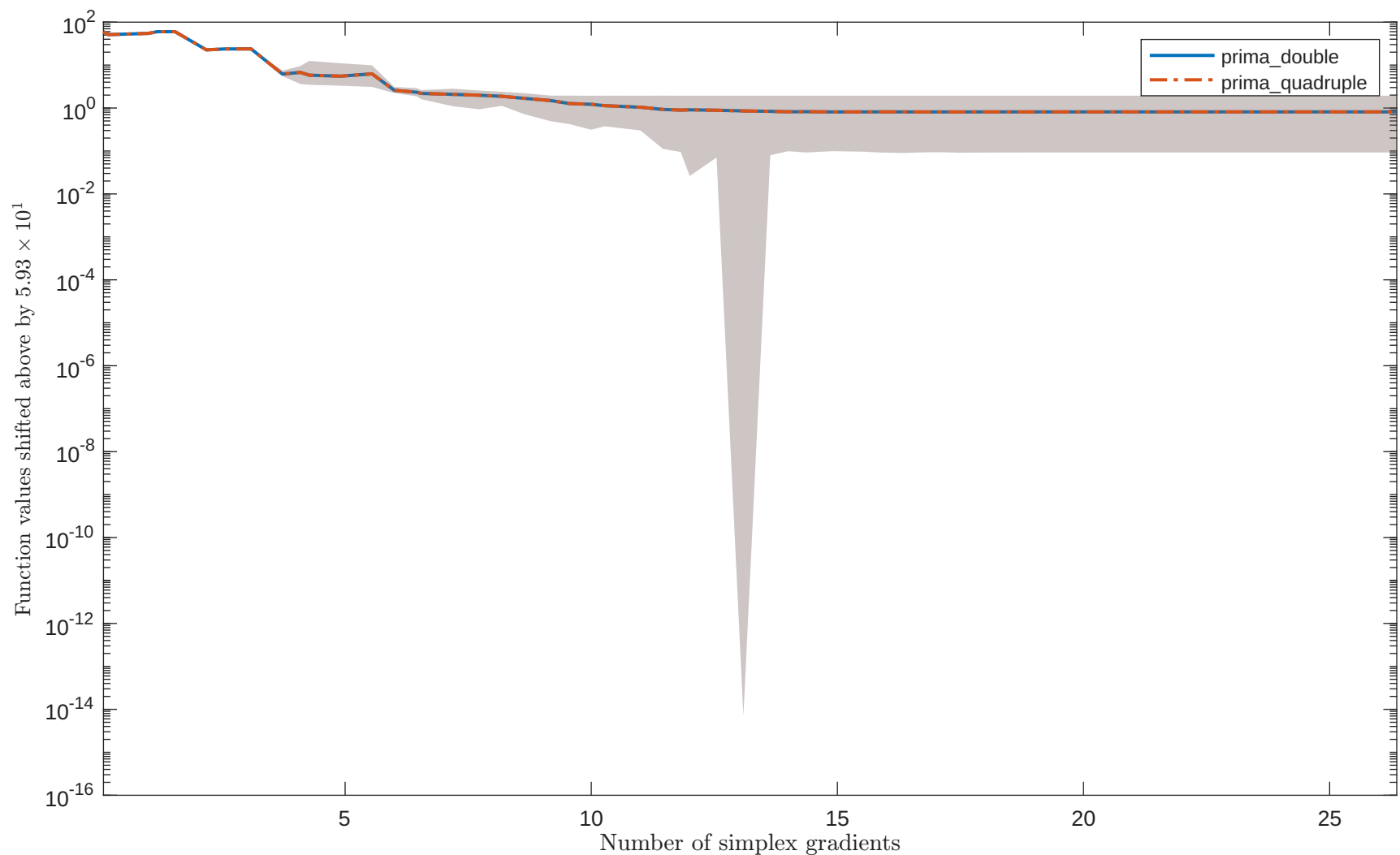
Solving "SINQUAD" with "noisy_0.001_mixed_gaussian" feature
