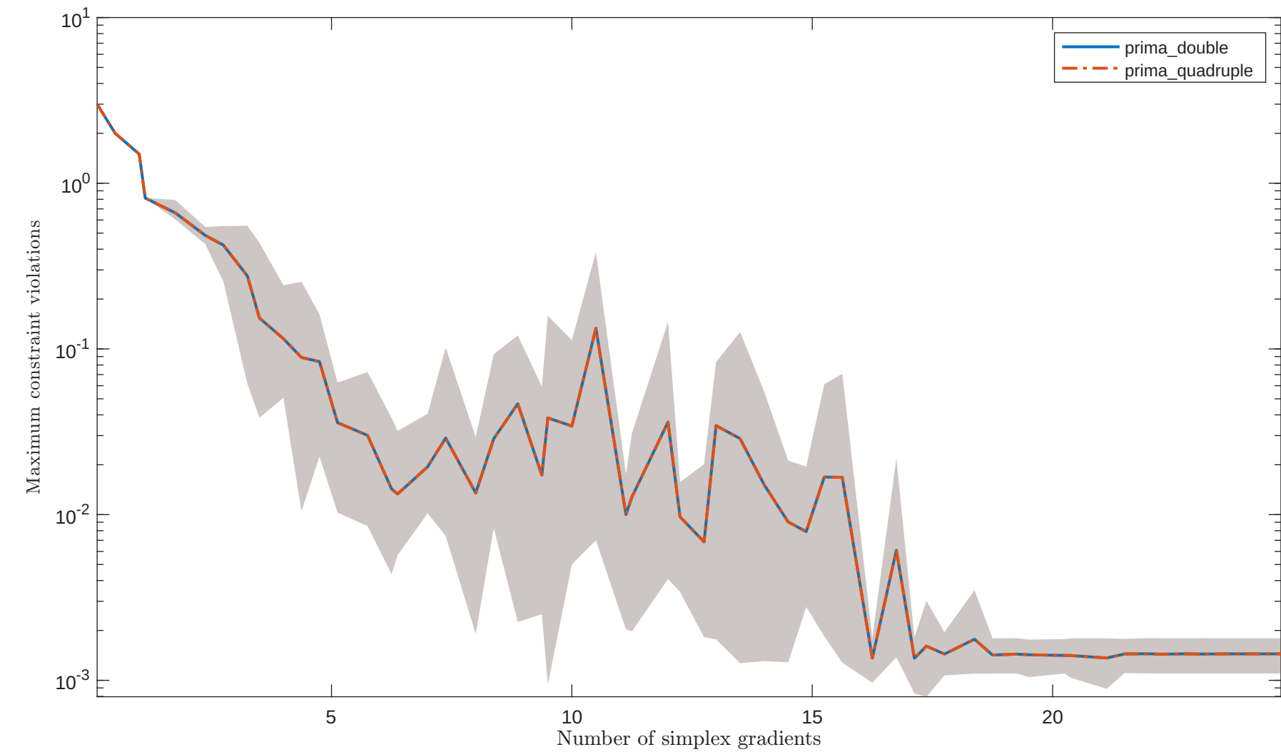
Solving “SPINOP” with “noisy_0.001_mixed_gaussian” feature
