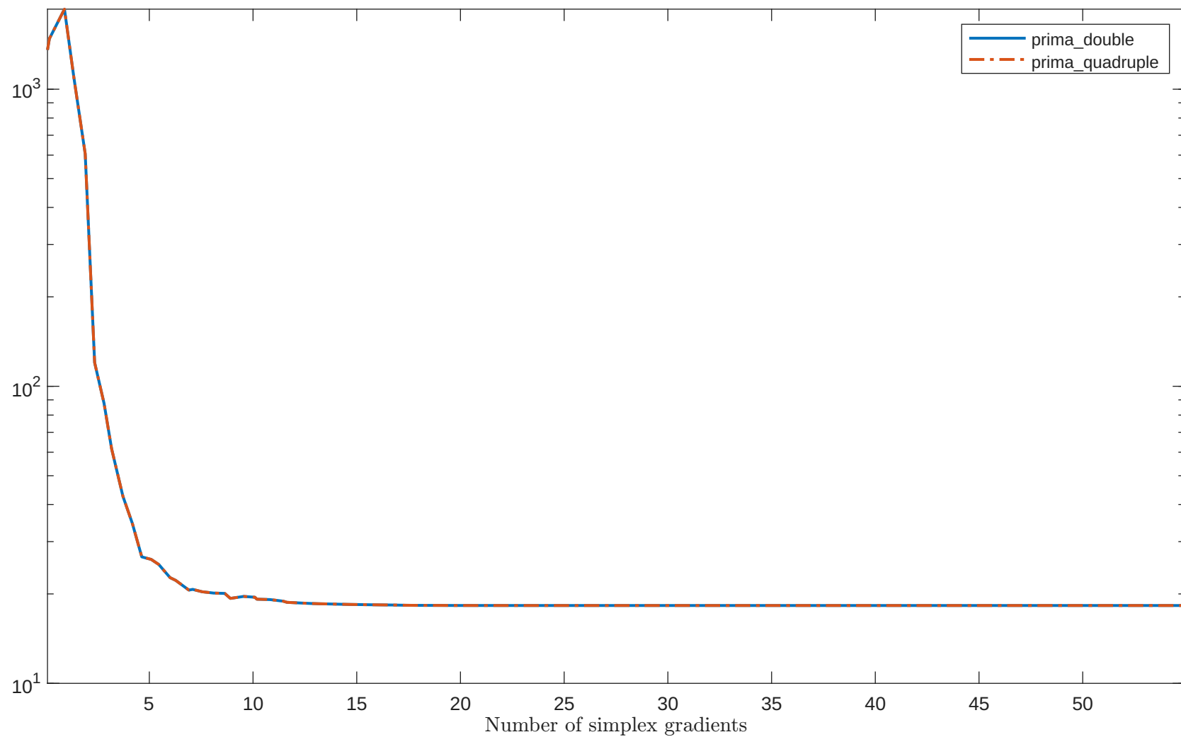
Solving “BDQRTIC” with “plain” feature
