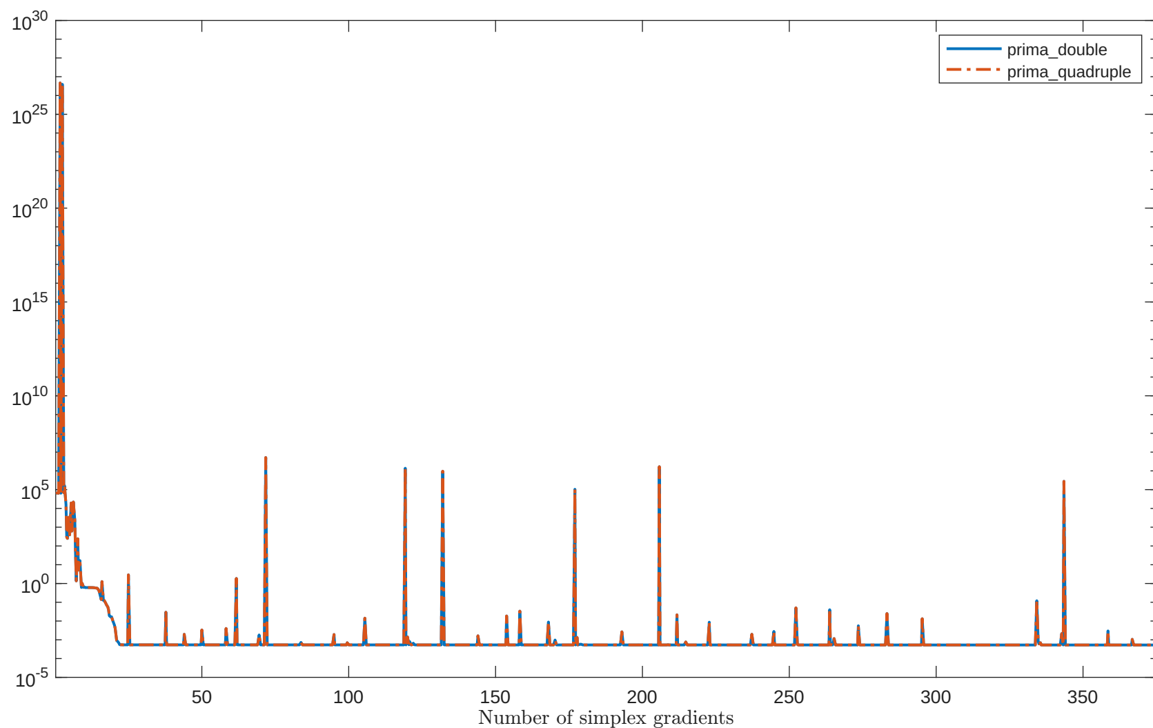
Solving "BENNETT5LS" with "plain" feature
