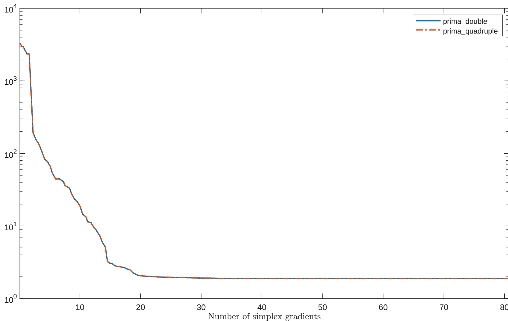
Solving "CRAGGLVY" with "plain" feature
