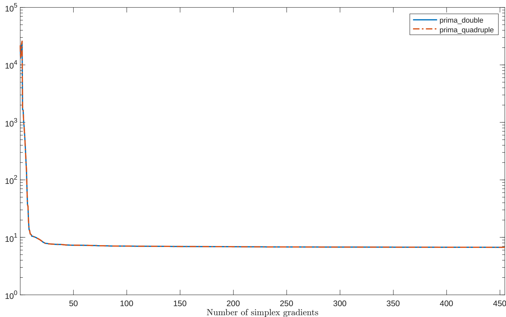
Solving "ERRINROS" with "plain" feature
