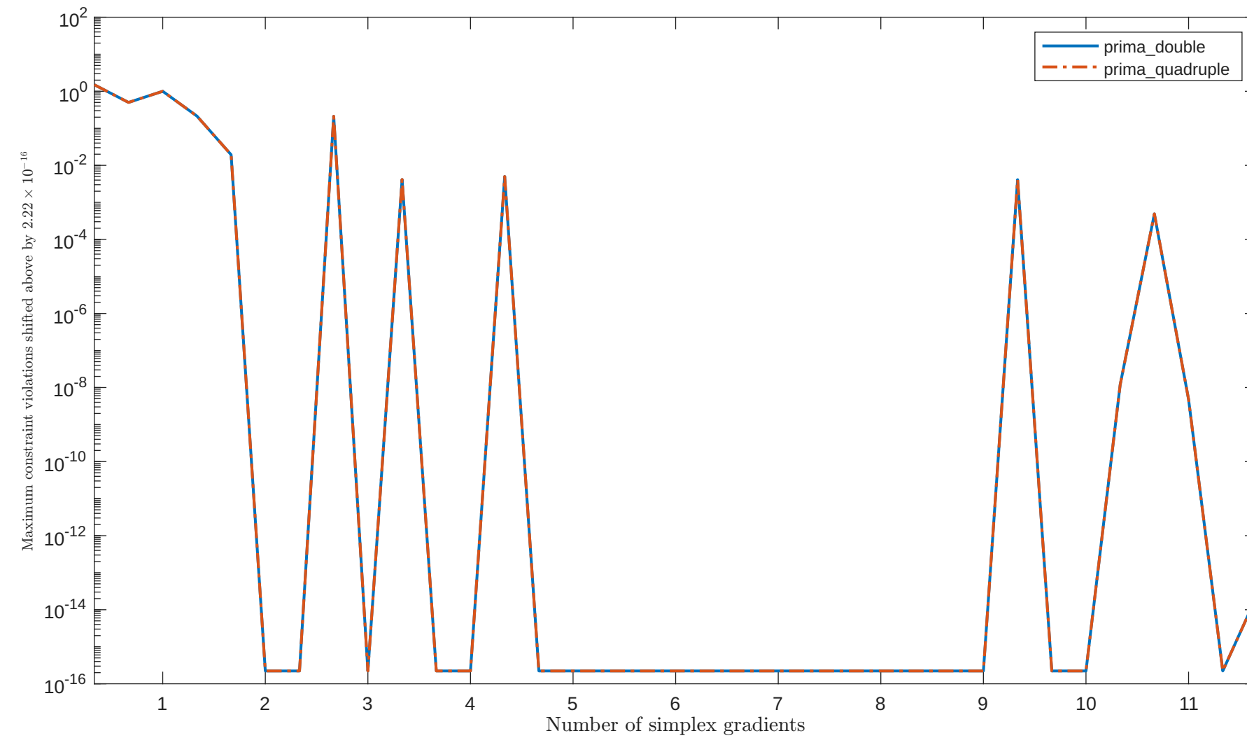
Solving "HS17" with "plain" feature
