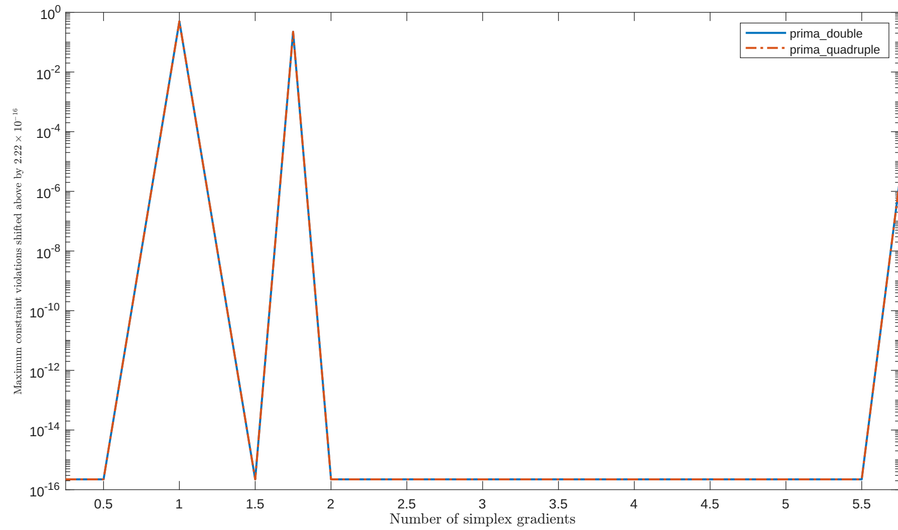
Solving “HS35MOD” with “plain” feature
