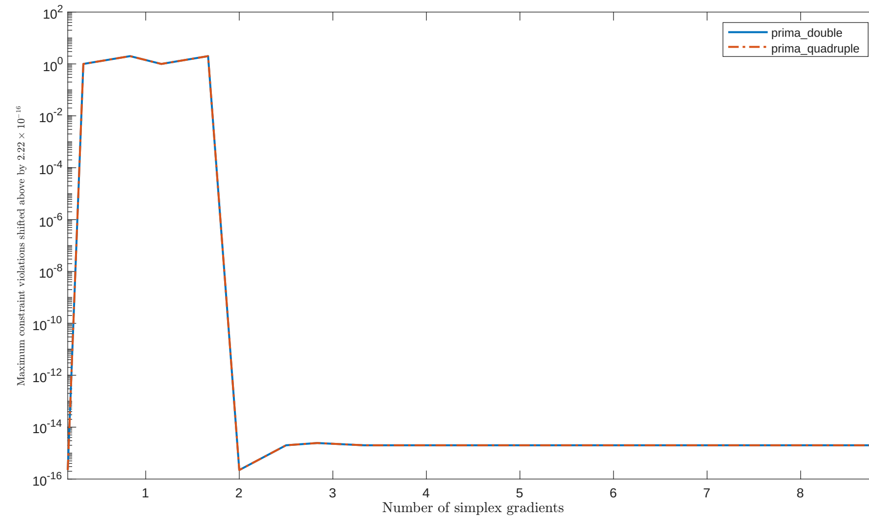
Solving "HS48" with "plain" feature
