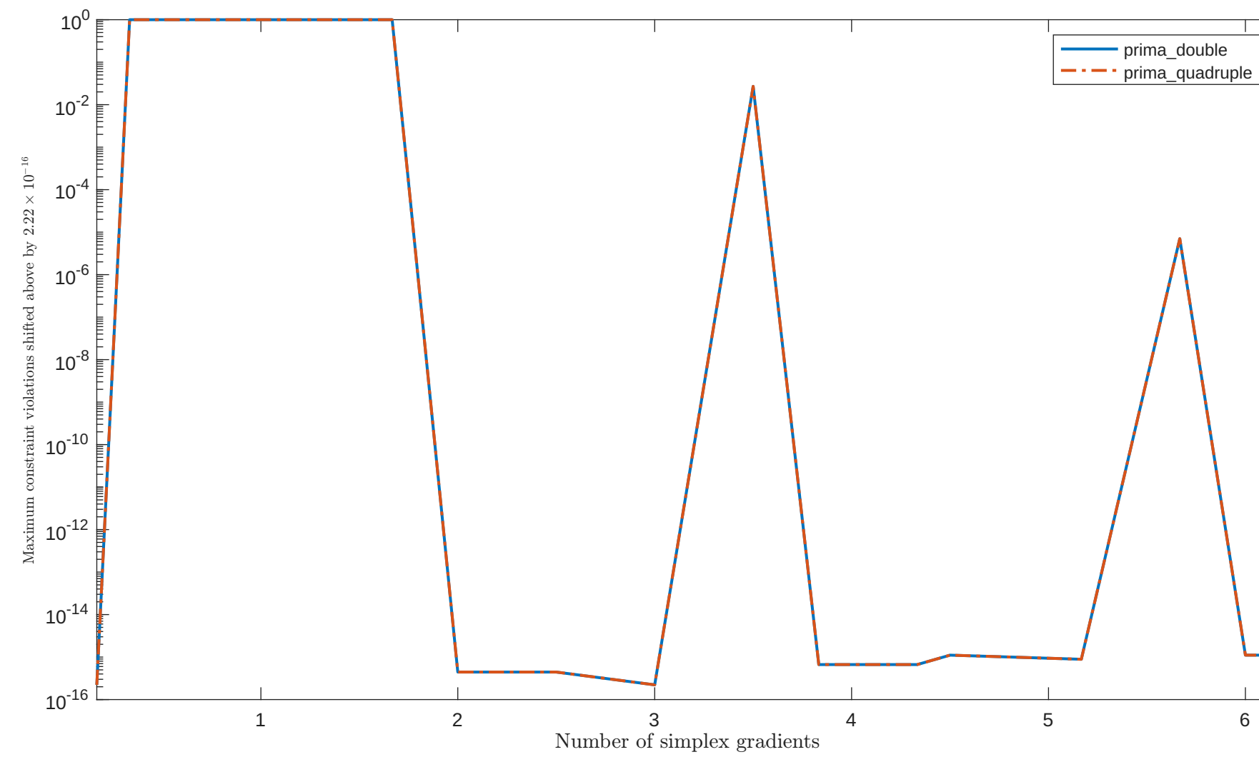
Solving "HS51" with "plain" feature
