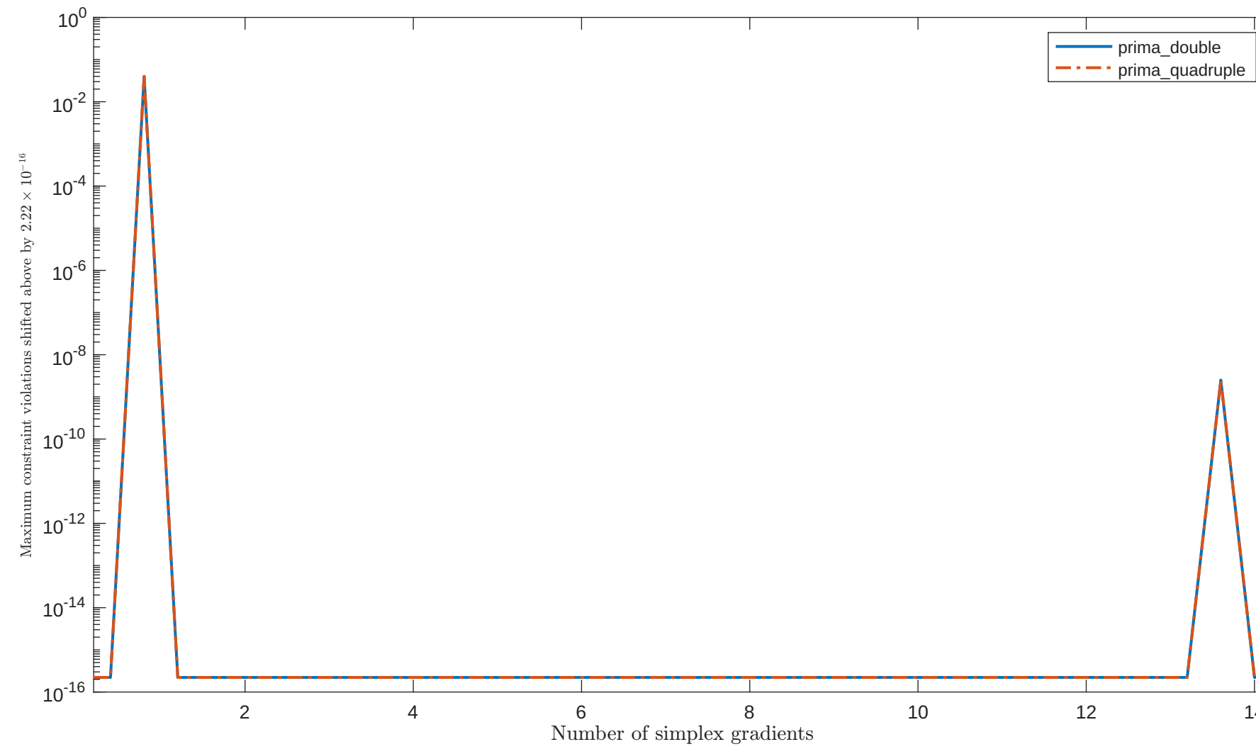
Solving “HS70” with “plain” feature
