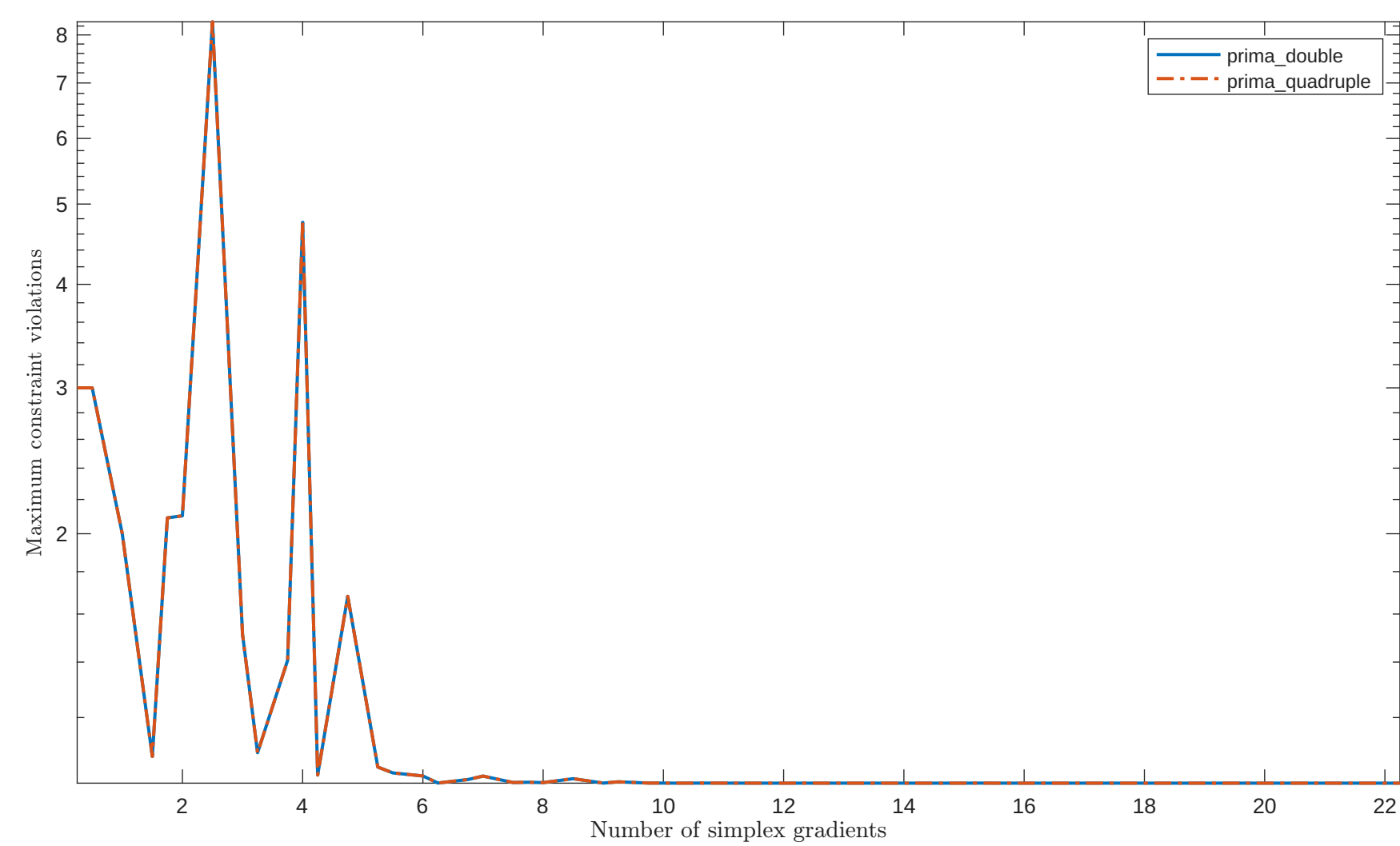
Solving "LOOTSMA" with "plain" feature
