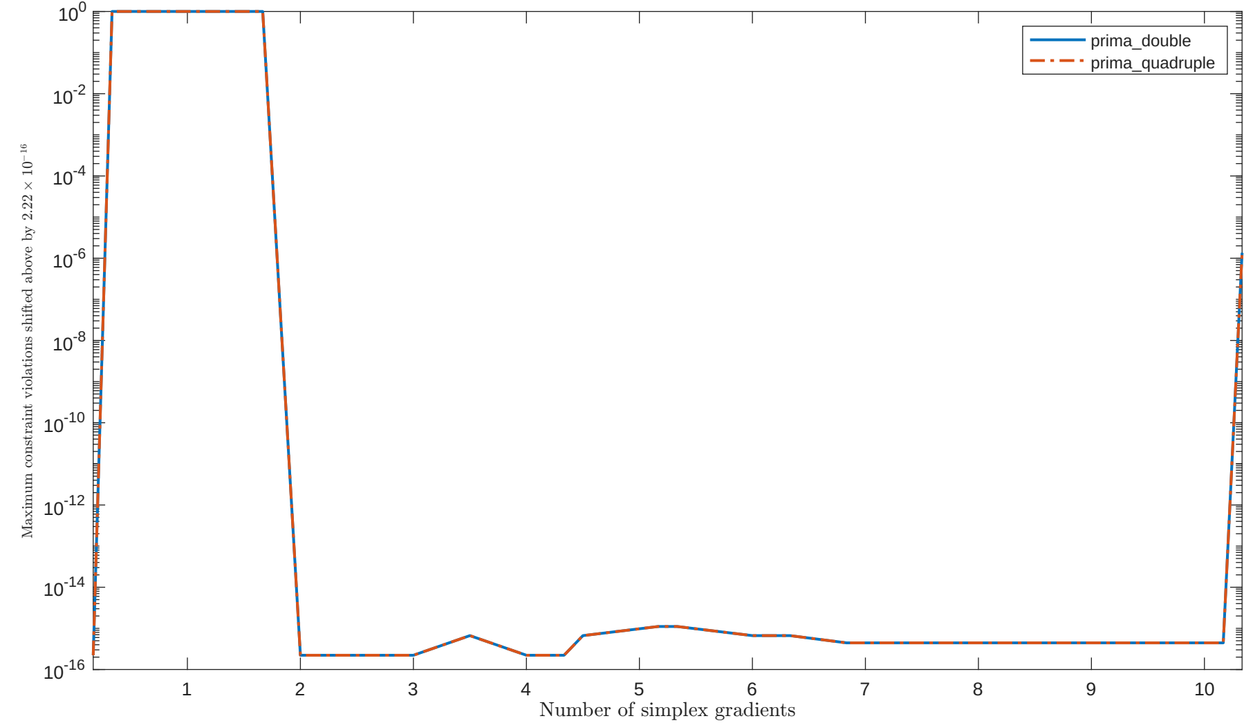
Solving “LSNNODOC” with “plain” feature
