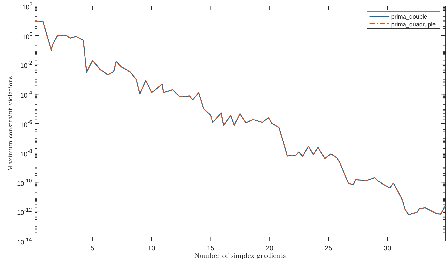
Solving "LUKVLE6" with "plain" feature
