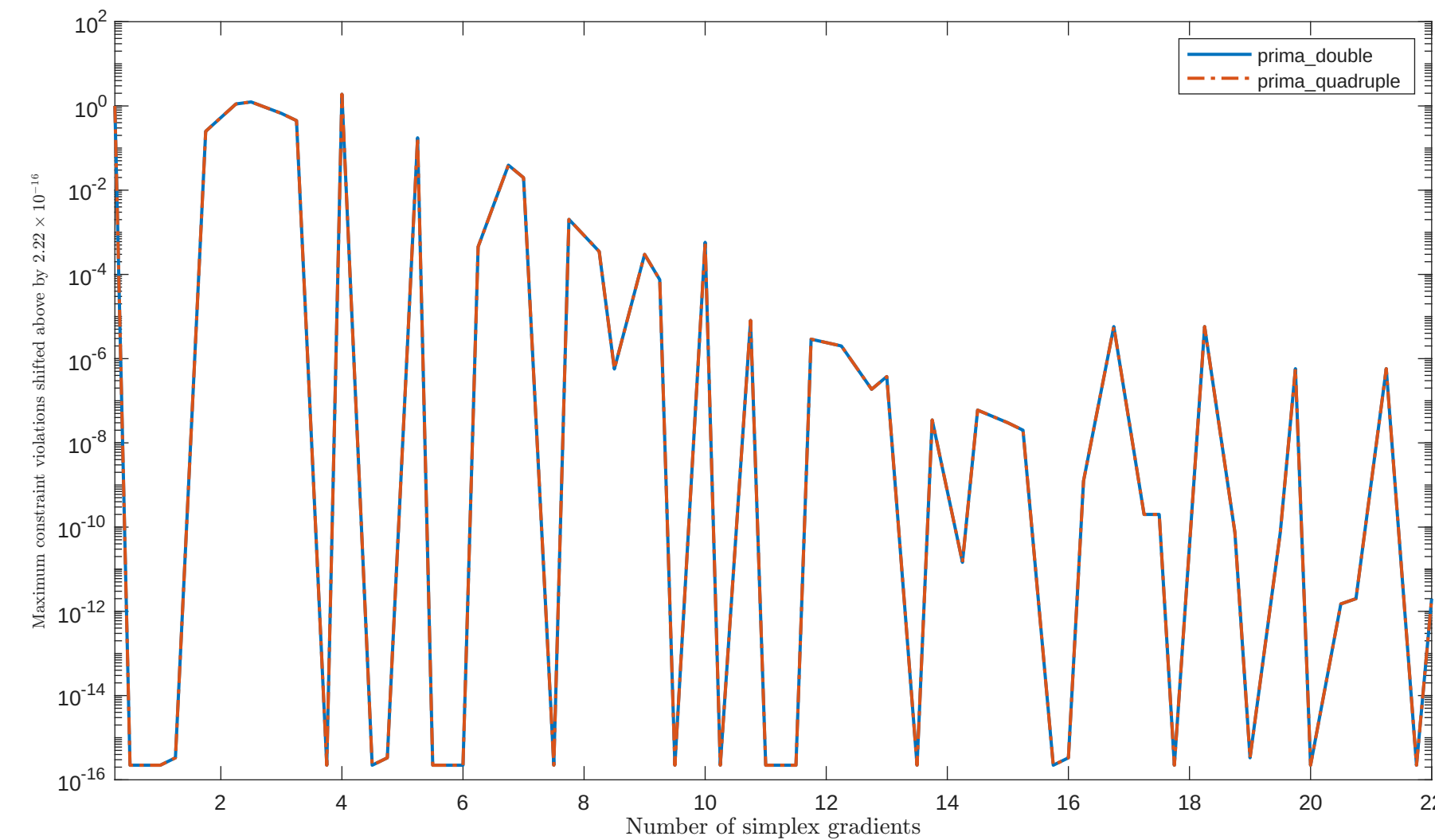
Solving "MAKELA1" with "plain" feature
