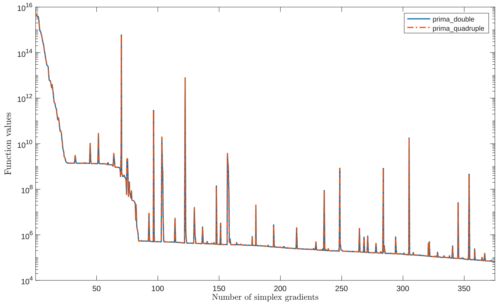
Solving “MGH10SLS” with “plain” feature
