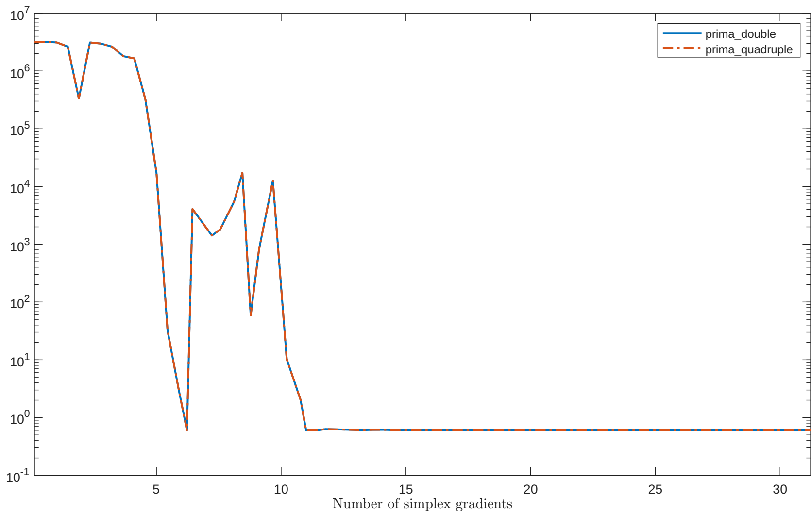
Solving "PALMER7C" with "plain" feature
