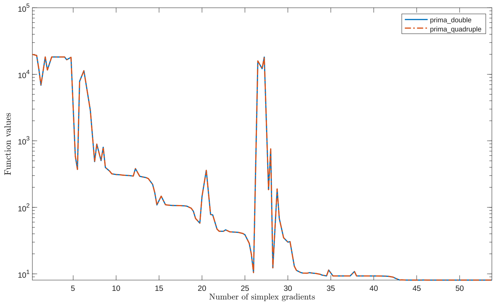
Solving "RAT42LS" with "plain" feature
