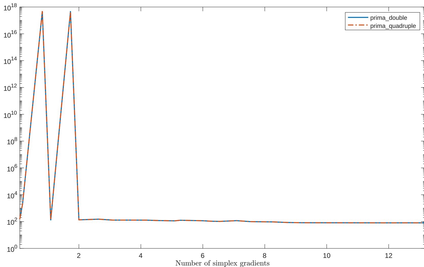
Solving “SBRYBND” with “plain” feature
