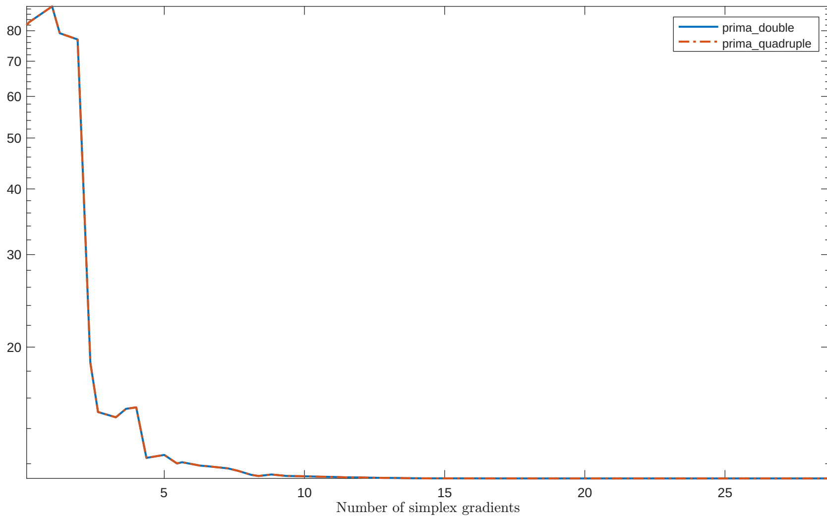
Solving "TOINTGSS" with "plain" feature
