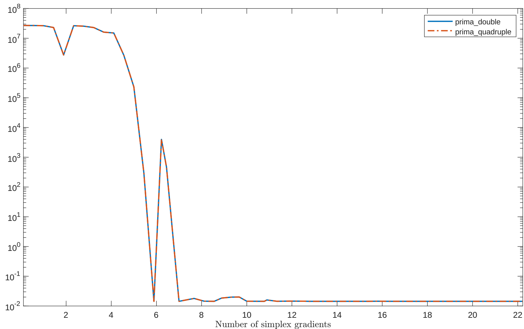
Solving "PALMER2C" with "plain" feature
