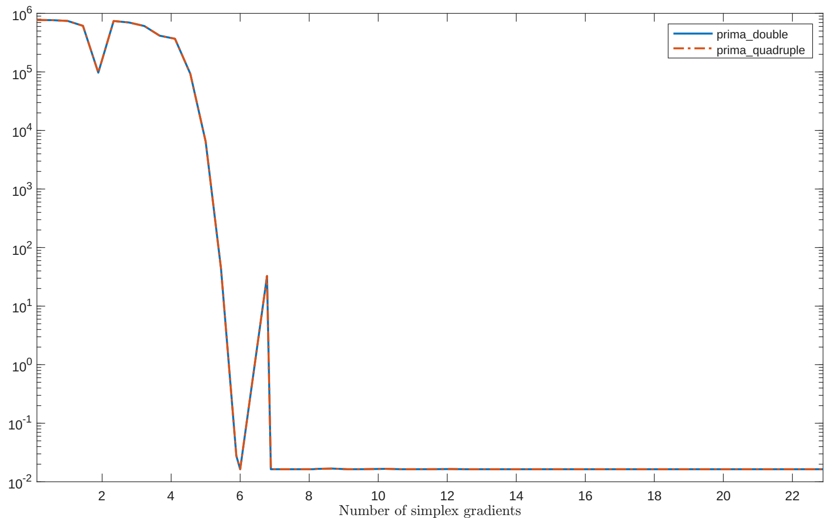
Solving "PALMER6C" with "plain" feature
