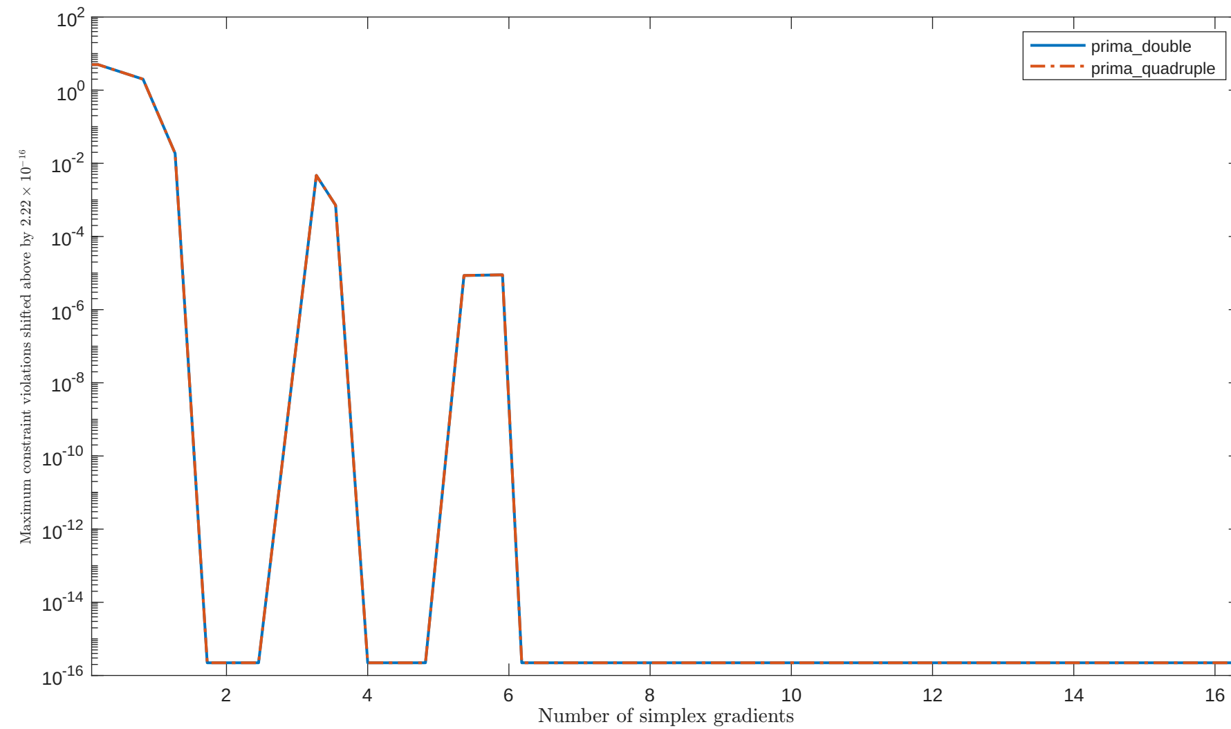
Solving "LUKVL10" with "plain" feature
