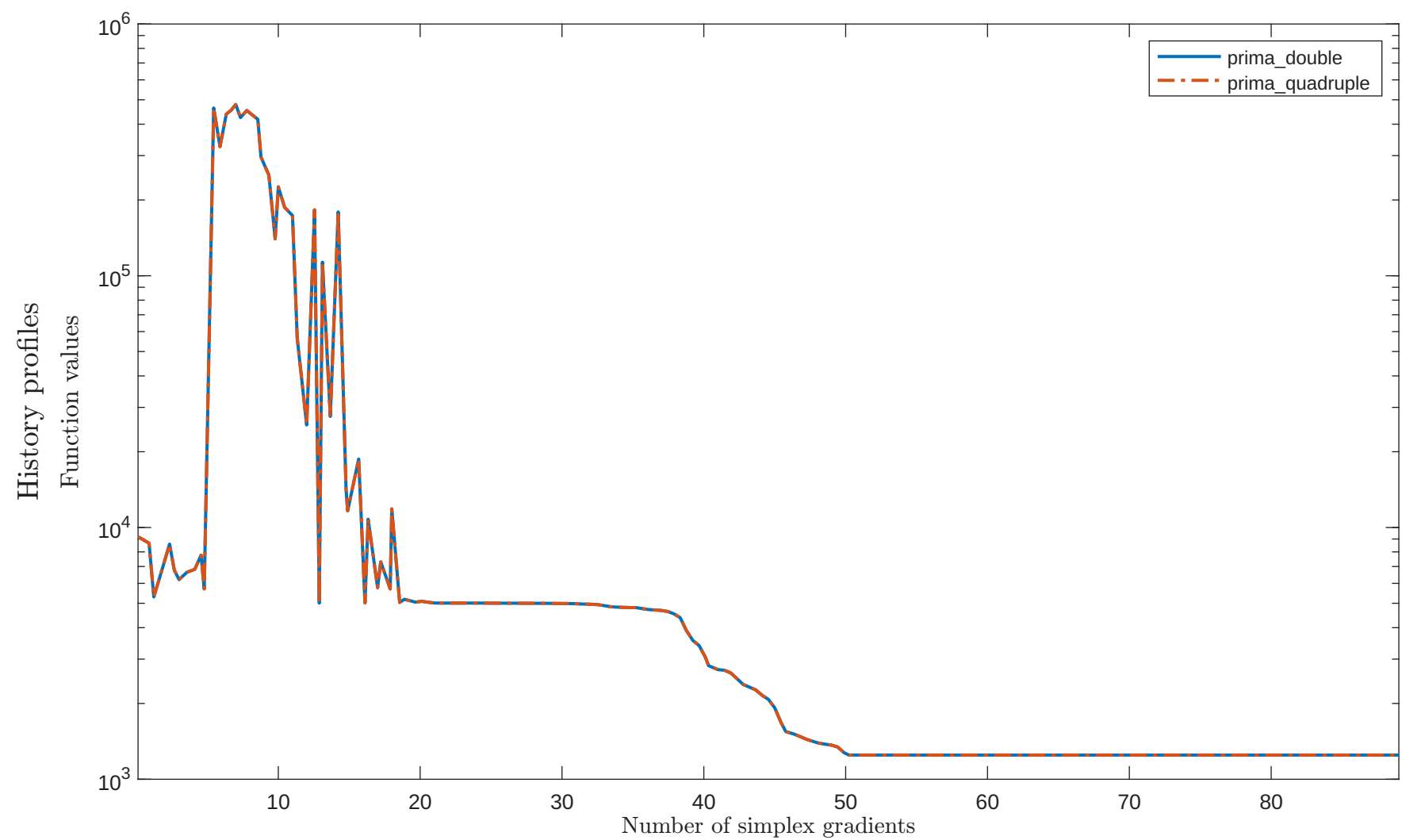
Solving “GAUSS2LS” with “plain” feature
