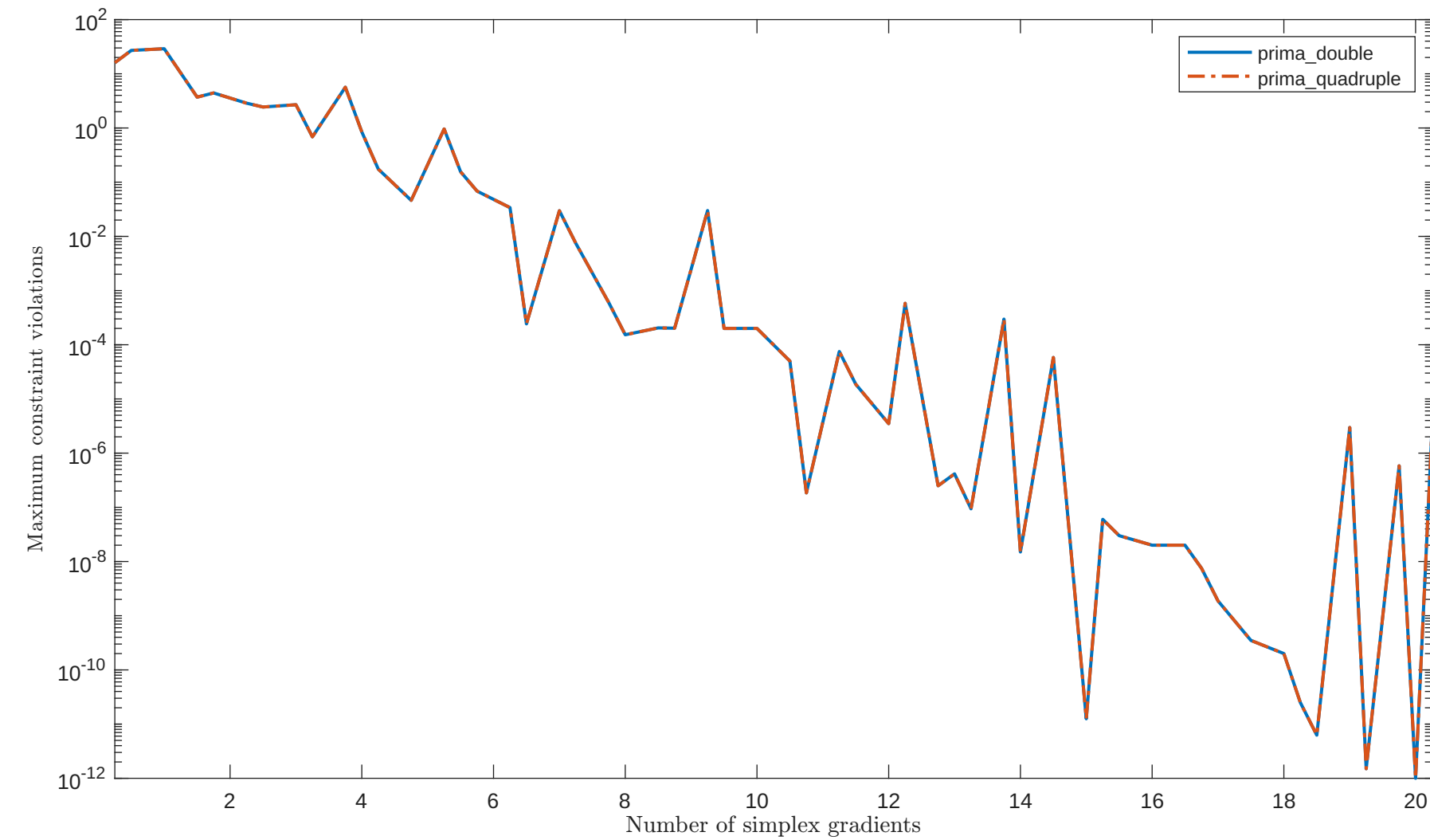
Solving "BYRDSPHR" with "plain" feature
