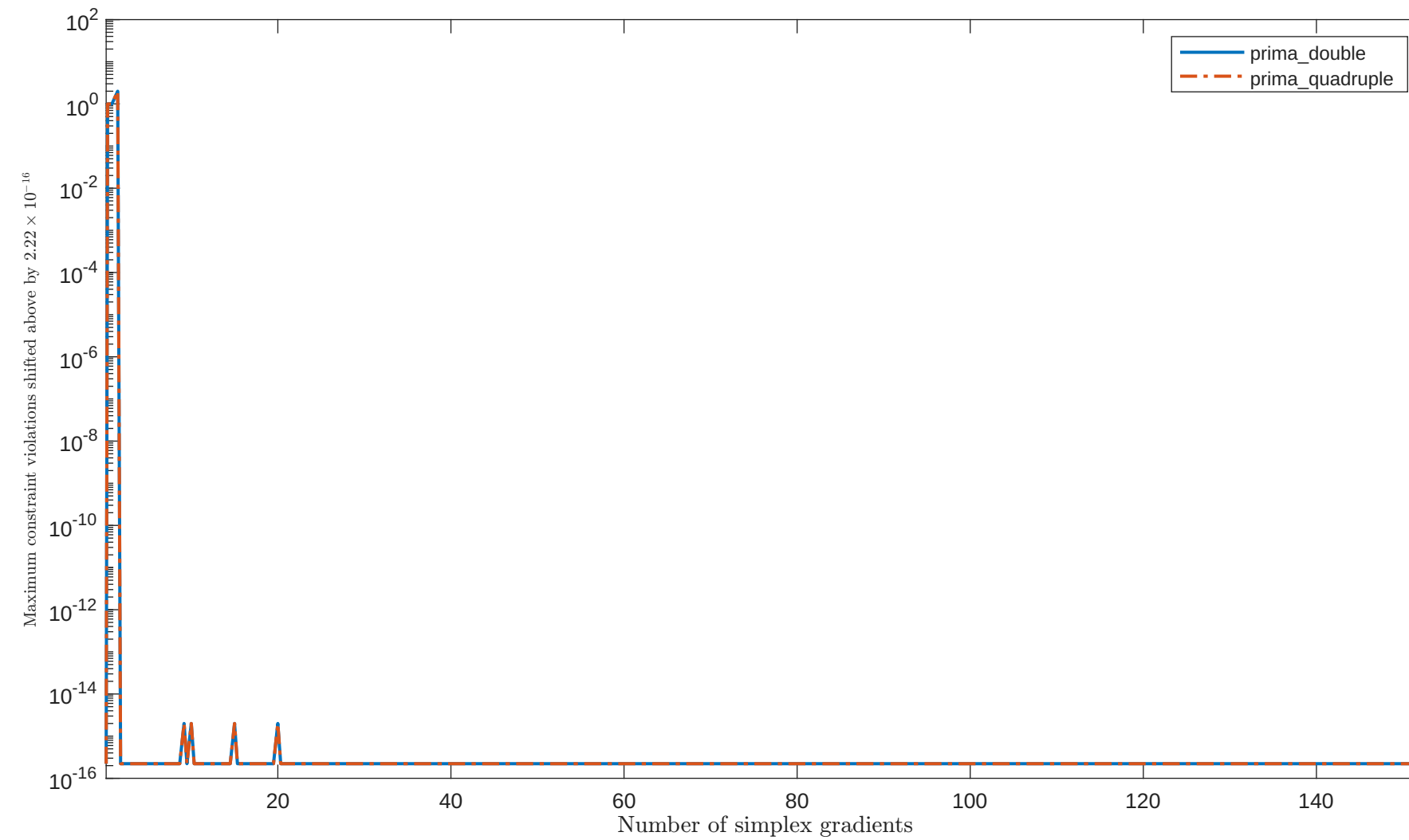
Solving "HS268" with "plain" feature
