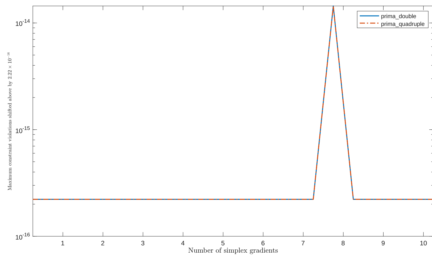
Solving "HS37" with "plain" feature
