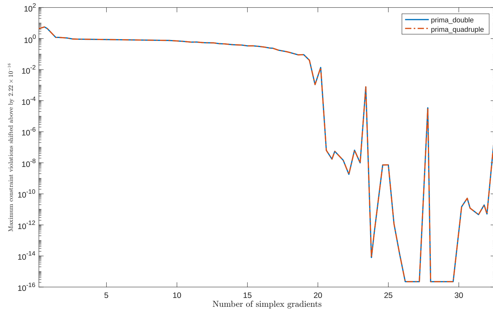
Solving "STREGNE" with "plain" feature
