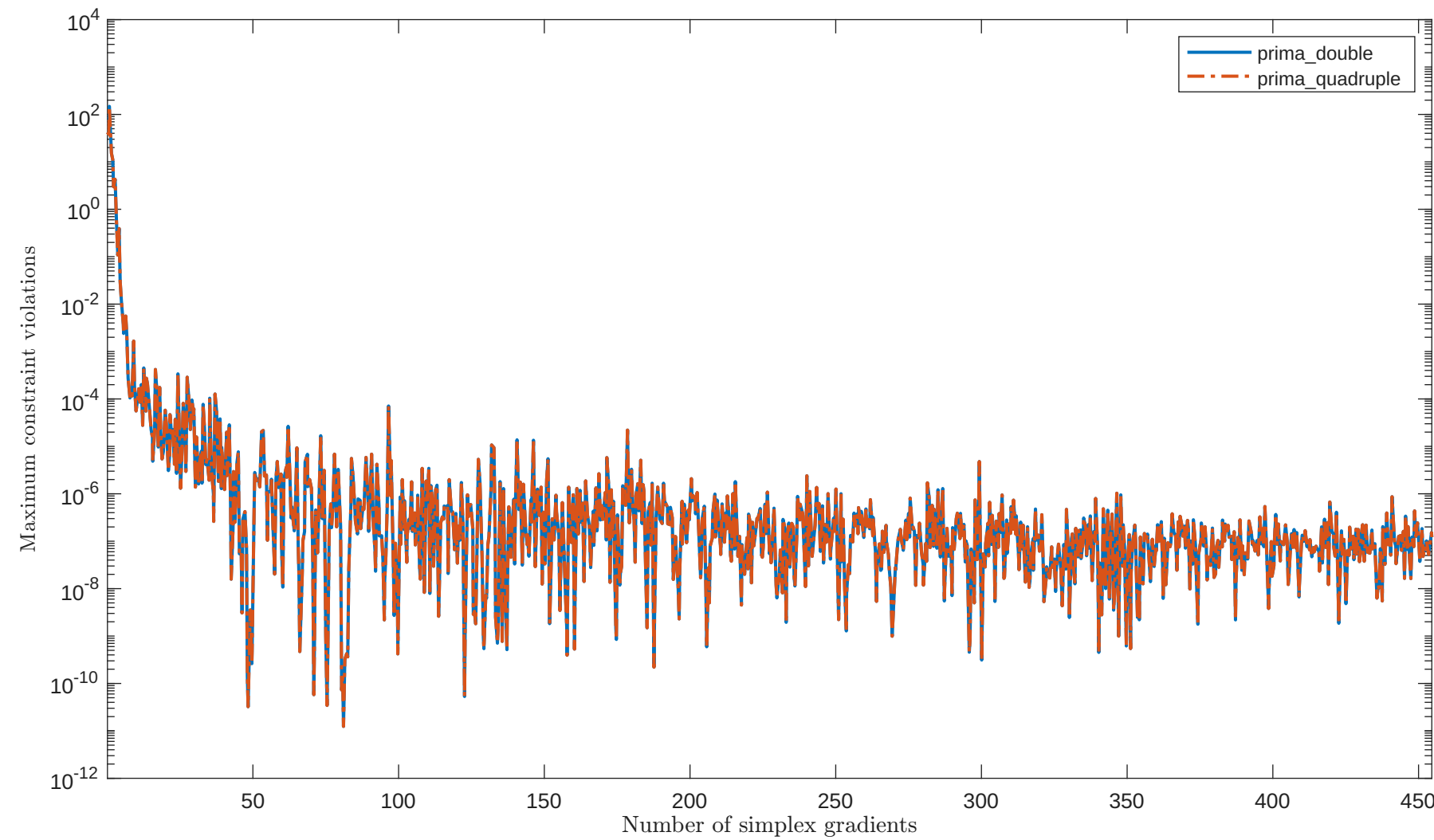
Solving "LUKVLE4" with "plain" feature
