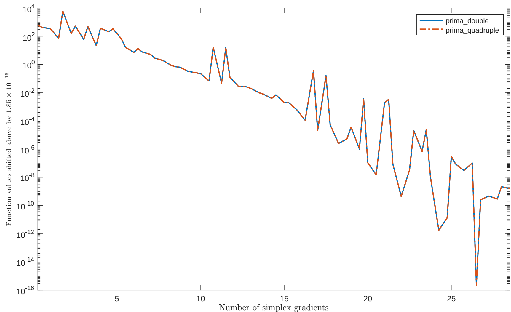
Solving “ENGVAL2” with “plain” feature
