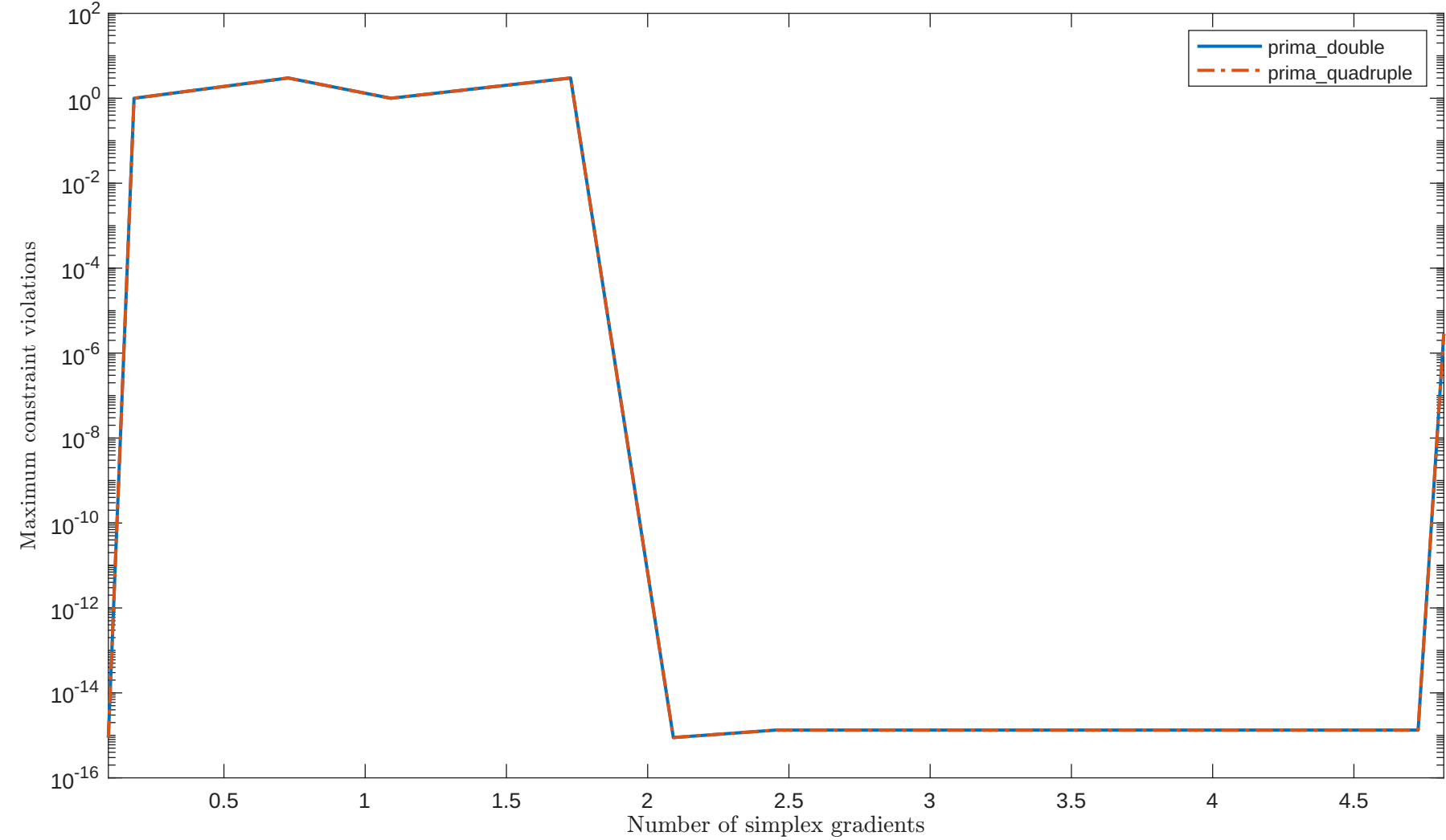
Solving "GENHS28" with "plain" feature
