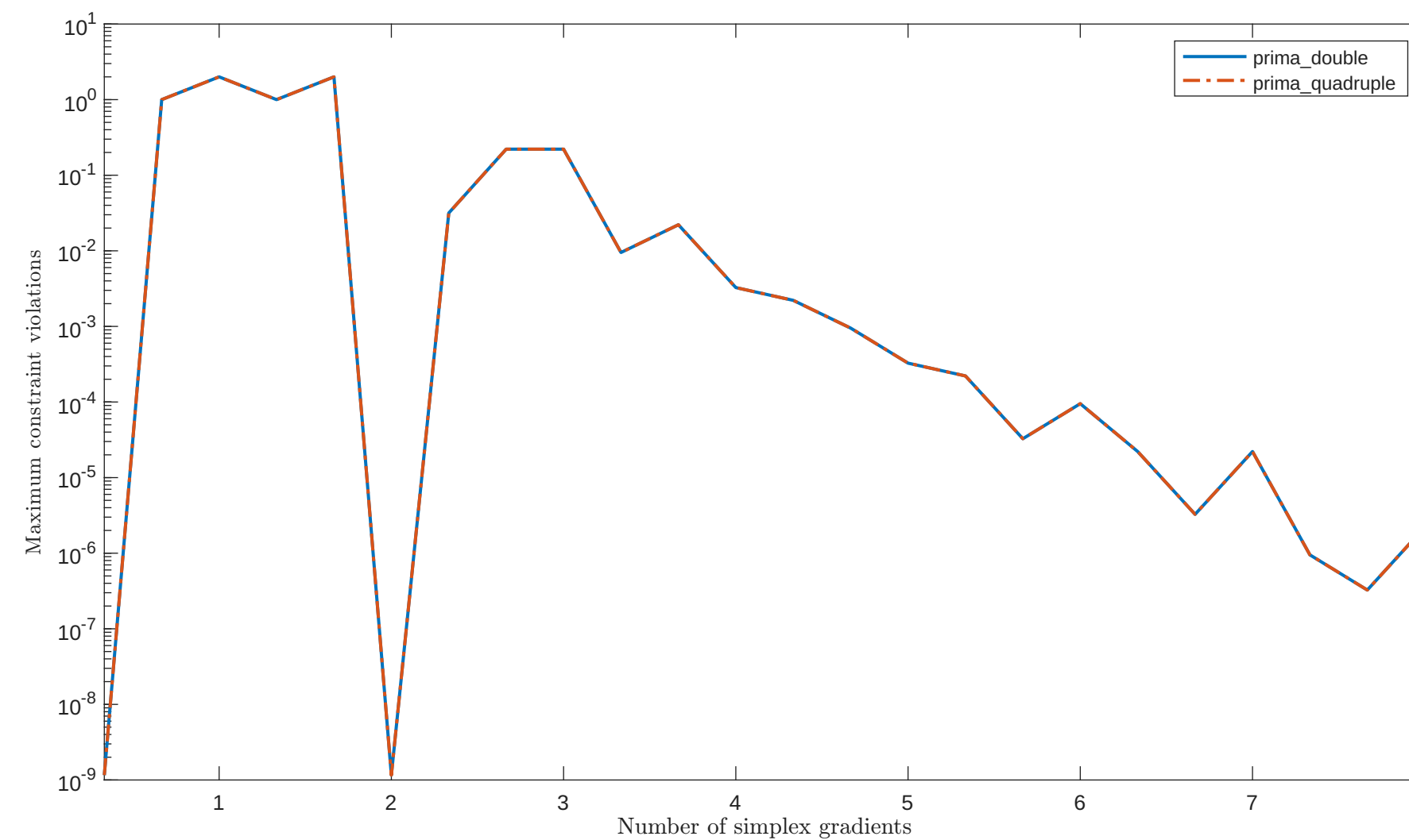
Solving "EXTRASIM" with "plain" feature
