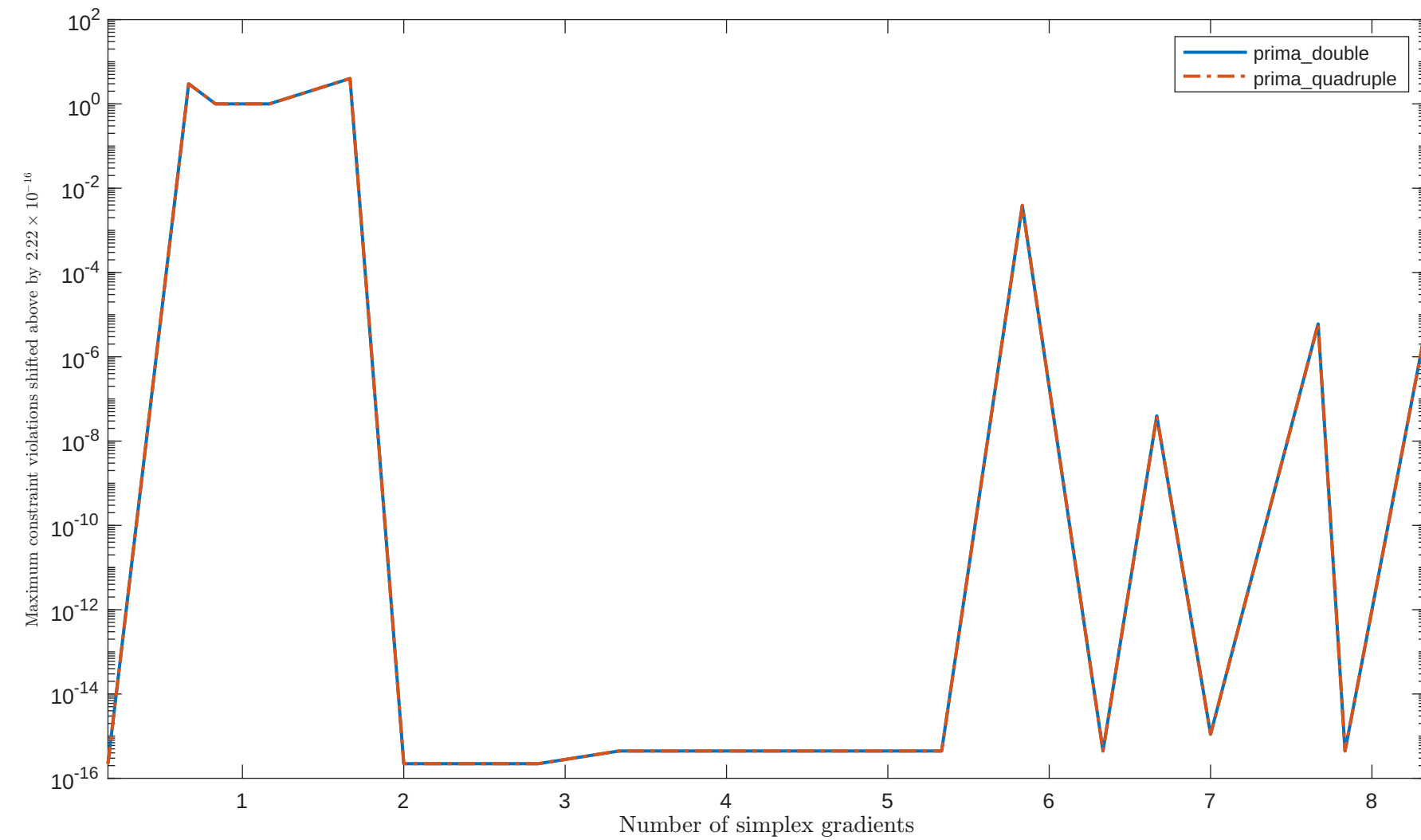
Solving "HS86" with "plain" feature
