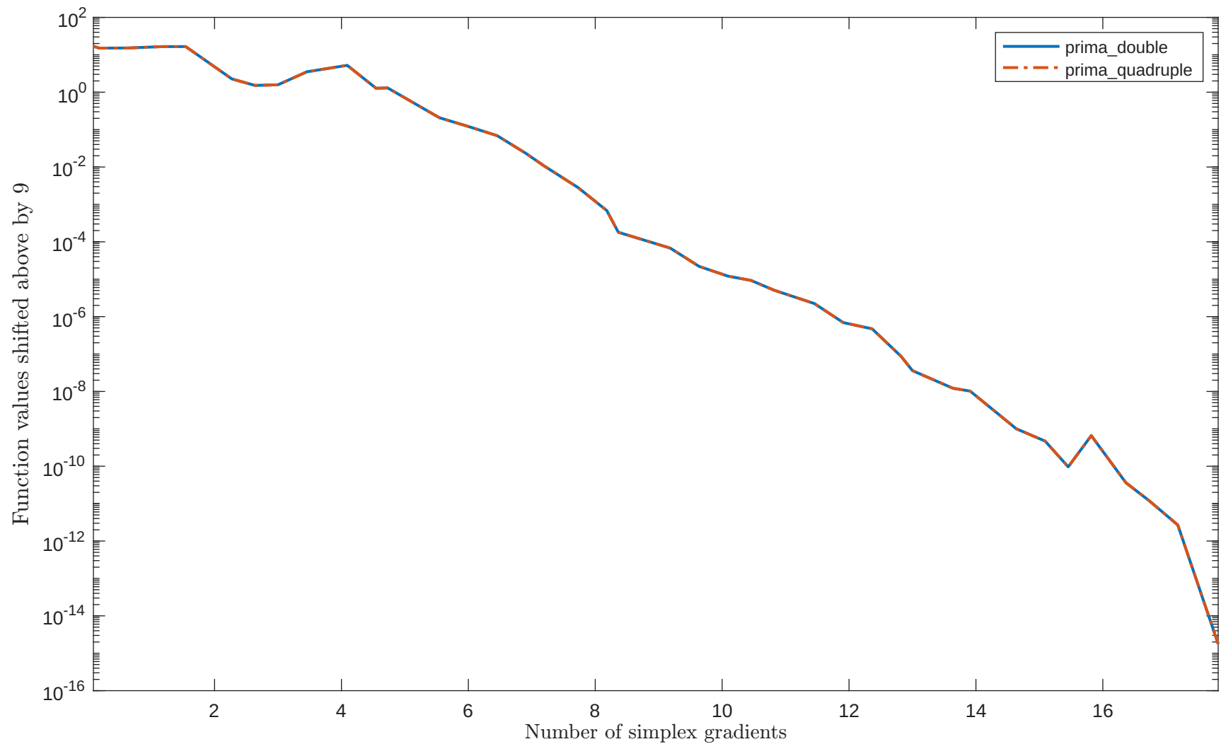
Solving "COSINE" with "plain" feature
