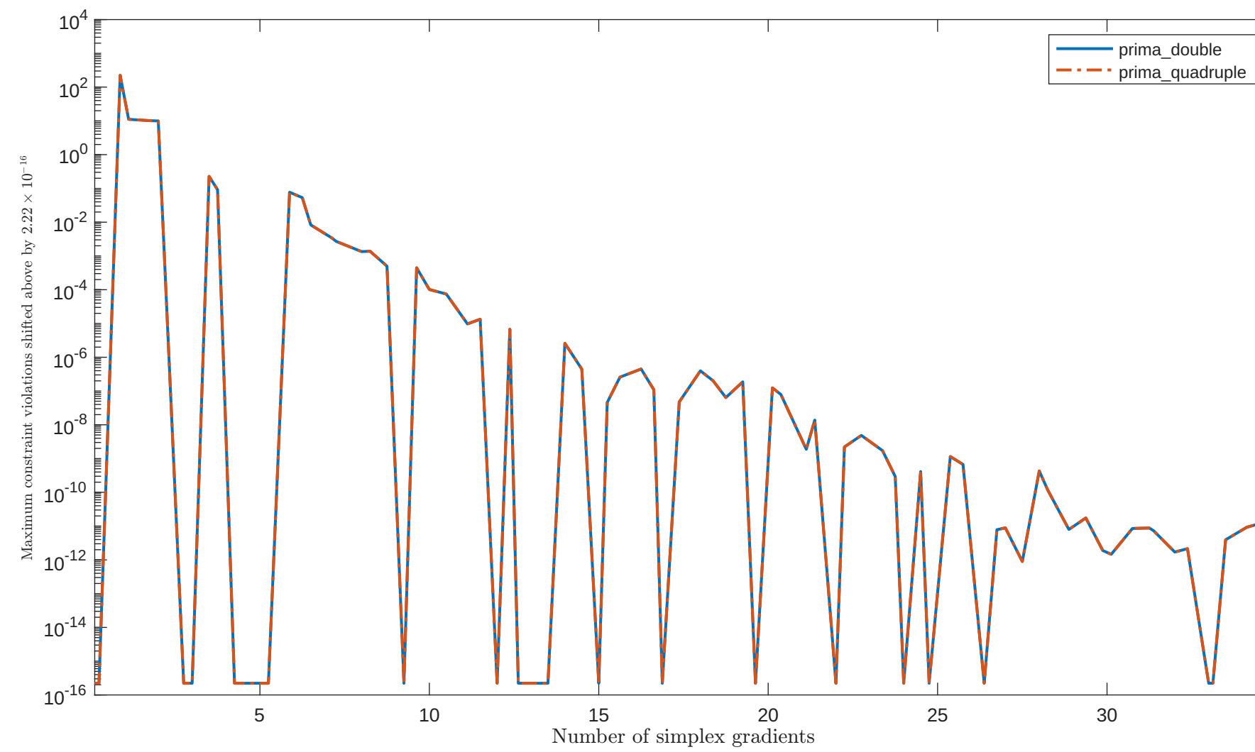
Solving “HS100MOD” with “plain” feature
