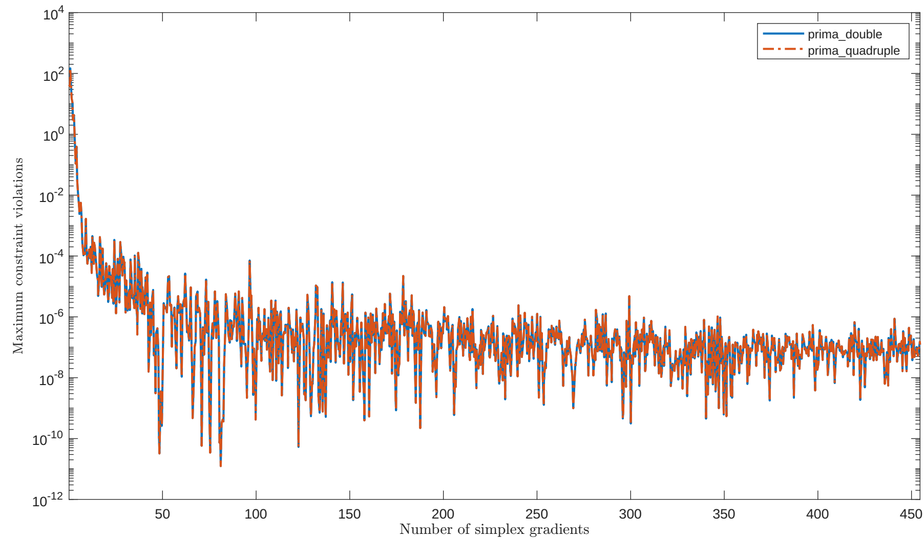
Solving "LUKVL14" with "plain" feature
