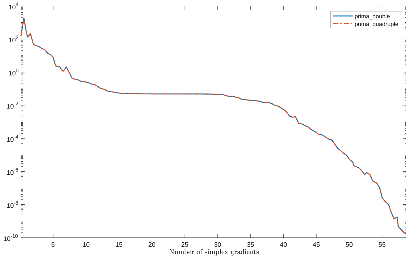
Solving "BROYDNBDLS" with "plain" feature
