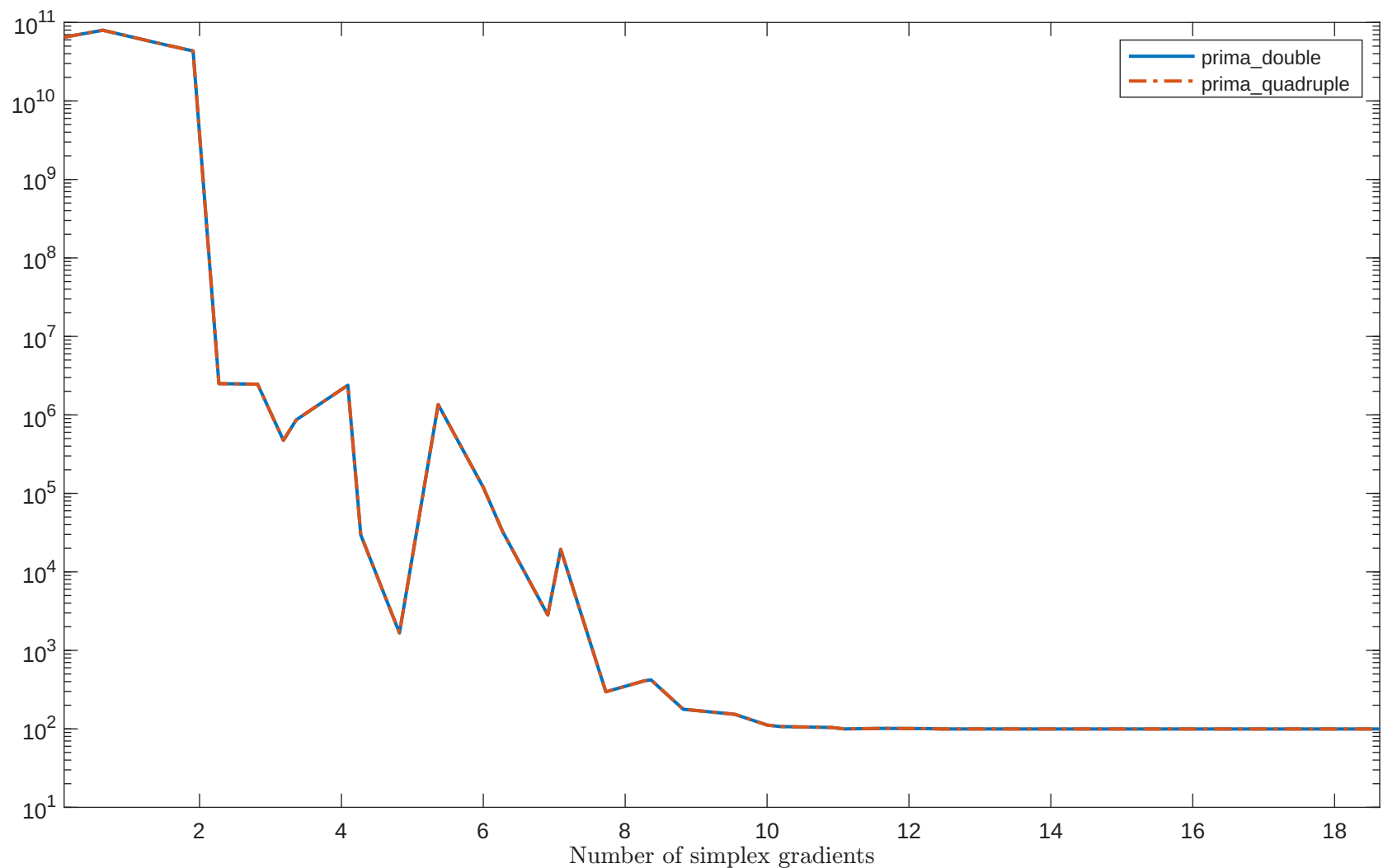
Solving "ARGLINB" with "plain" feature
