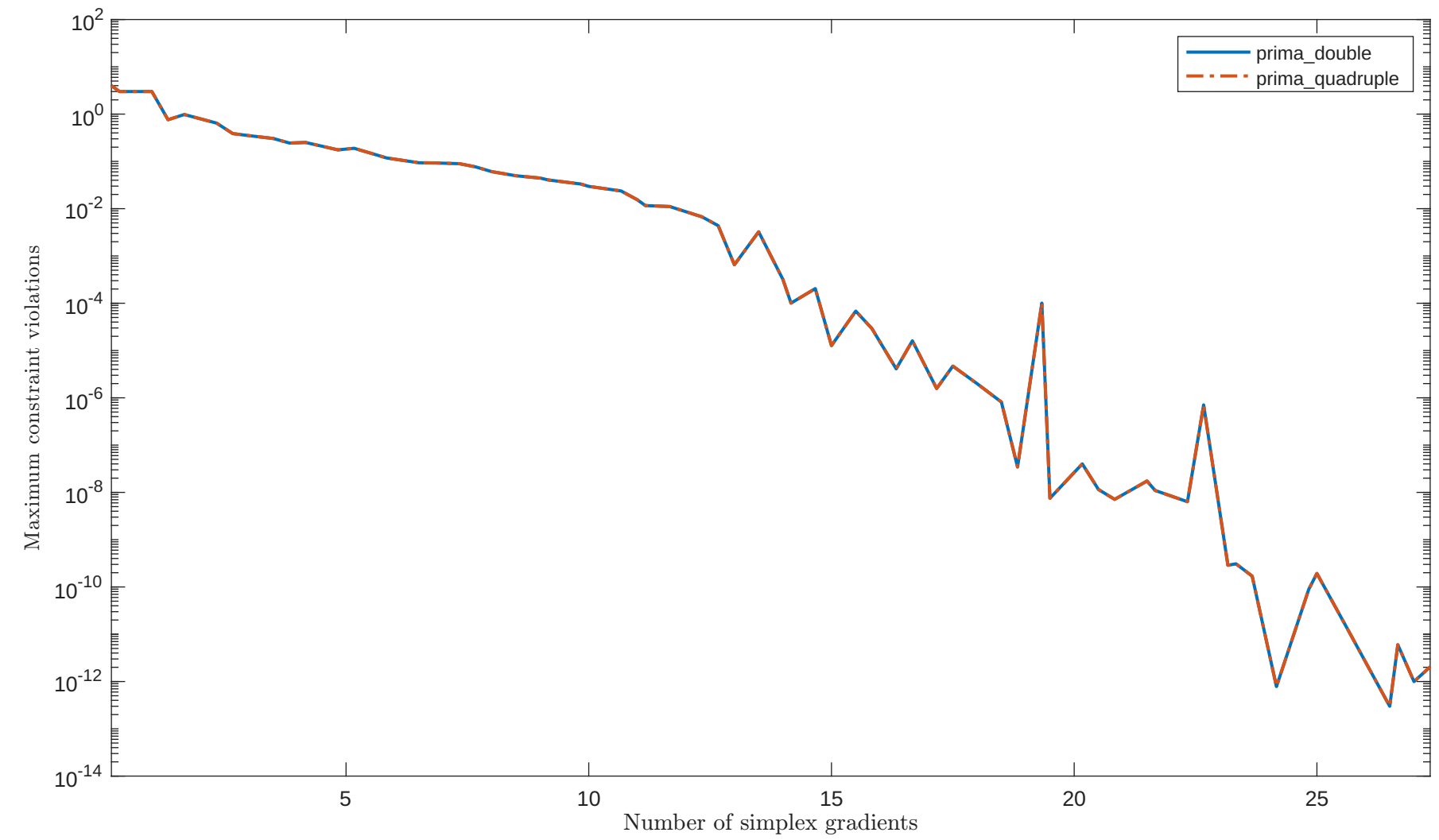
Solving "BT7" with "plain" feature
