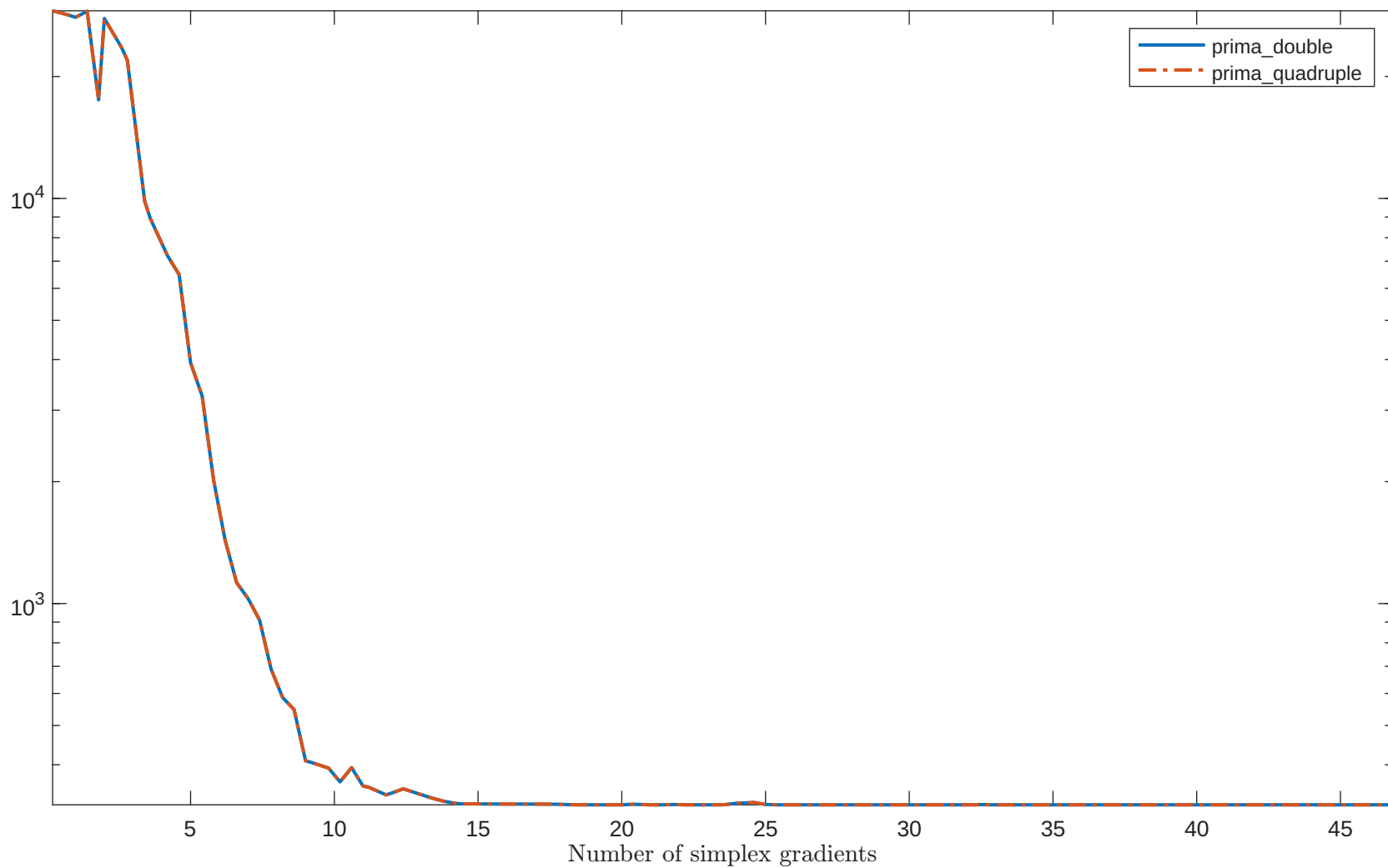
Solving "HIMMELBF" with "plain" feature
