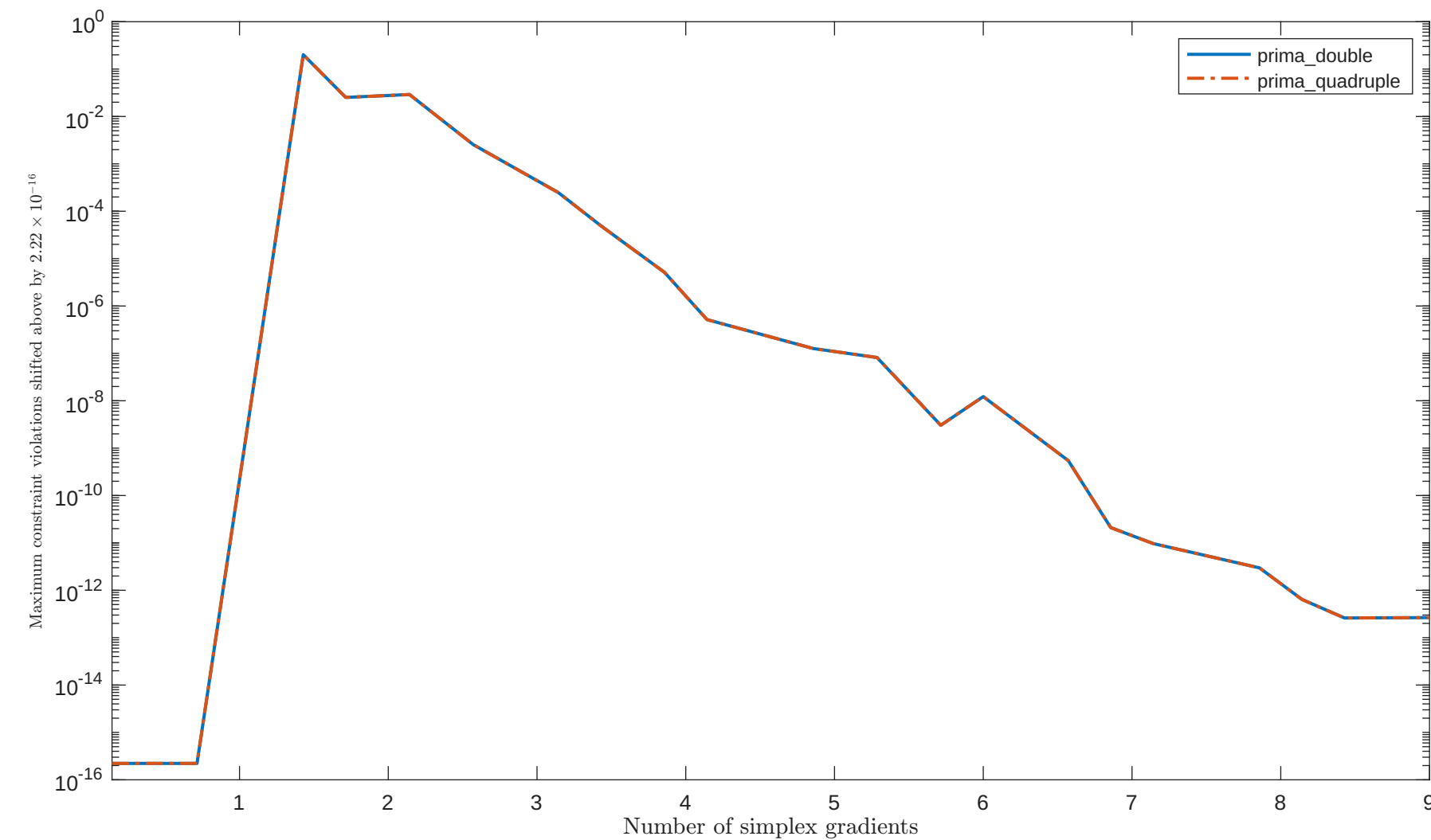
Solving "EIGENACO" with "plain" feature
