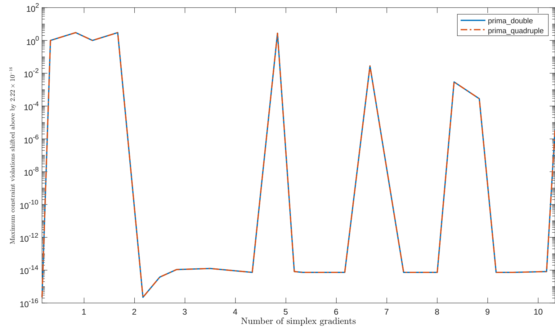
Solving "HS50" with "plain" feature
