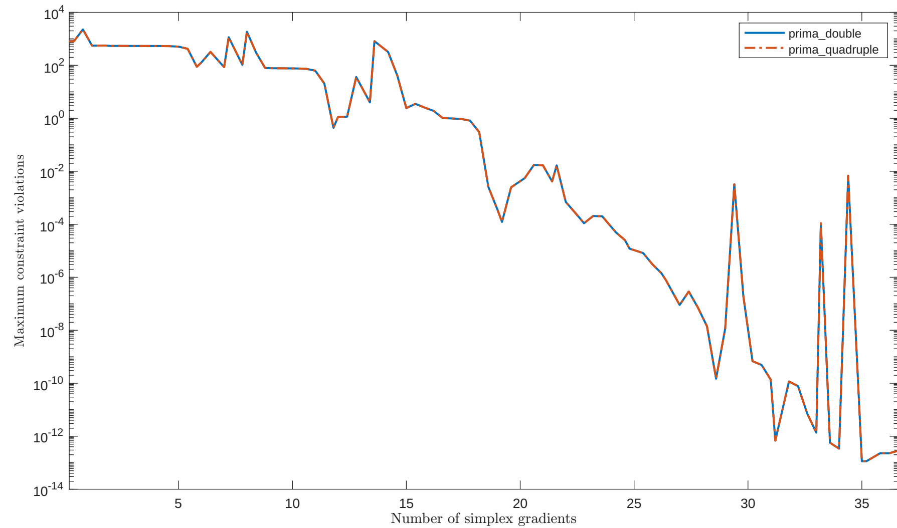
Solving "HS74" with "plain" feature
