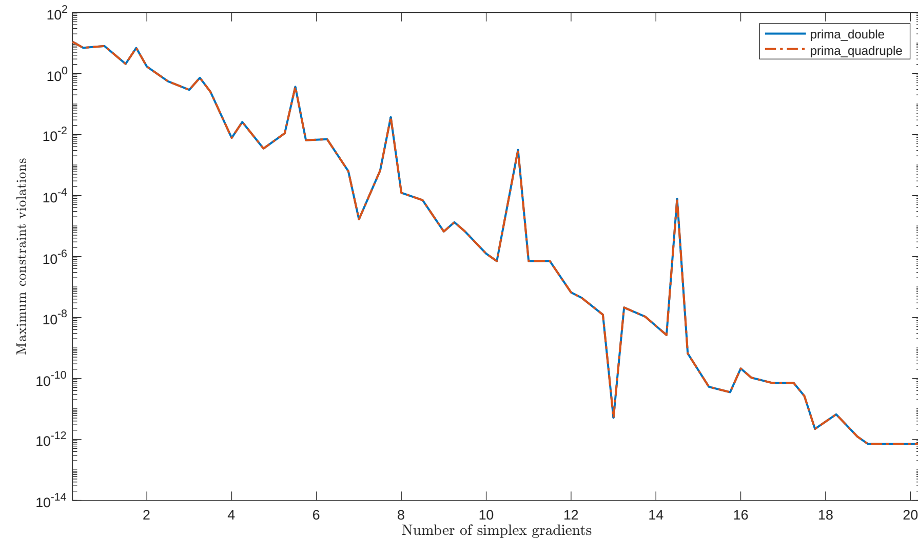
Solving "HS61" with "plain" feature
