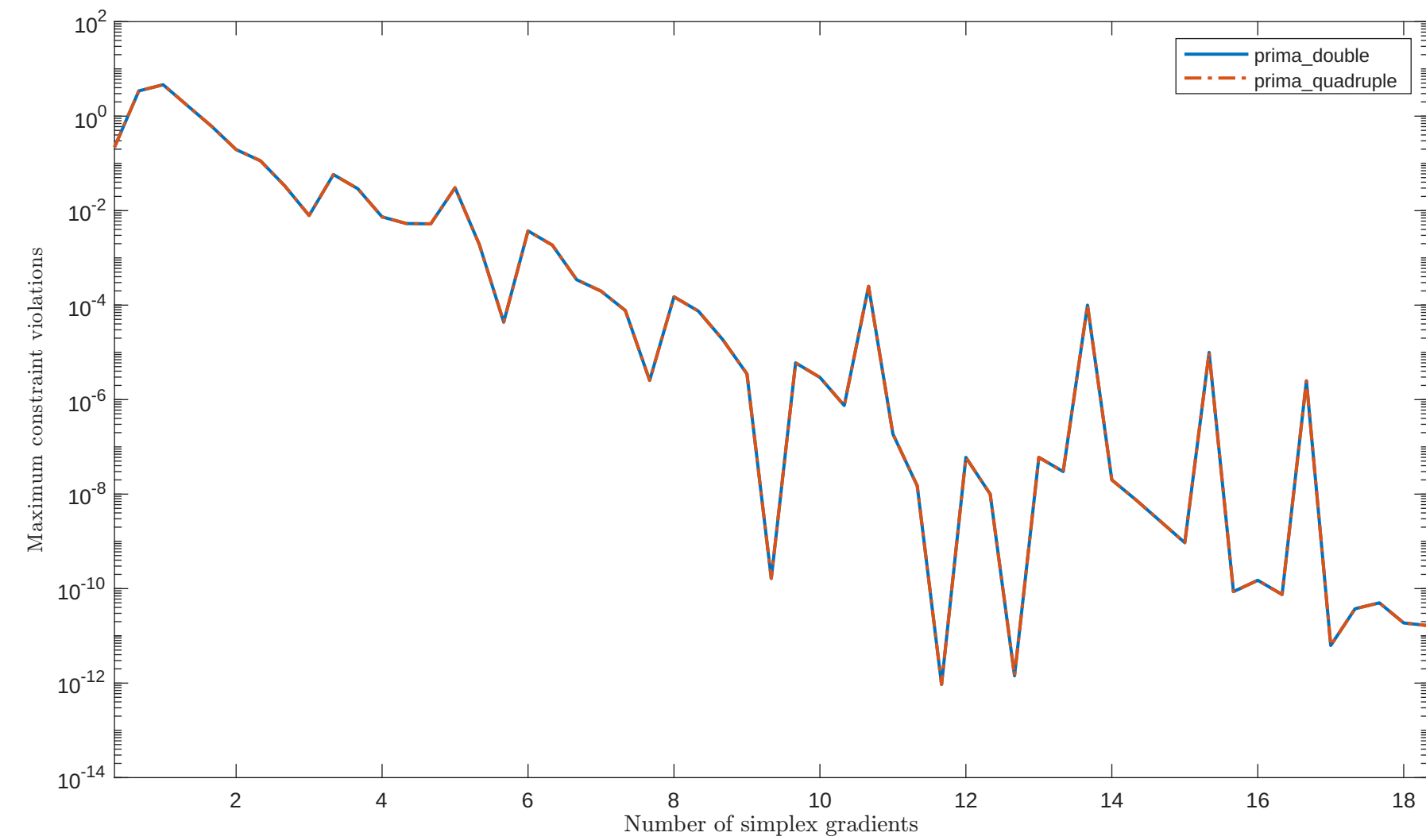
Solving "MARATOS" with "plain" feature
