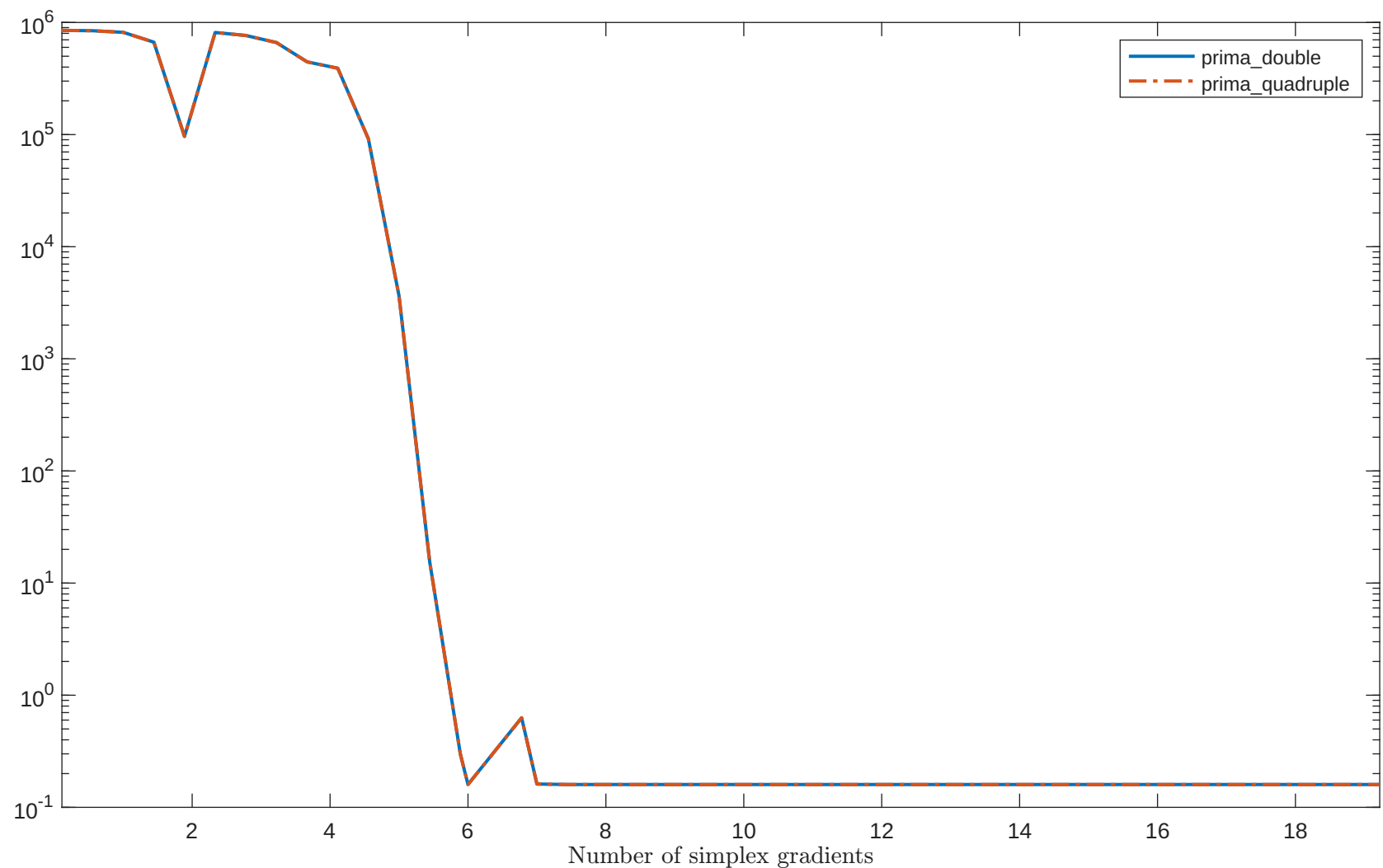
Solving "PALMER8C" with "plain" feature
