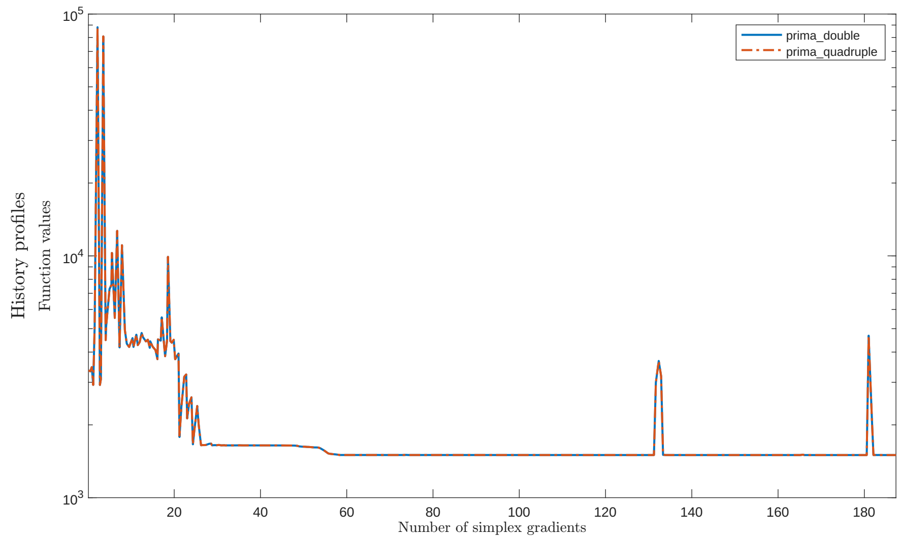
Solving "VESUVIOLS" with "plain" feature
