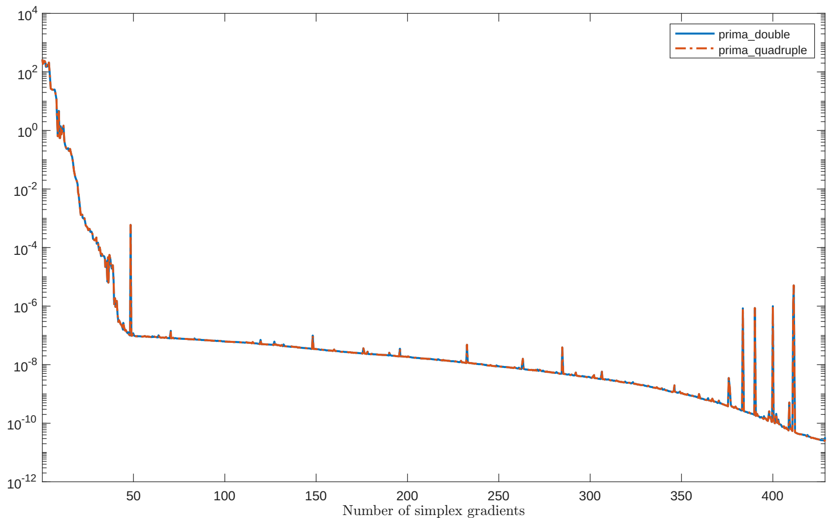
Solving “LANCZOS2LS” with “plain” feature
