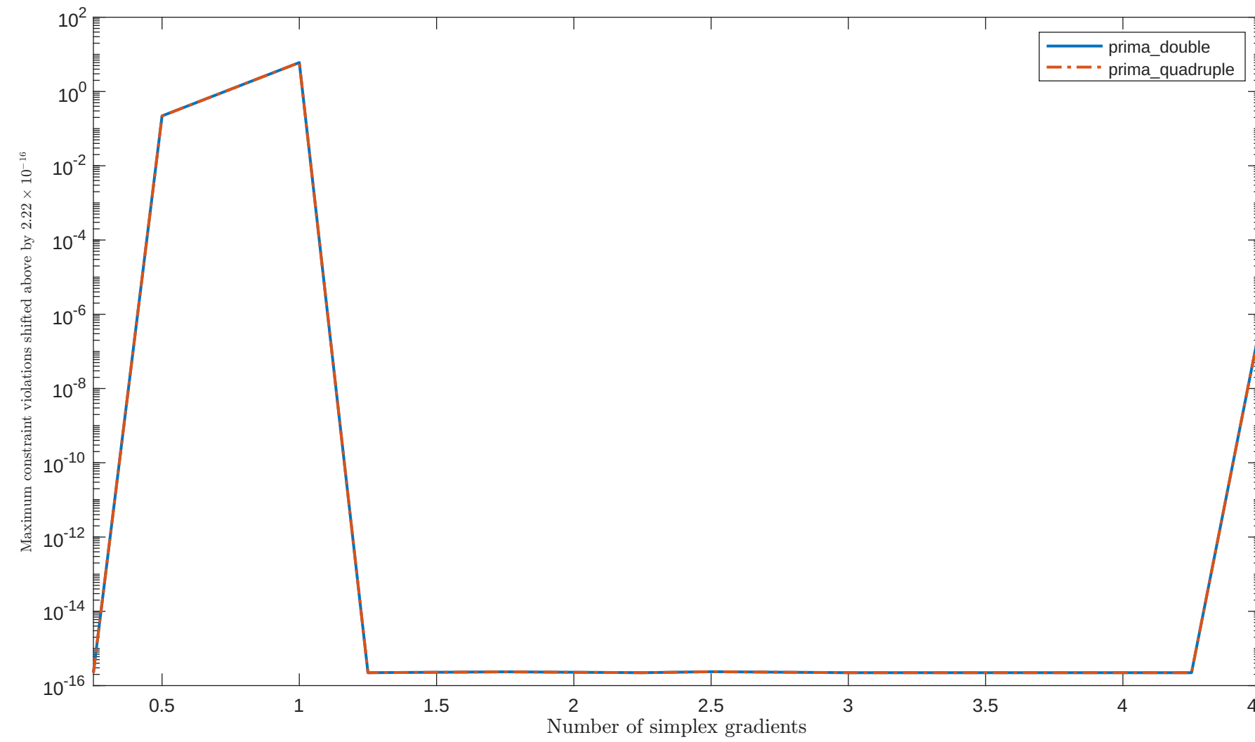
Solving “ZY2” with “plain” feature
