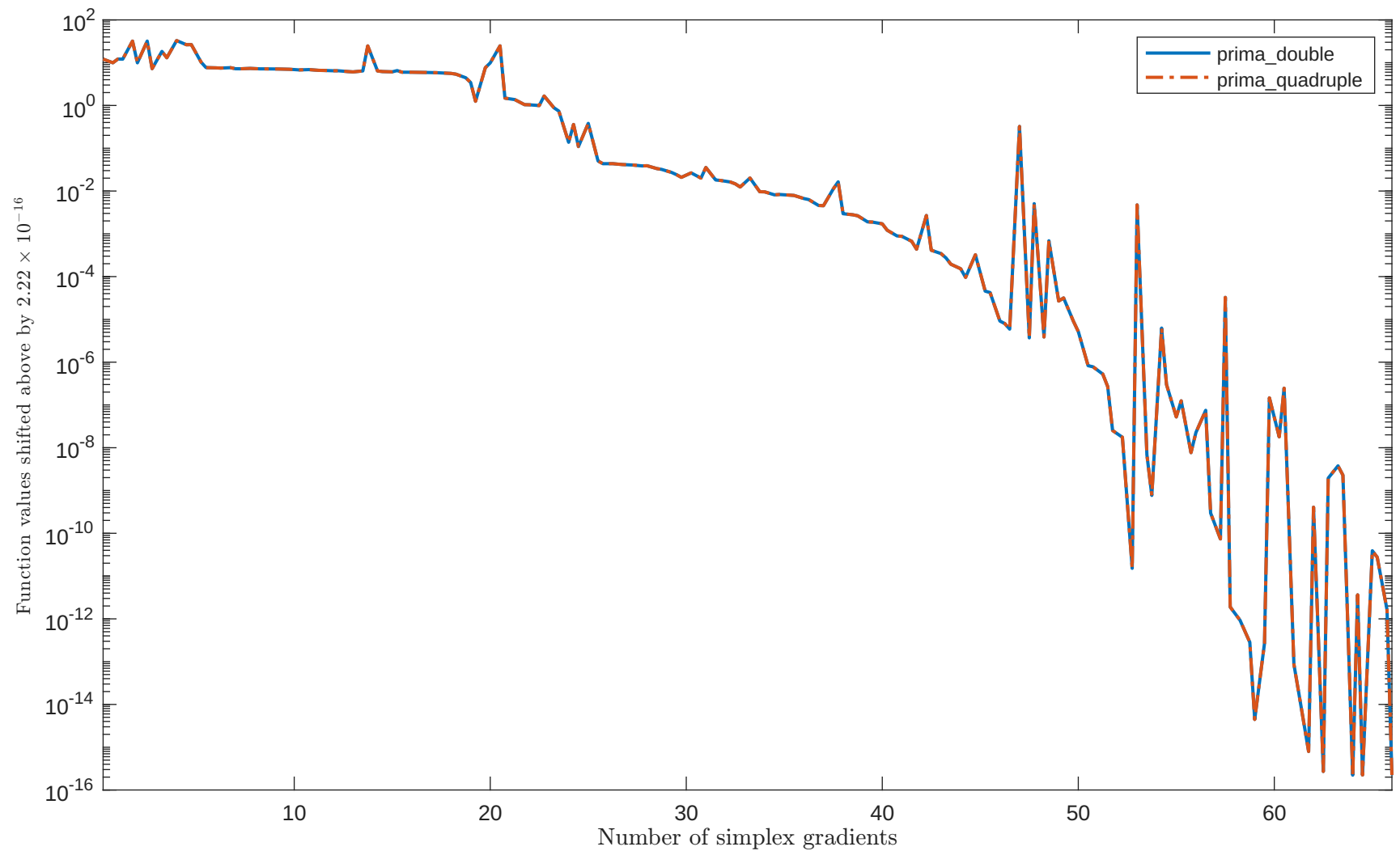
Solving “GULF” with “plain” feature
