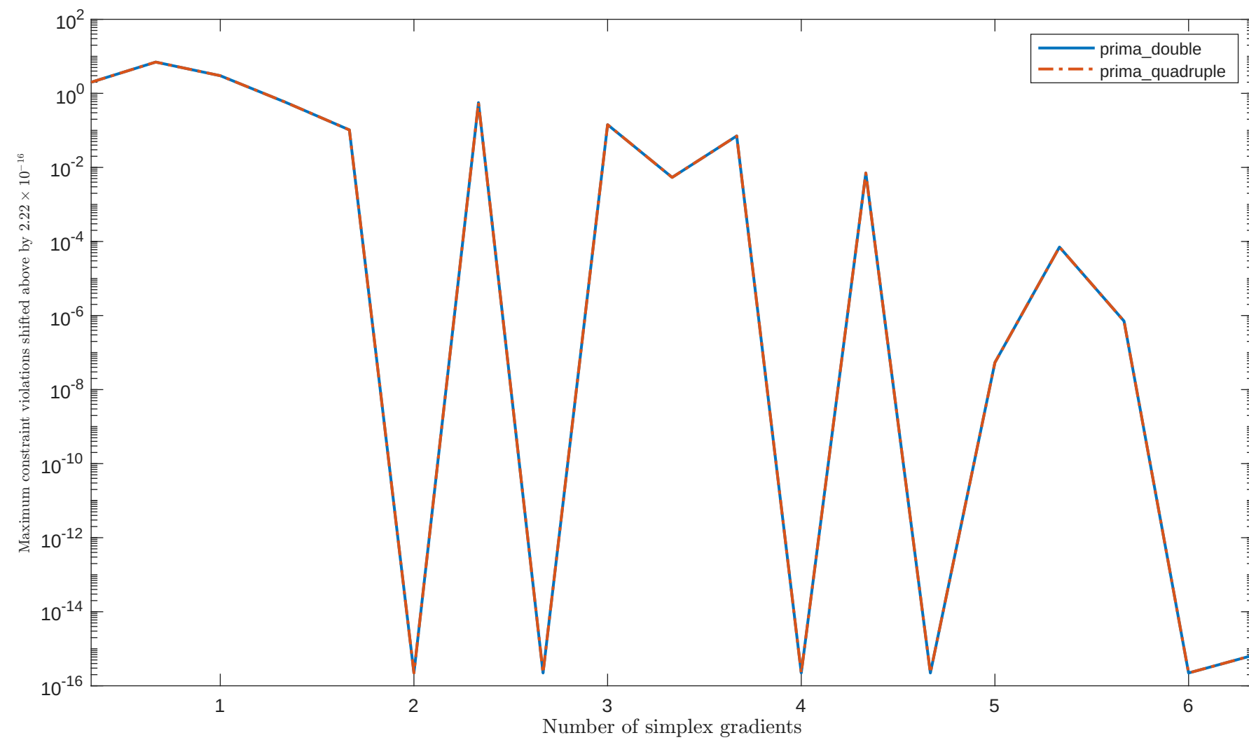
Solving "HS22" with "plain" feature
