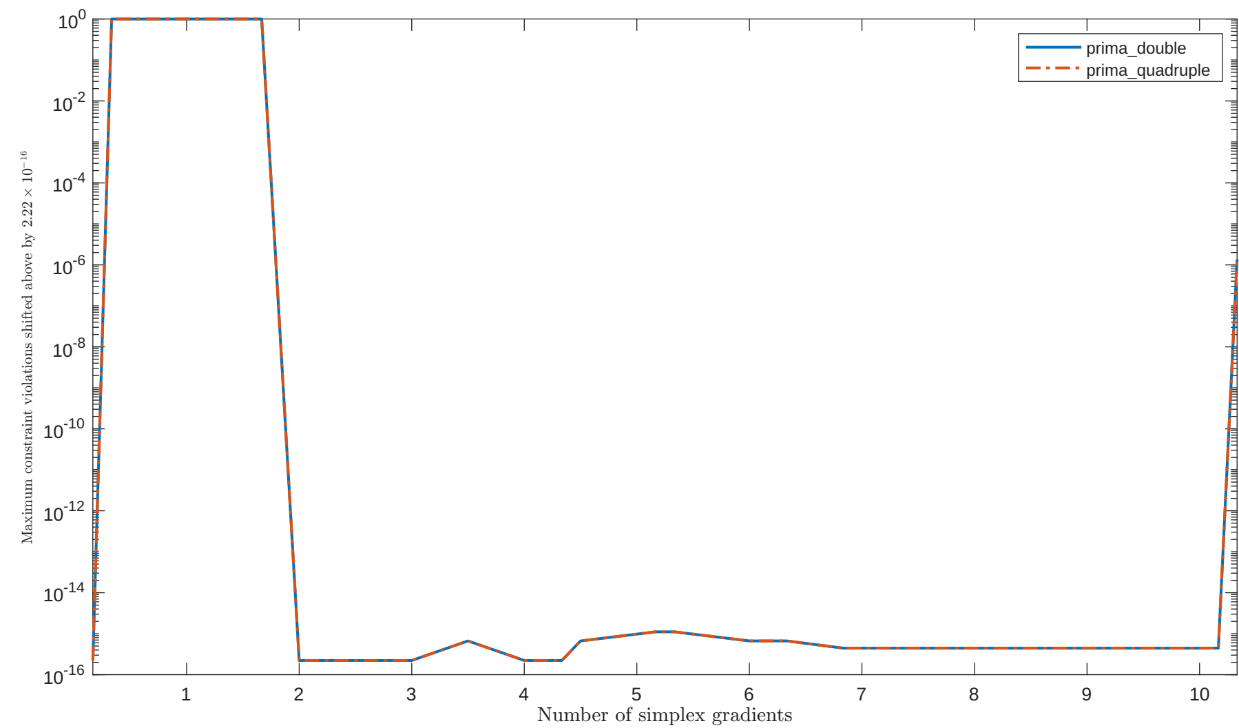
Solving "LSNNODOC" with "plain" feature
