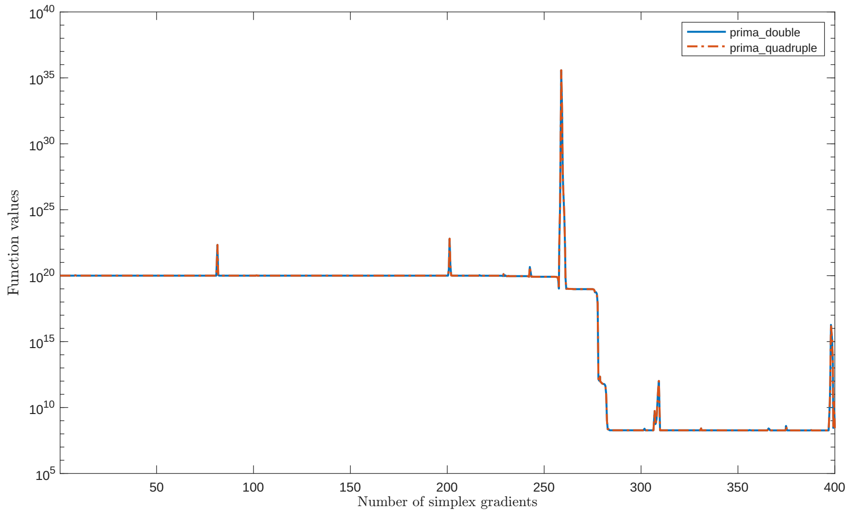
Solving "STREG" with "plain" feature
