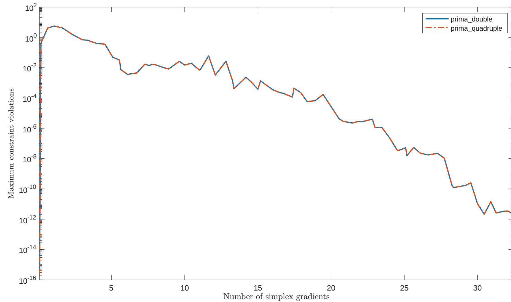
Solving "DIXCHLNV" with "plain" feature
