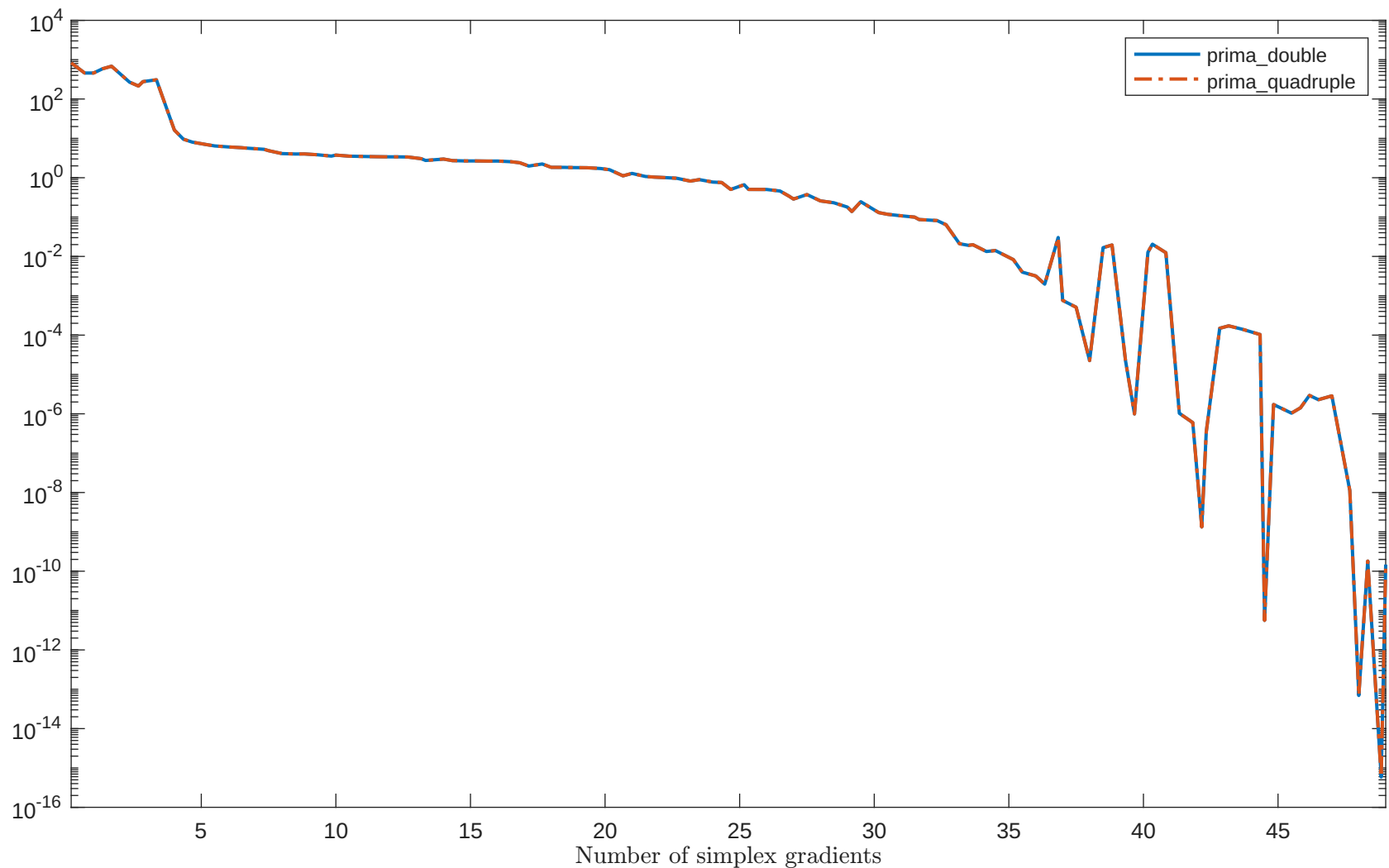
Solving "CHNROSNB" with "plain" feature
