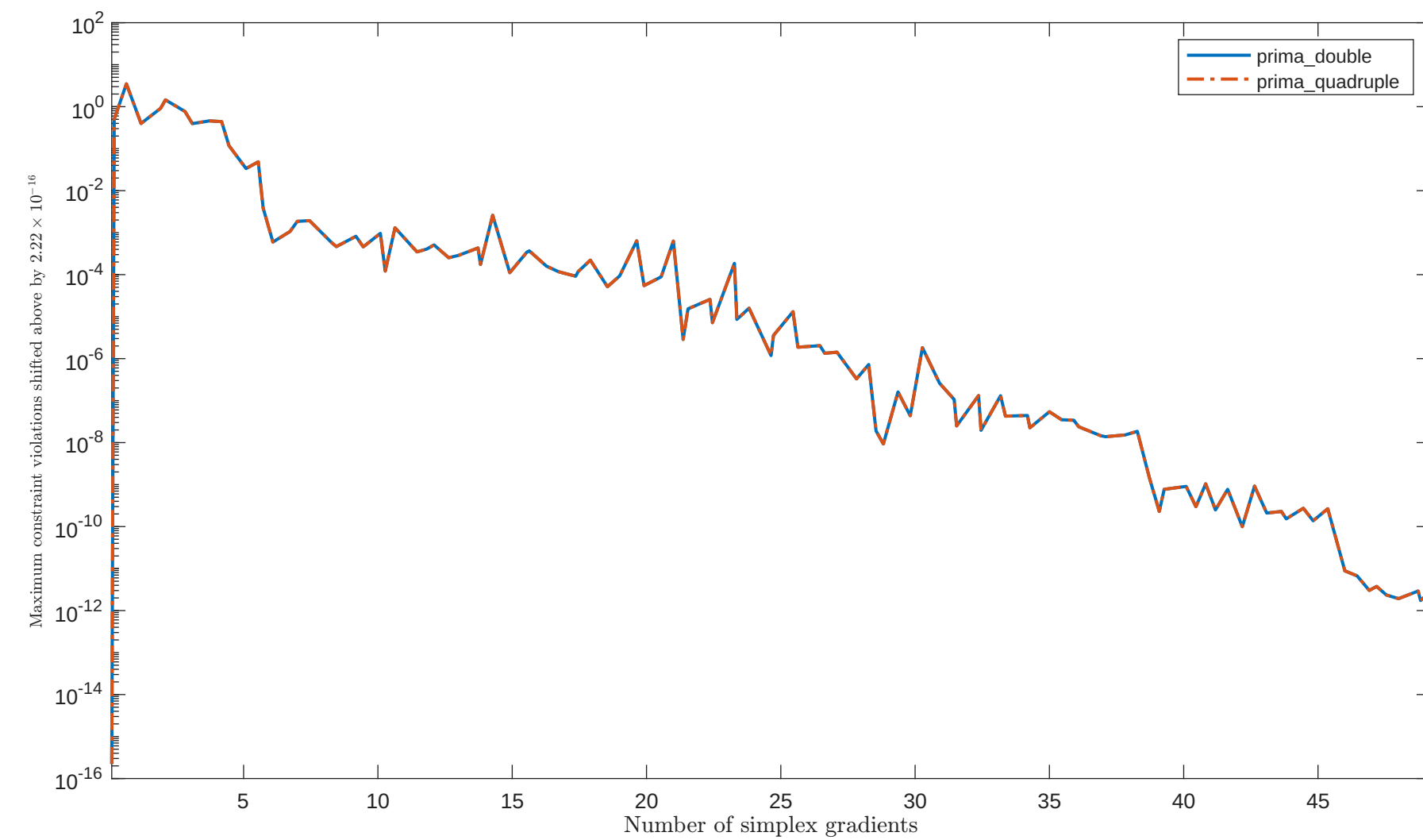
Solving "DIXCHLNG" with "plain" feature
