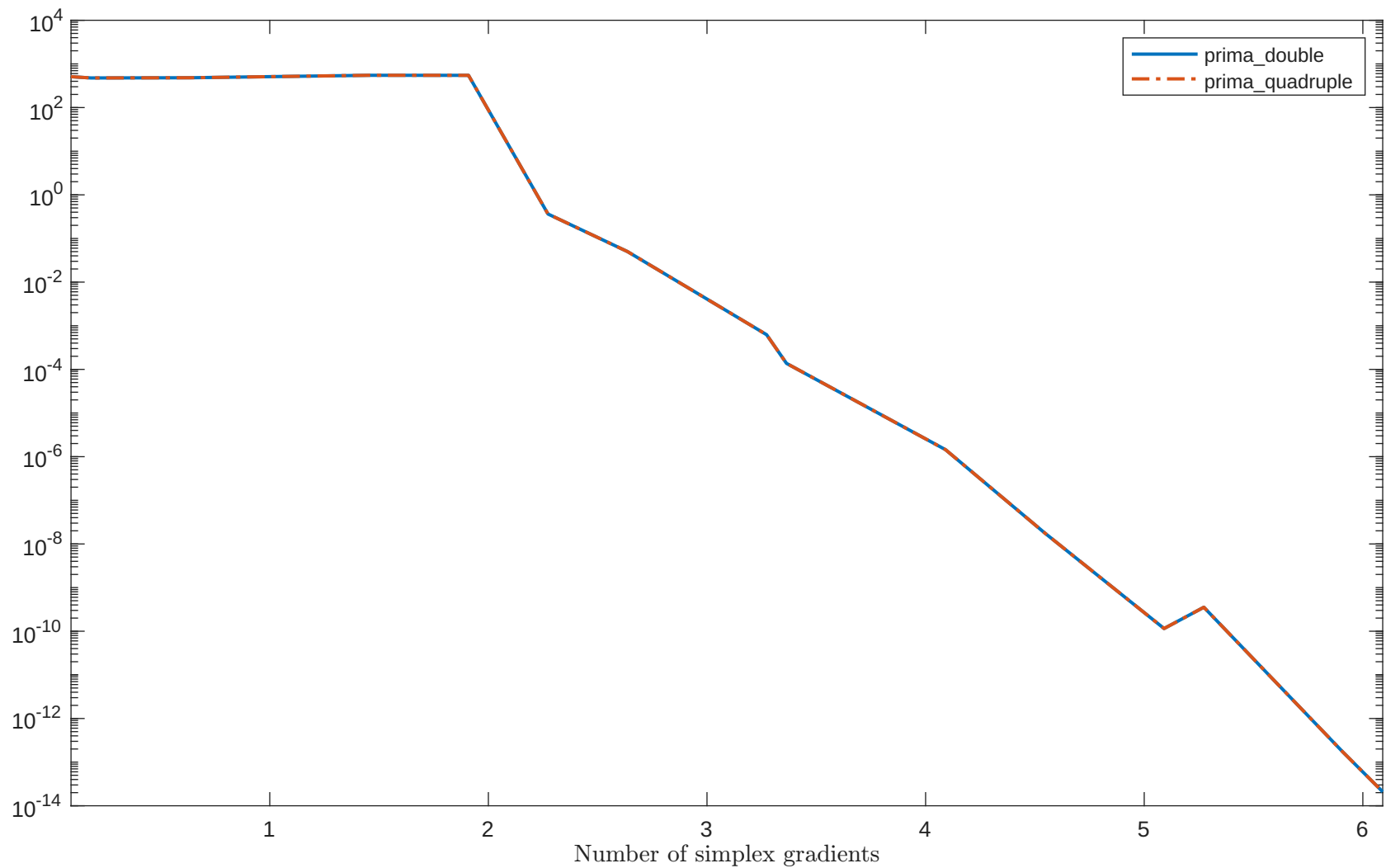
Solving "HILBERTB" with "plain" feature
