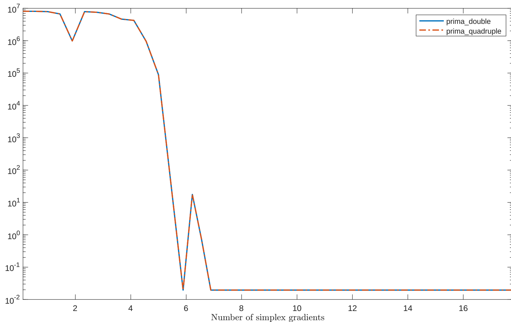
Solving "PALMER3C" with "plain" feature
