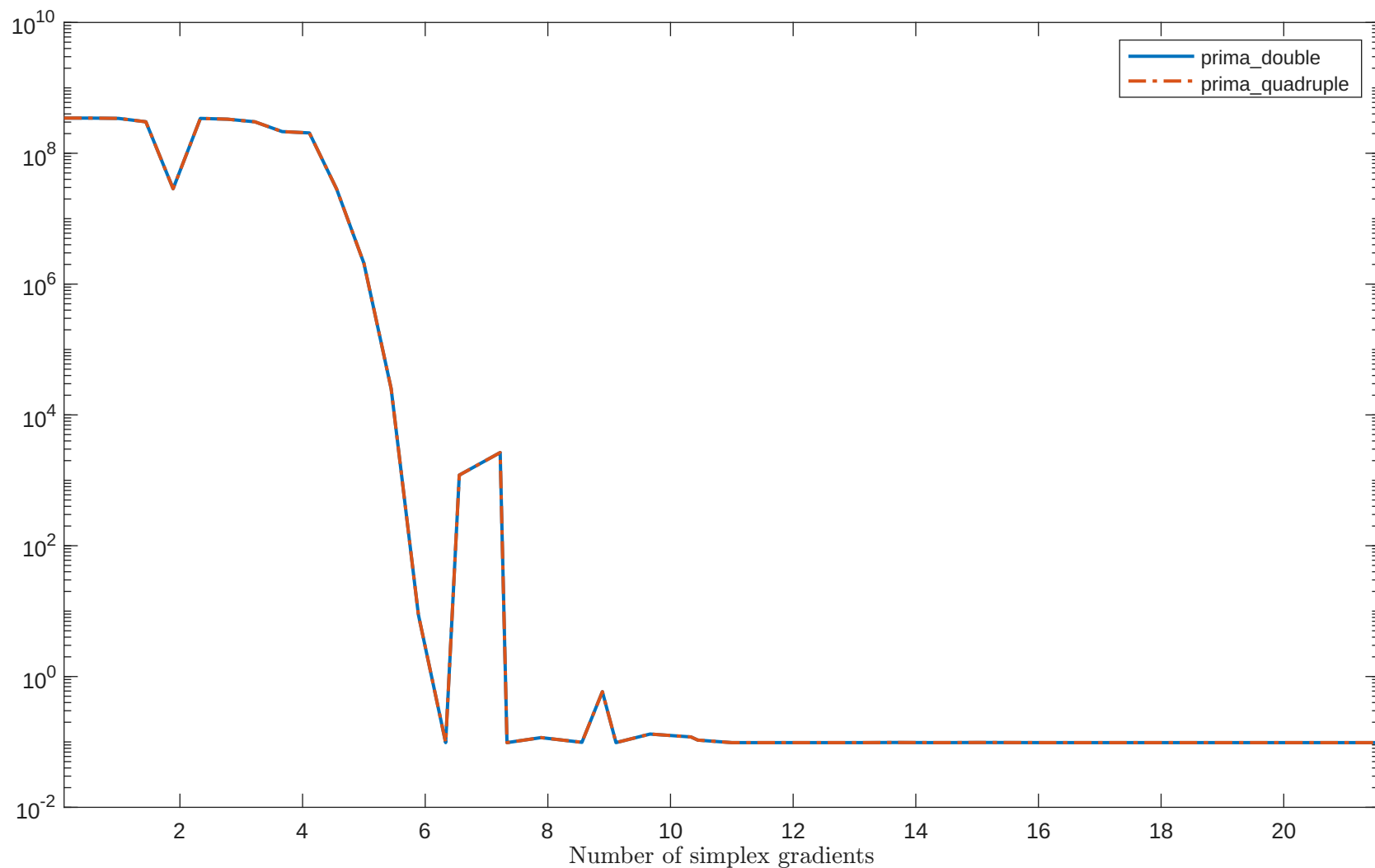
Solving "PALMER1C" with "plain" feature
