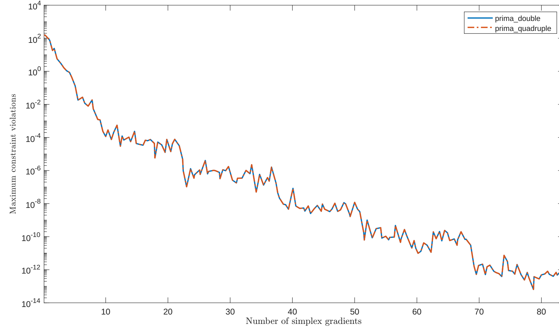
Solving "LUKVLE3" with "plain" feature
