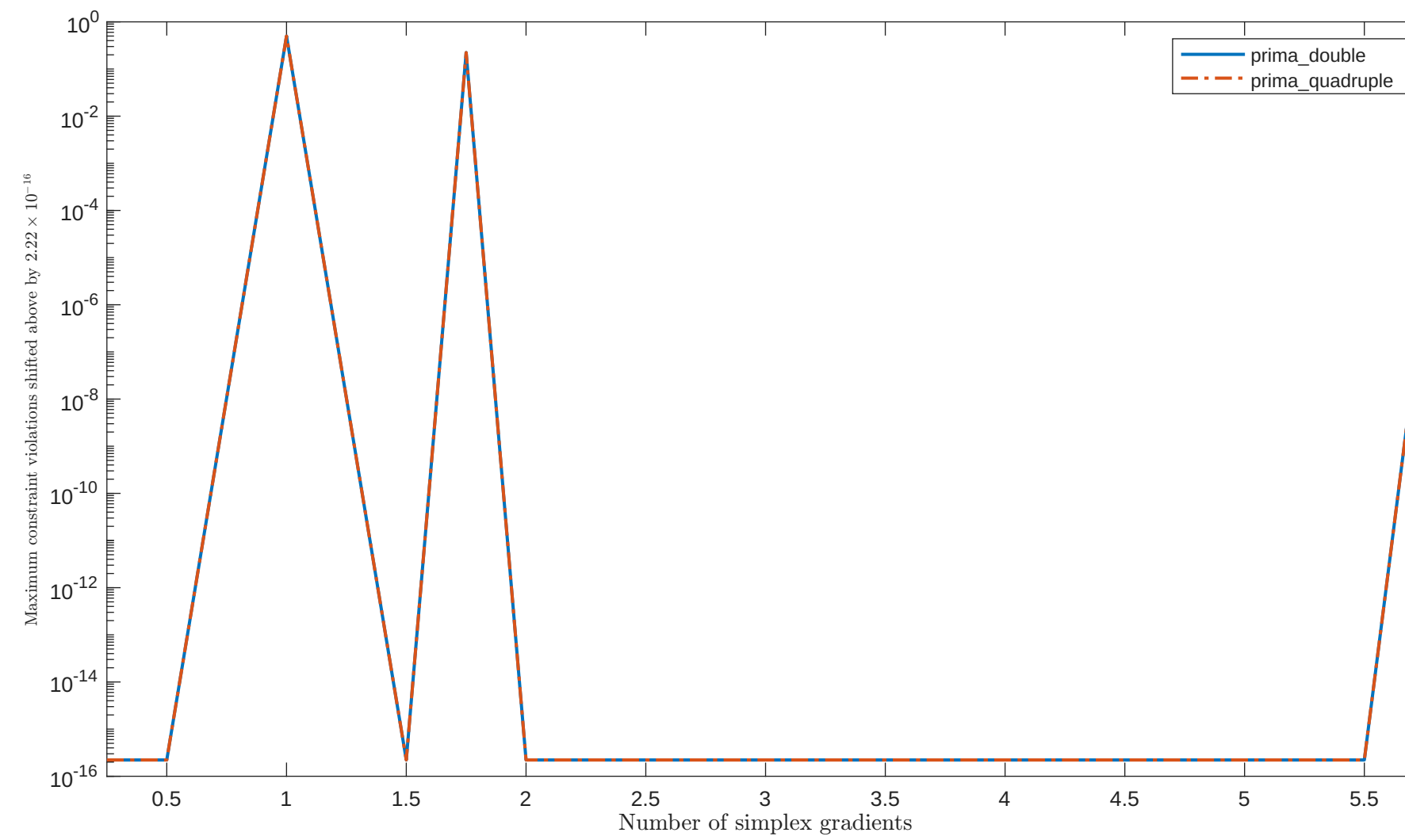
Solving “HS35MOD” with “plain” feature
