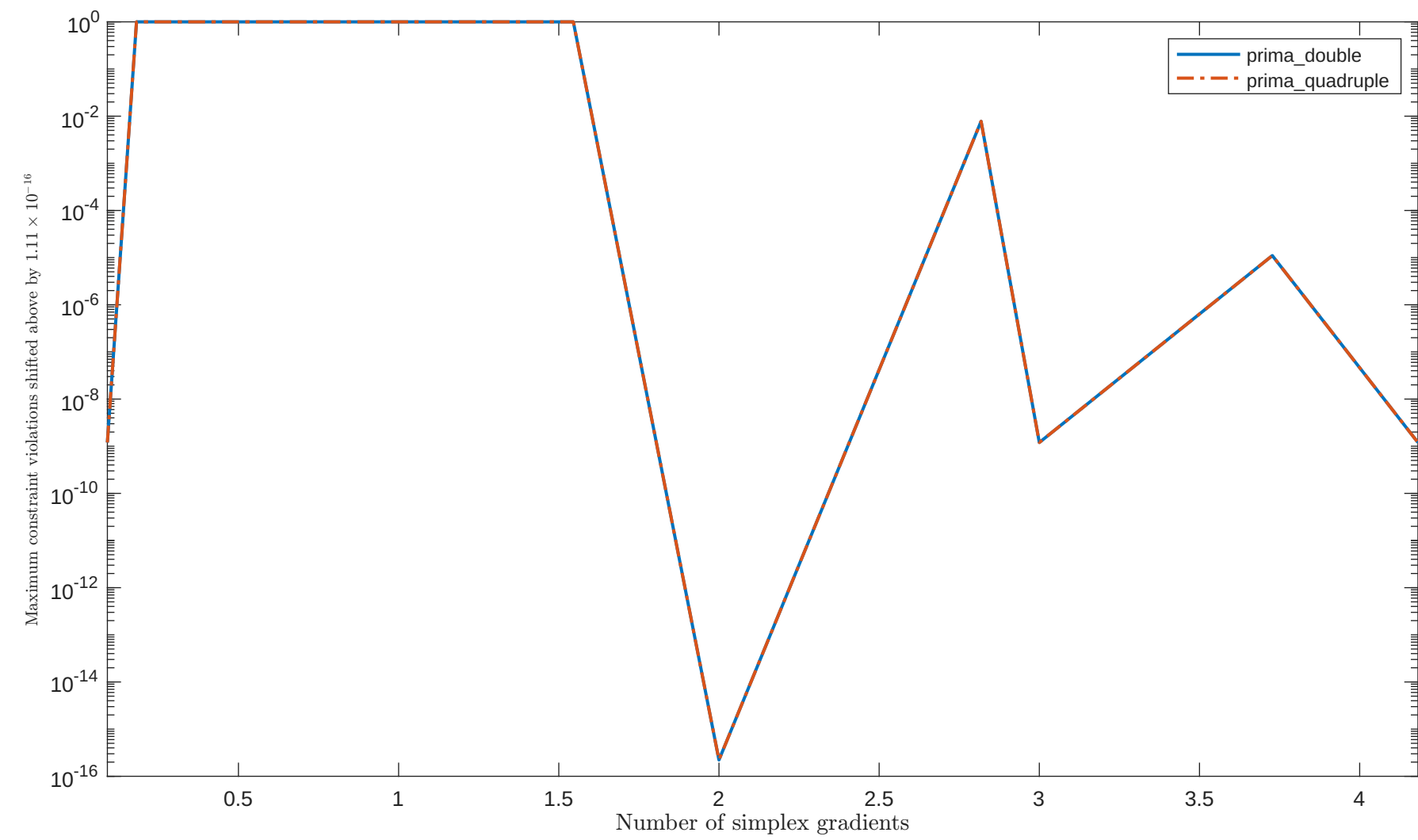
Solving “PORTSNQP” with “plain” feature
