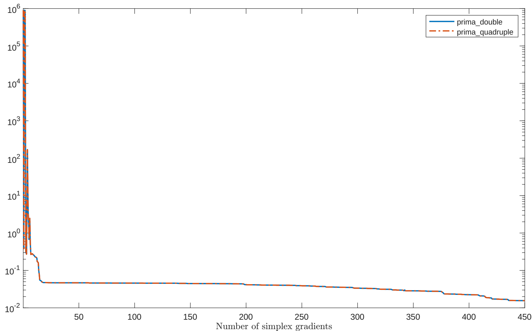
Solving “COOLHANSLS” with “plain” feature
