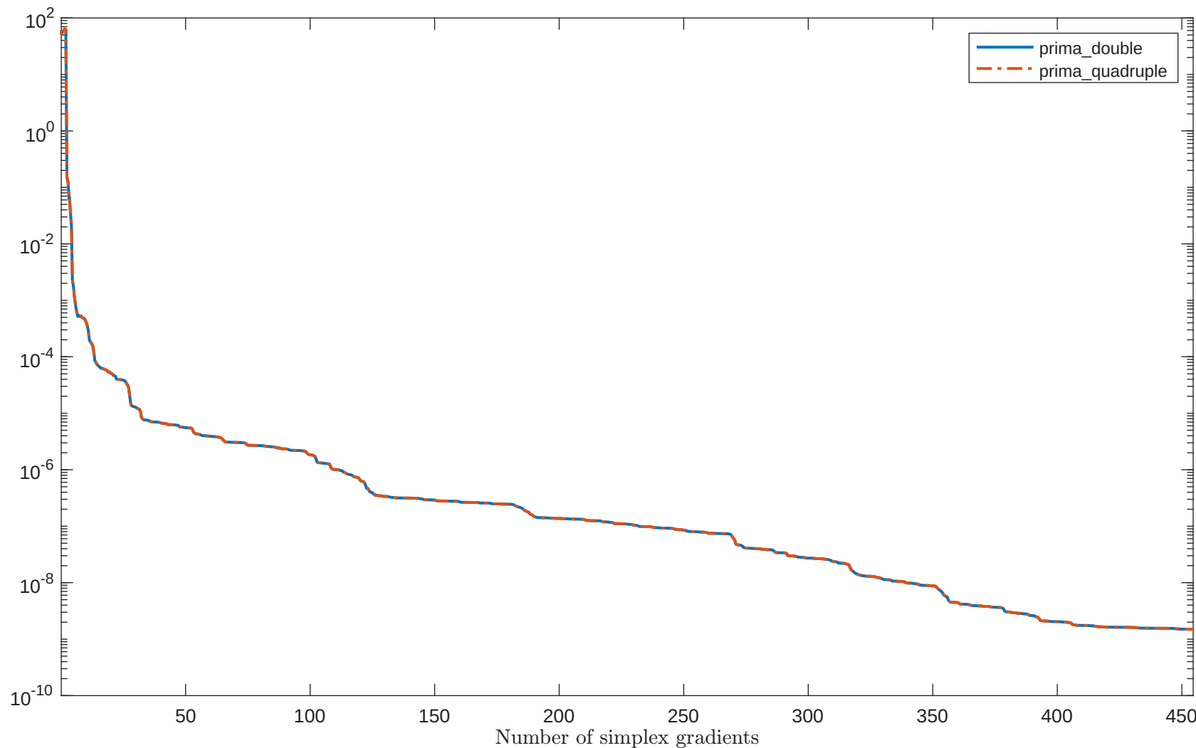
Solving "HILBERTA" with "plain" feature
