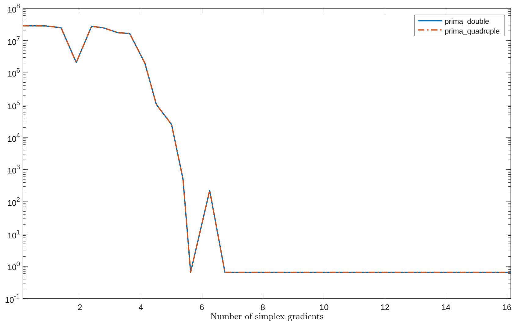
Solving "PALMER1D" with "plain" feature
