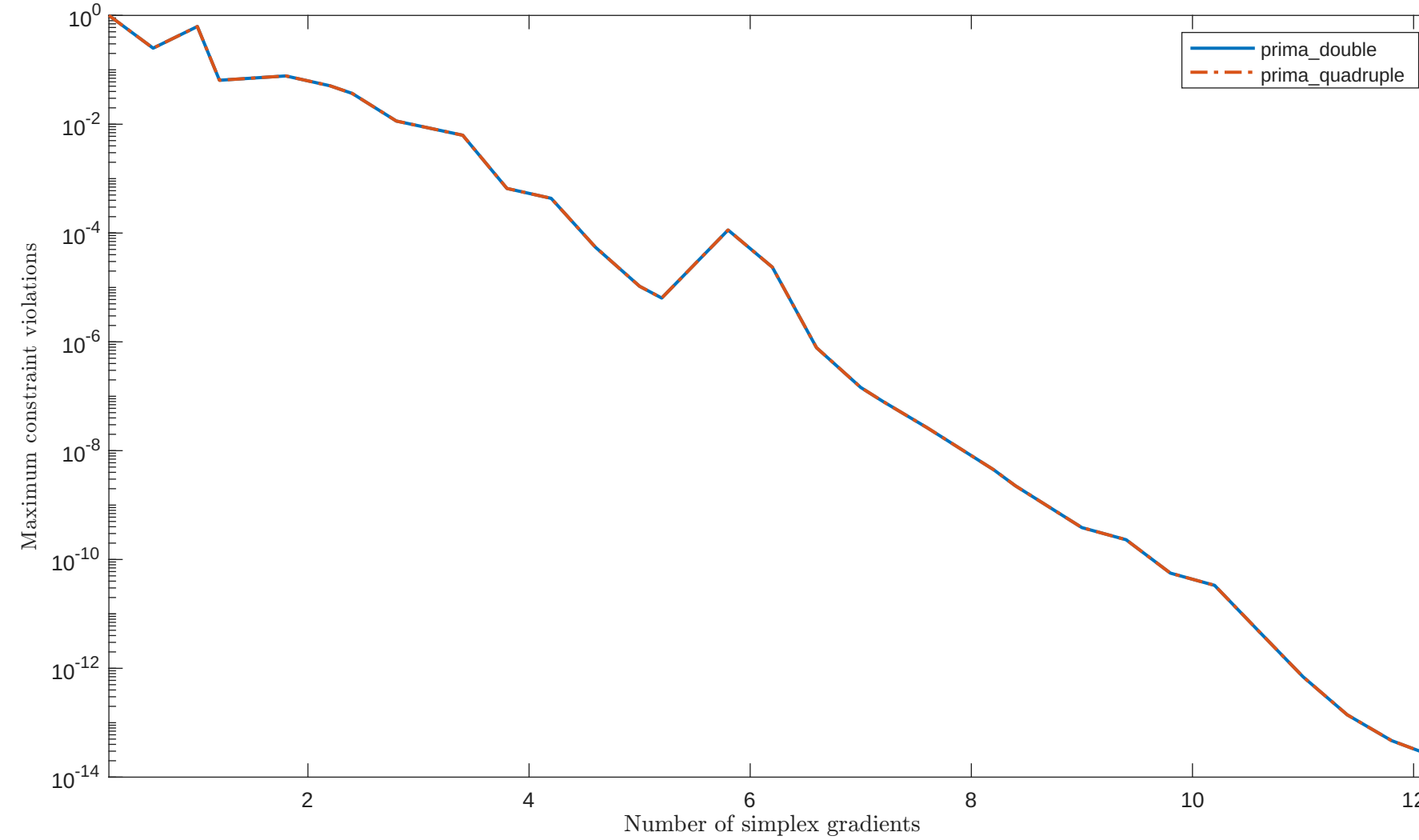
Solving "ALLINITA" with "plain" feature
