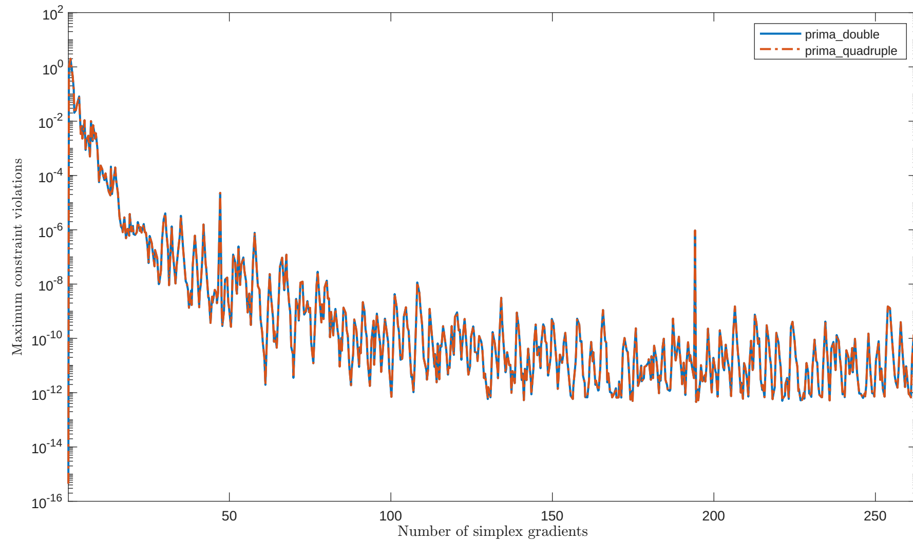
Solving "HS47" with "plain" feature
