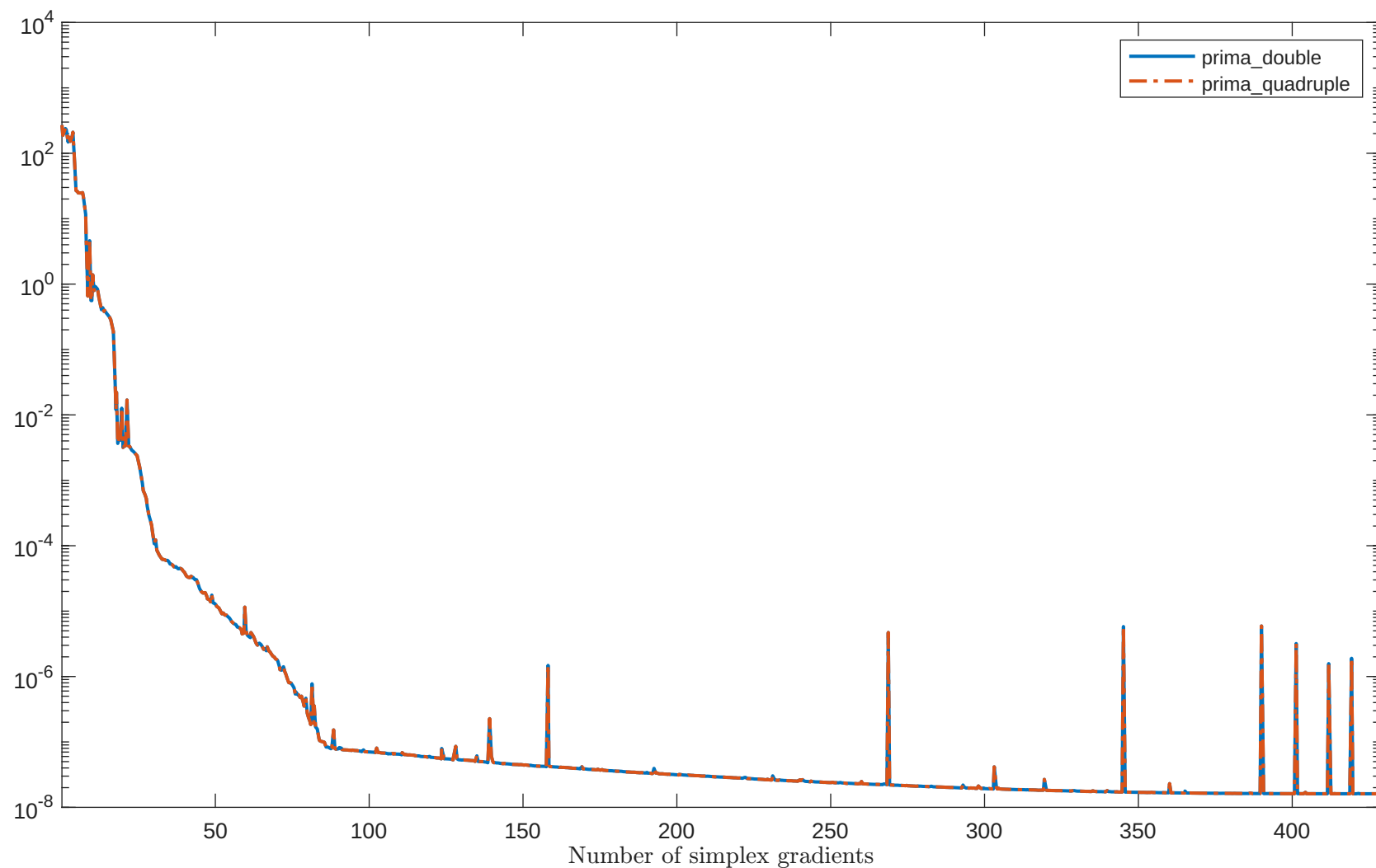
Solving “LANCZOS3LS” with “plain” feature
