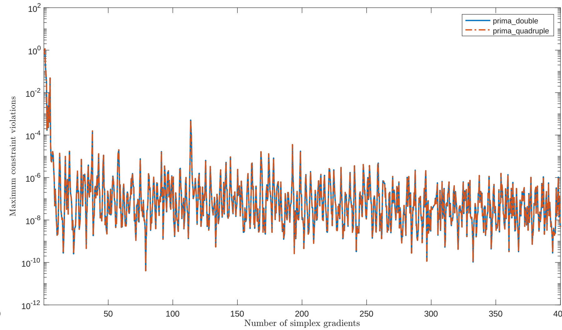
Solving “HS69” with “plain” feature
