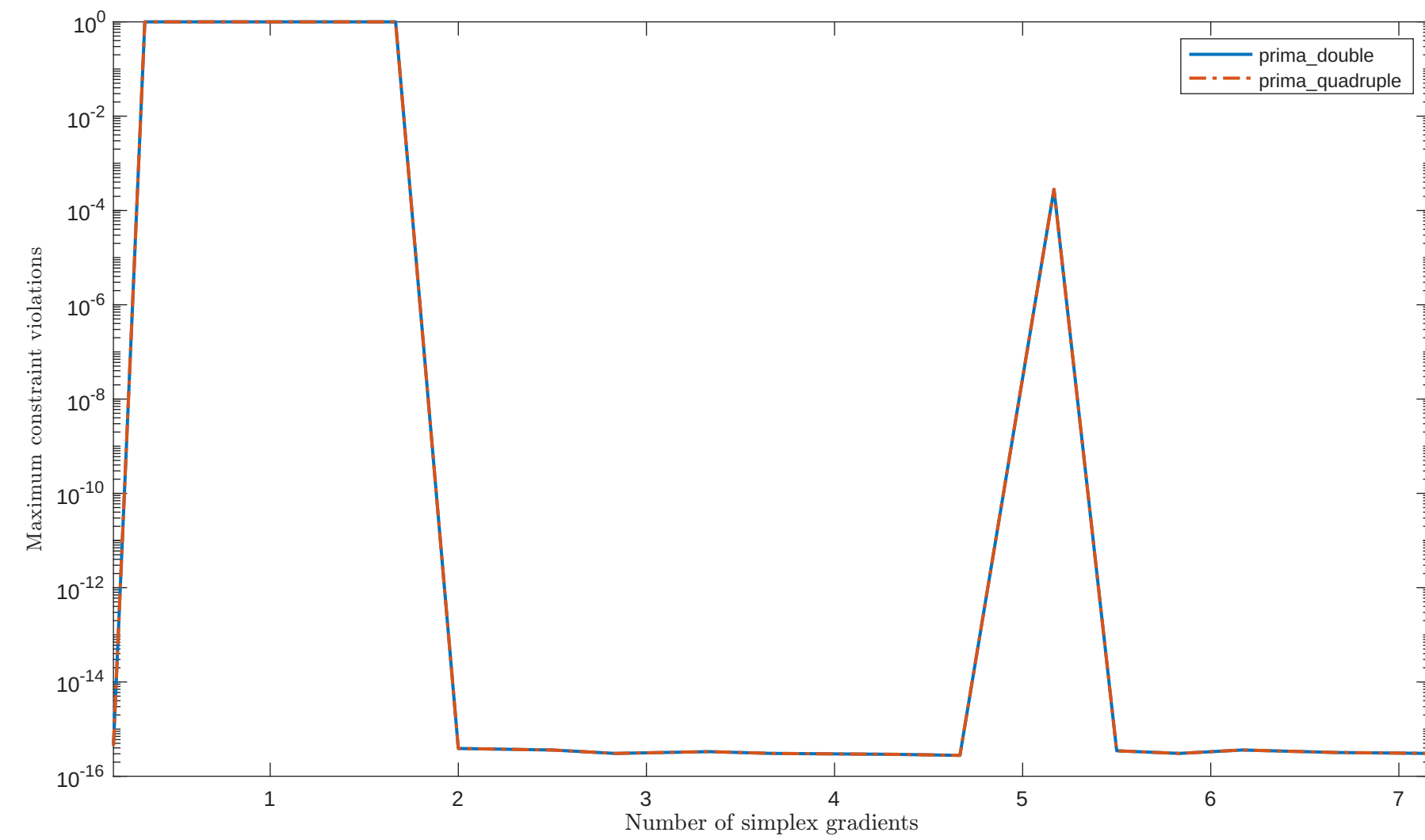
Solving "HS52" with "plain" feature
