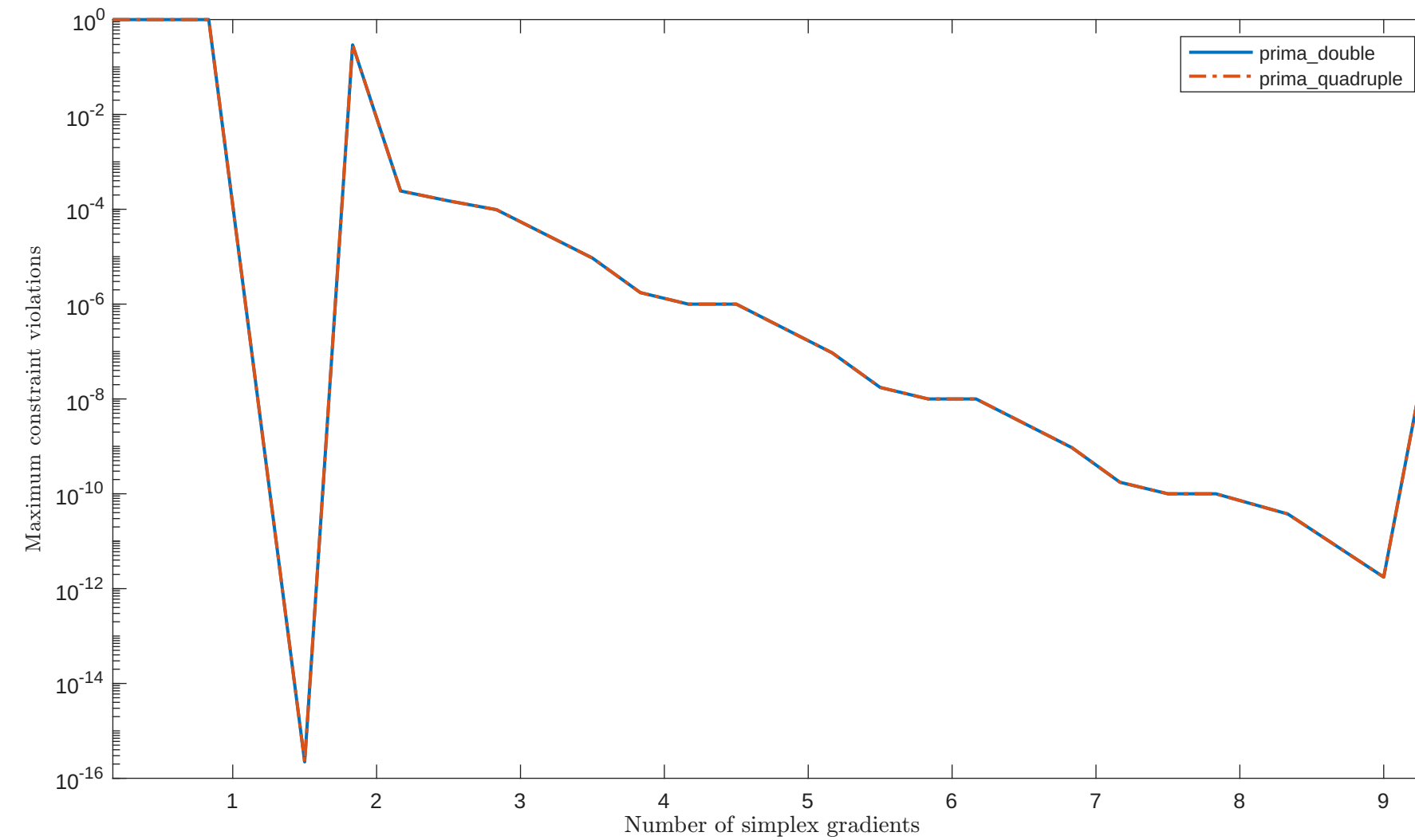
Solving "MINPERM" with "plain" feature
