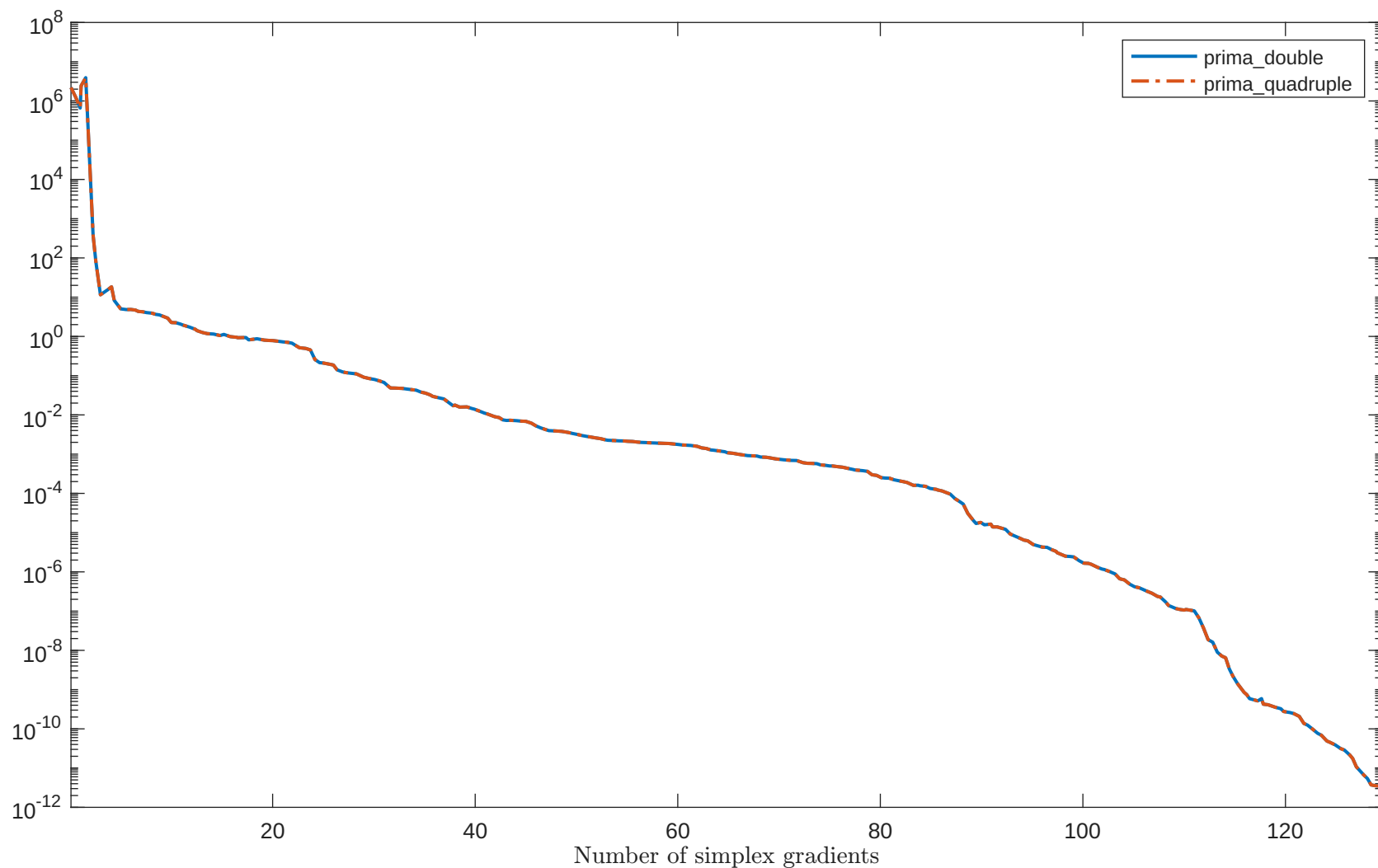
Solving "VARDIM" with "plain" feature
