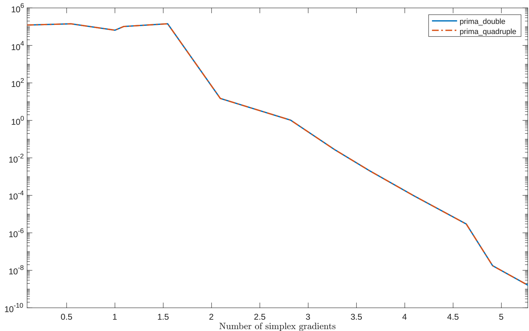
Solving “MANCINO” with “plain” feature
