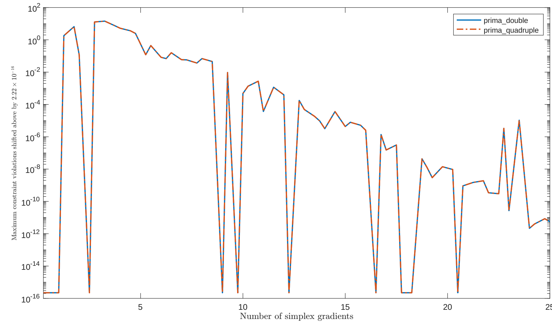
Solving "HS29" with "plain" feature
