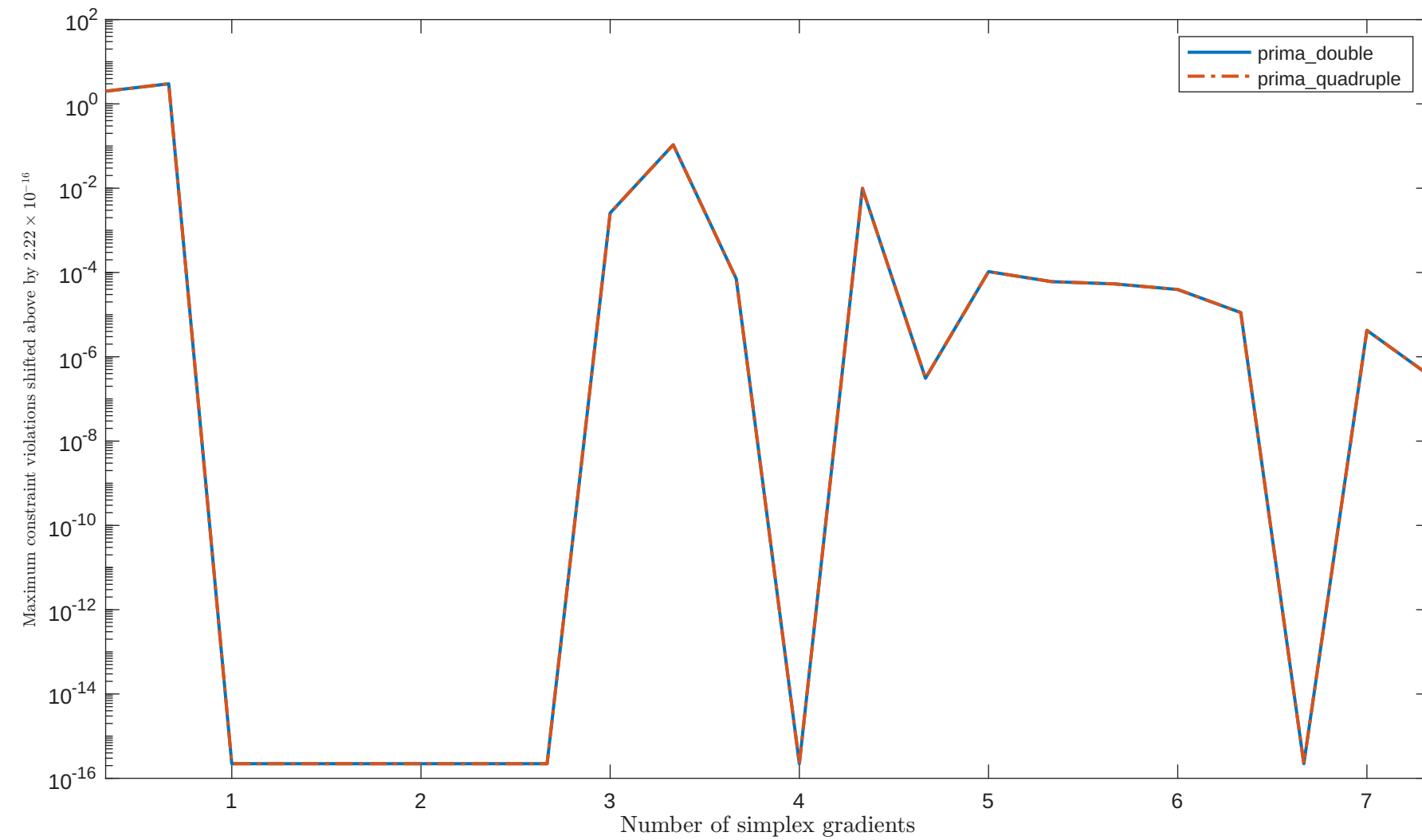
Solving "HS23" with "plain" feature
