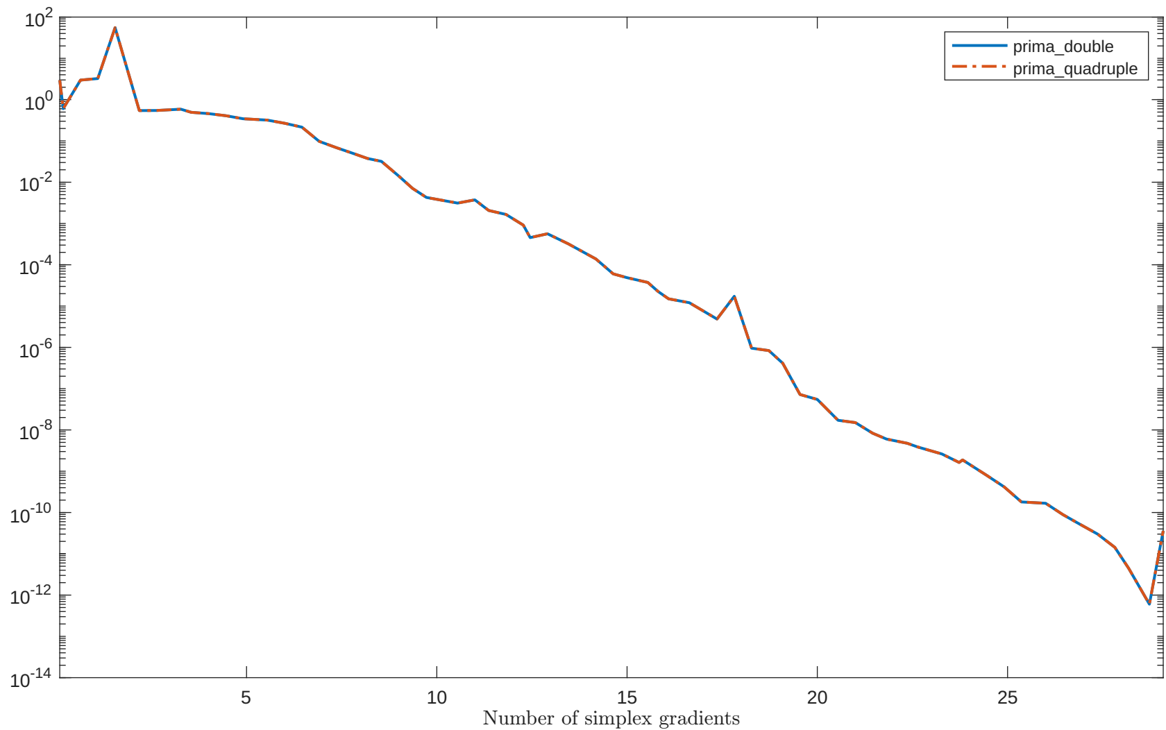
Solving "TRIGON1" with "plain" feature
