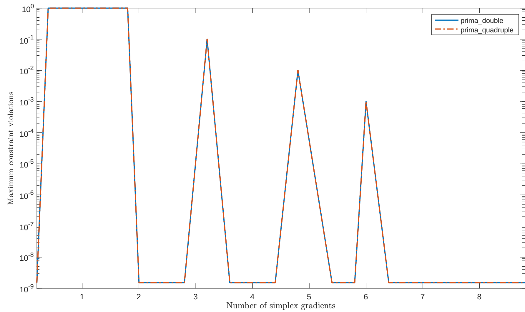
Solving "HS41" with "plain" feature
