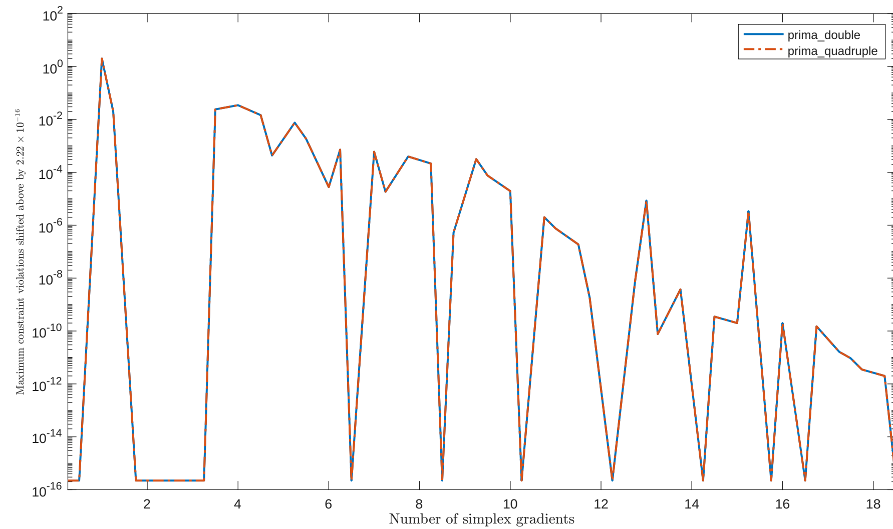
Solving "JANNSON4" with "plain" feature
