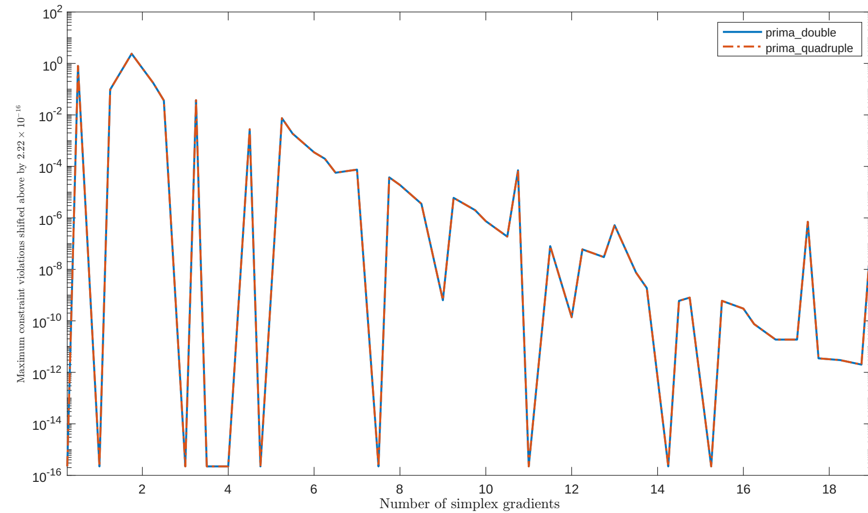
Solving "MIFFLIN1" with "plain" feature
