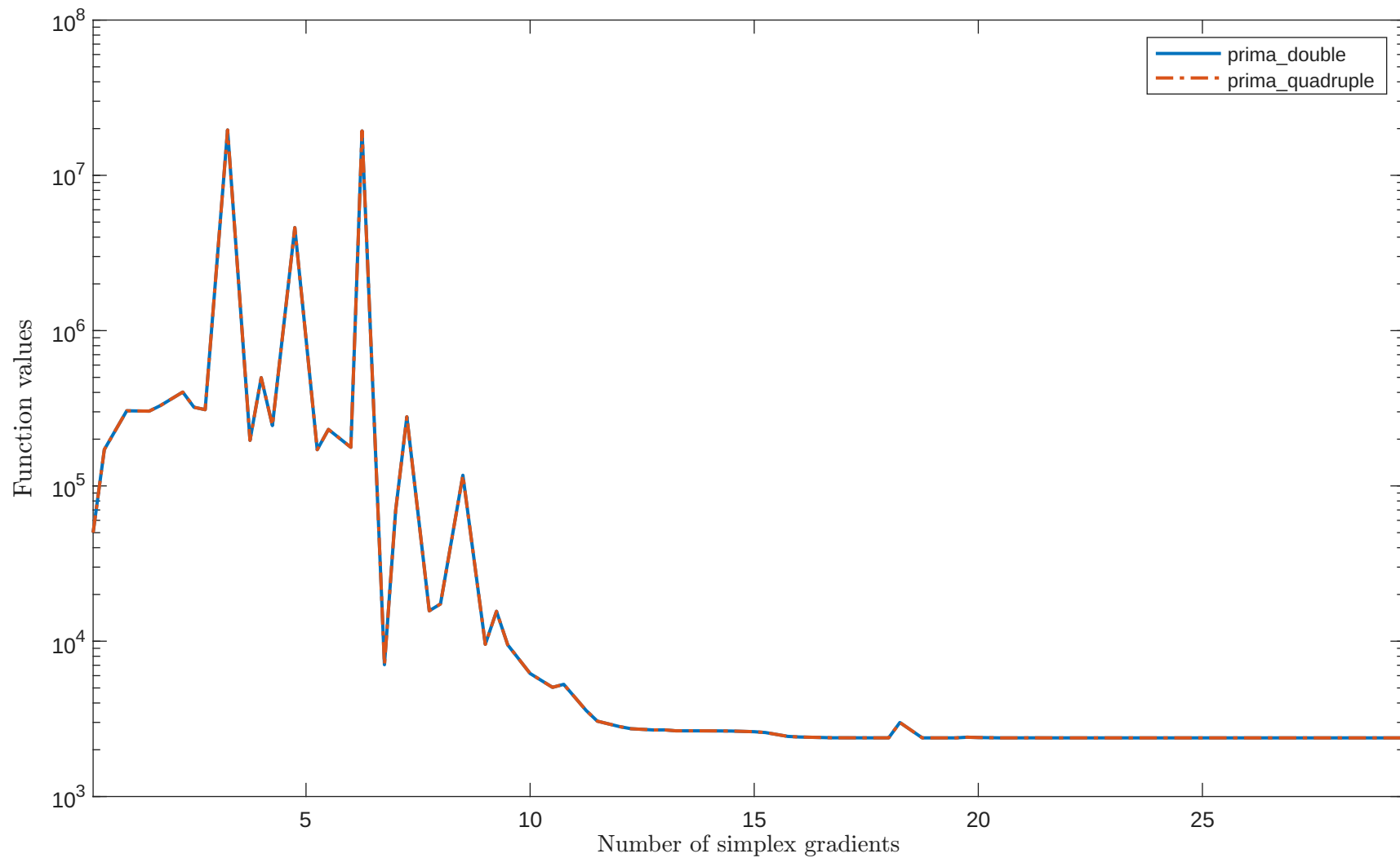
Solving “CHWIRUT1LS” with “plain” feature
