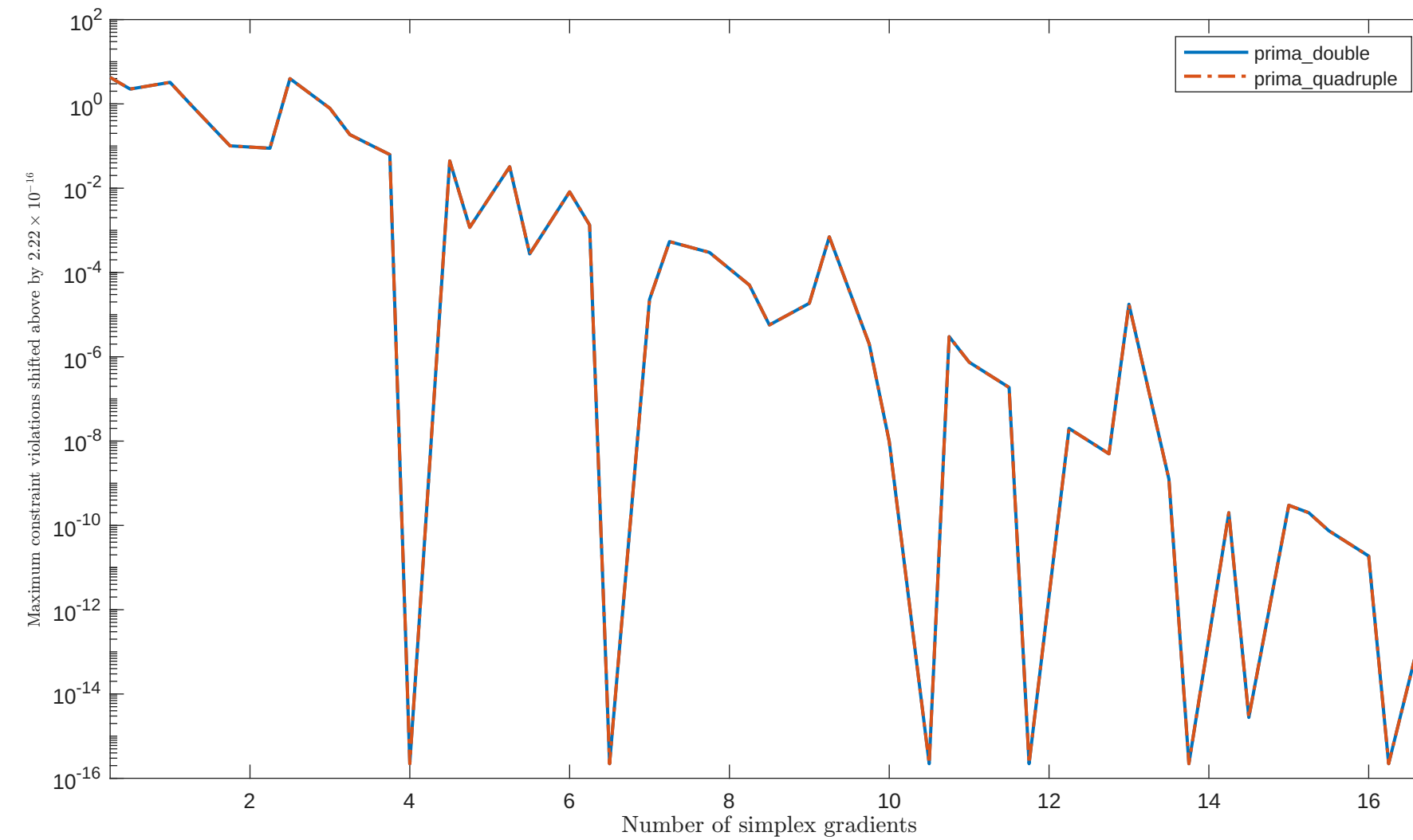
Solving "KIWCRES" with "plain" feature
