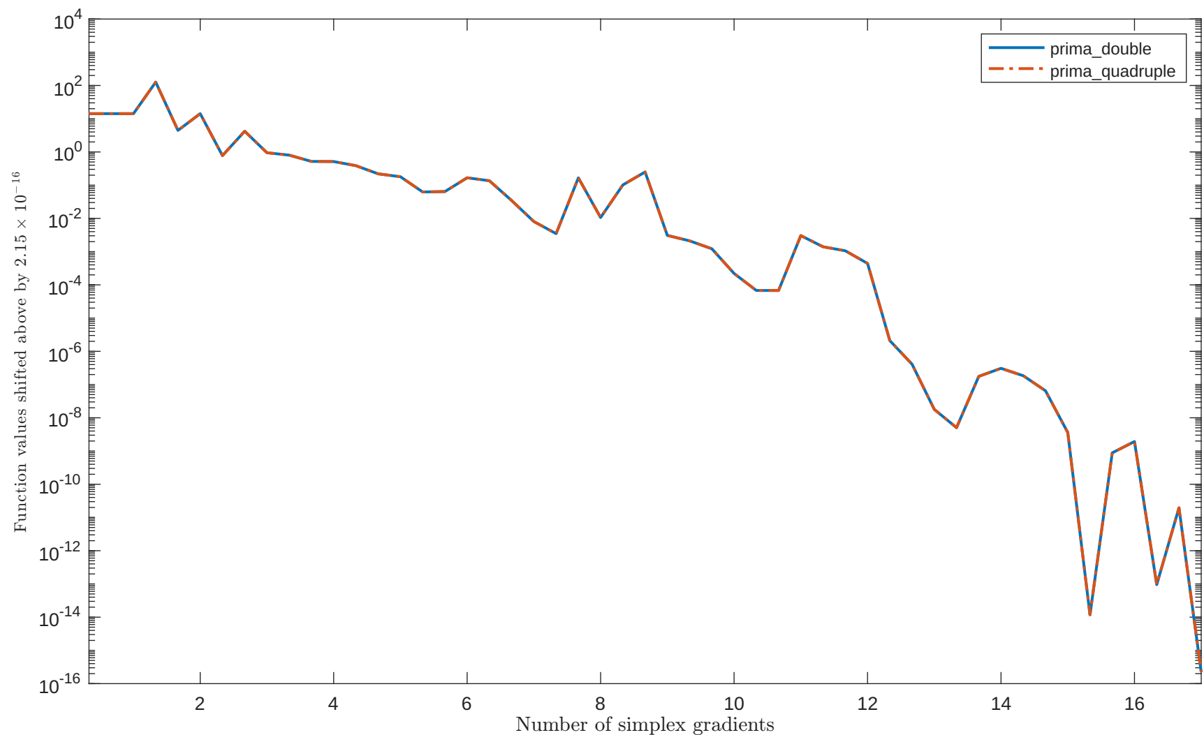
Solving “BEALE” with “plain” feature
