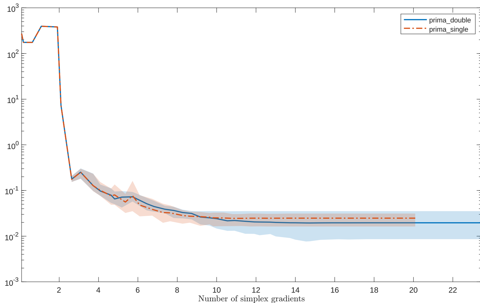
Solving “BROWNAL” with “noisy_0.001_mixed_gaussian” feature
